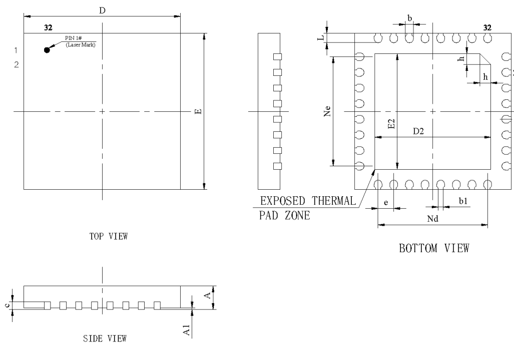
图 4-8 LKS32MC039PL5K6Q8B(C)封装图示
