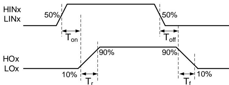
Figure 20-4 Switching sequence
