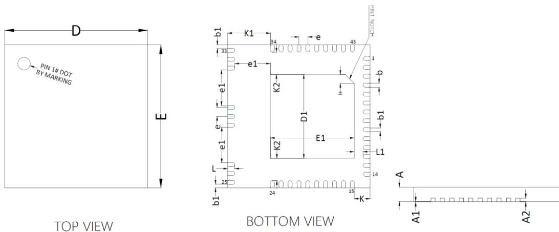
Figure 4- 3 LKS32MC038KU6Q8B(C) Packaging
