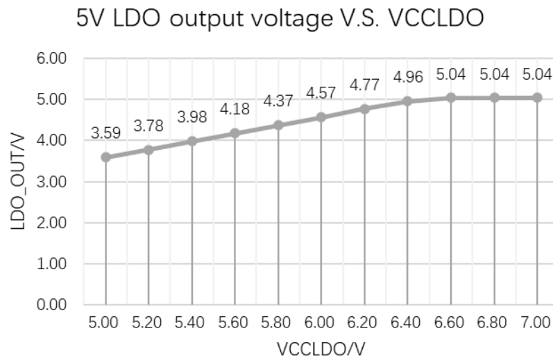
Figure 6-1 5V LDO Output Transfer Curve
