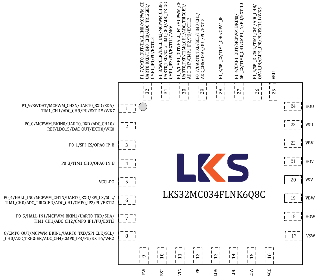
图 3-19 LKS32MC034FLNK6Q8C Pin Assignment Diagram
