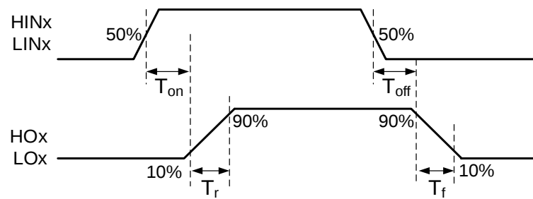
Figure 21-8 Switching Timing
