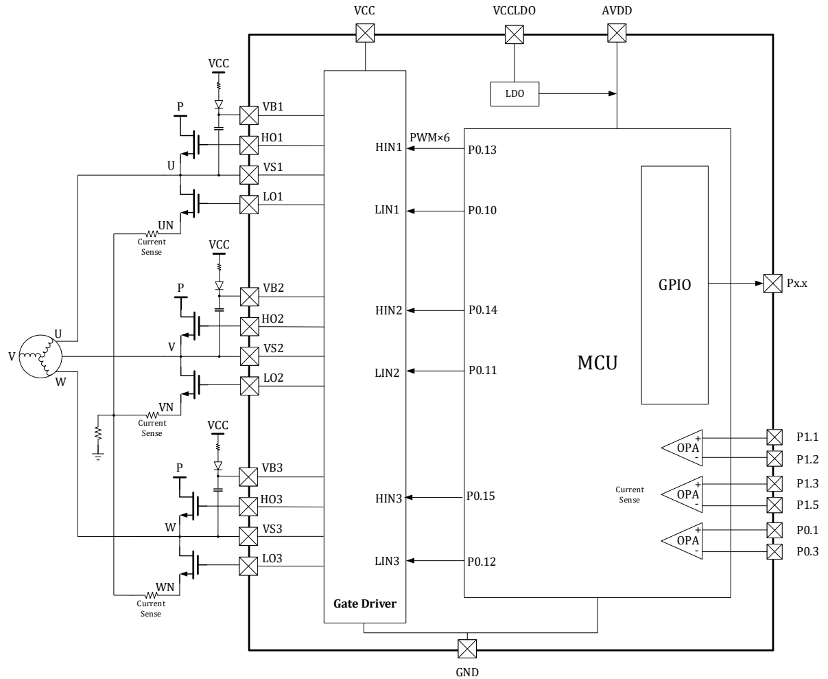
Figure 3-8 Schematic diagram of the LKS32MC034DOF6Q8 gate driver connection
