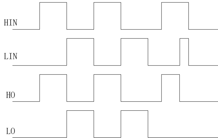
Figure 21-6 Schematic Diagram of LKS32MC034D(O)F6Q8 Gate Drive Polarity
