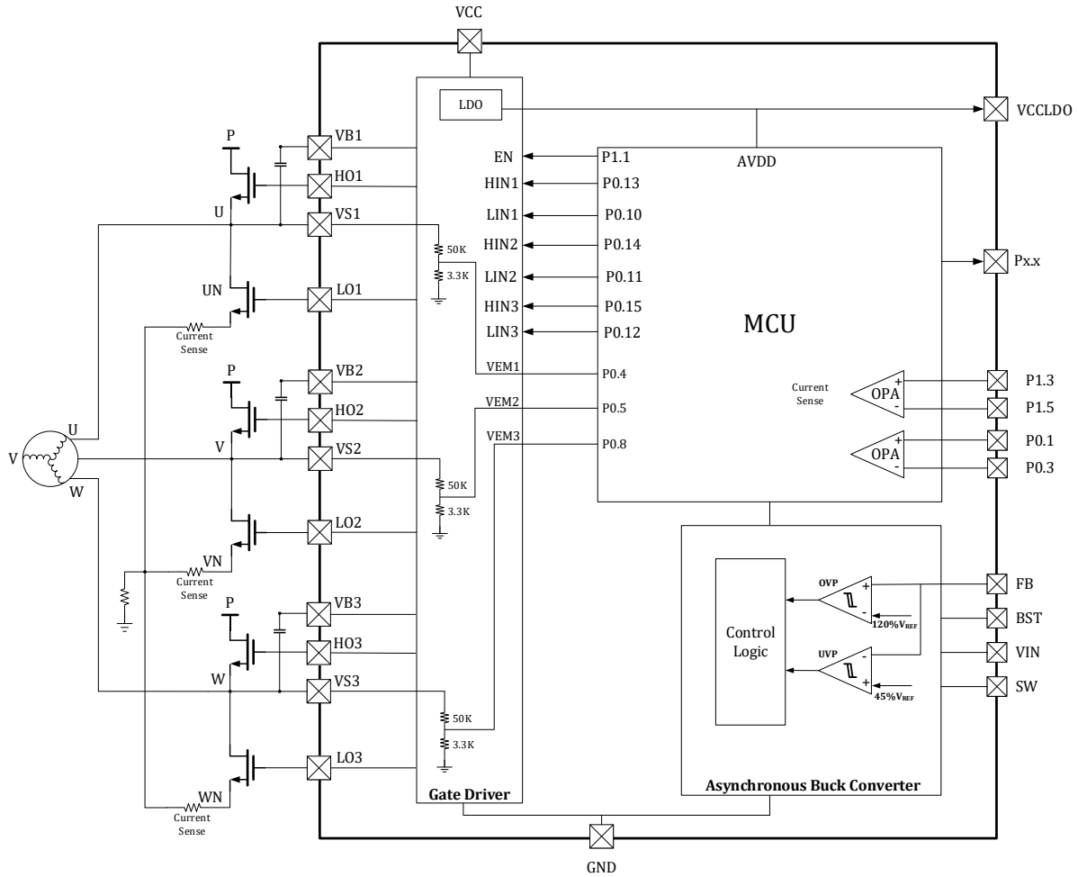
图 3-20 LKS32MC034FLNK6Q8C gate driver connection
