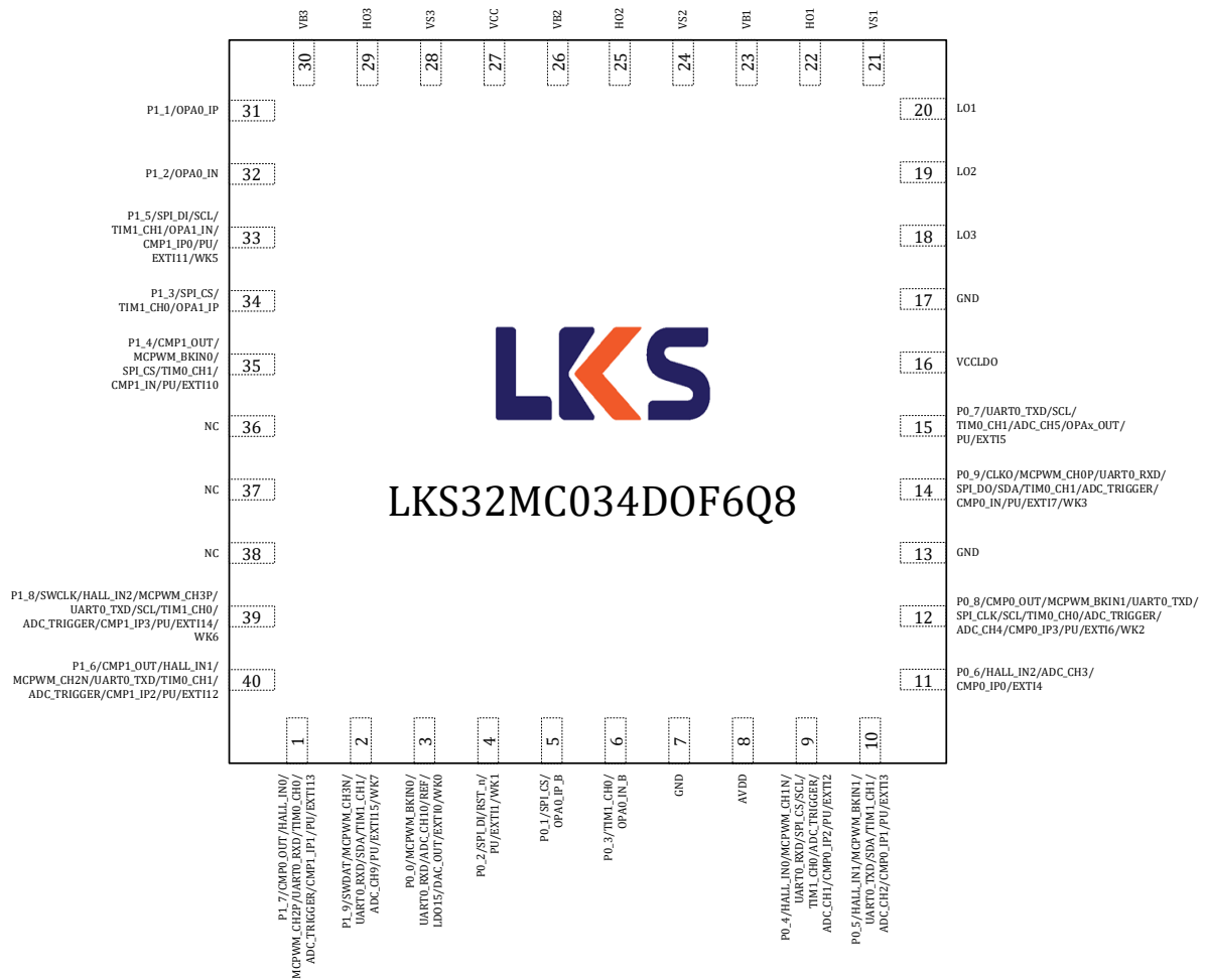
Figure 3-7 LKS32MC034DOF6Q8 Pin Assignment Diagram
