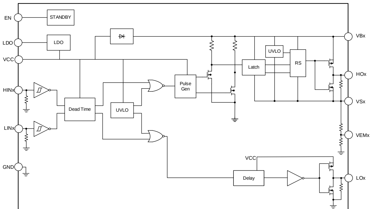
Figure 21-1 Internal block diagram of gate drive module G6
