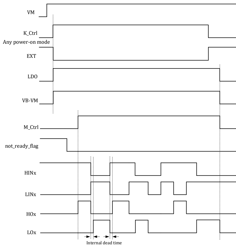
Figure 21-7 Schematic Diagram of Polarity for 6N-Type Gate Driver
