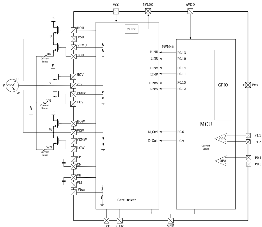
Figure 3-16 Schematic diagram of the LKS32MC034F2LF6Q8C gate driver connection
