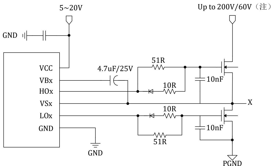
Figure 21-5 Typical Application Diagram of 6N Type Gate Drive Module LKS034FL
