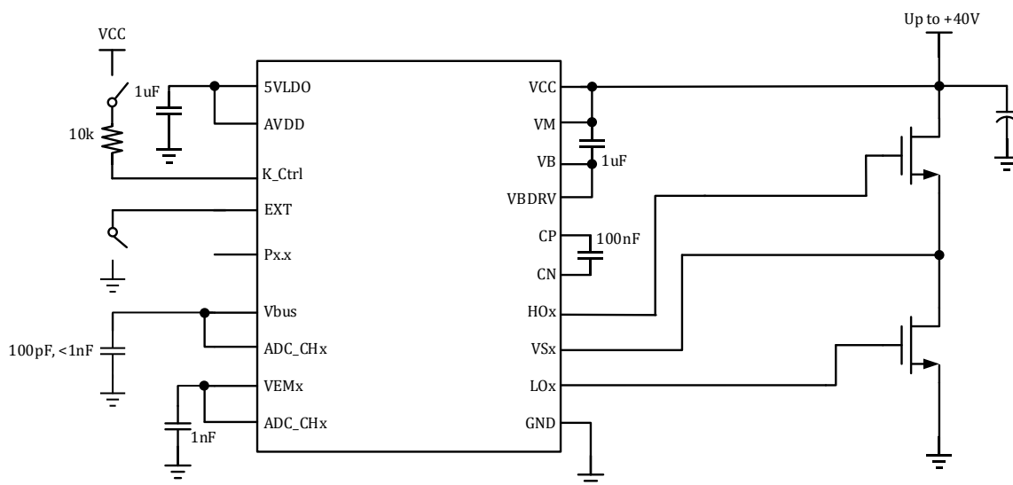
Figure 21-5 Typical Application Diagram of Gate Driver Module
