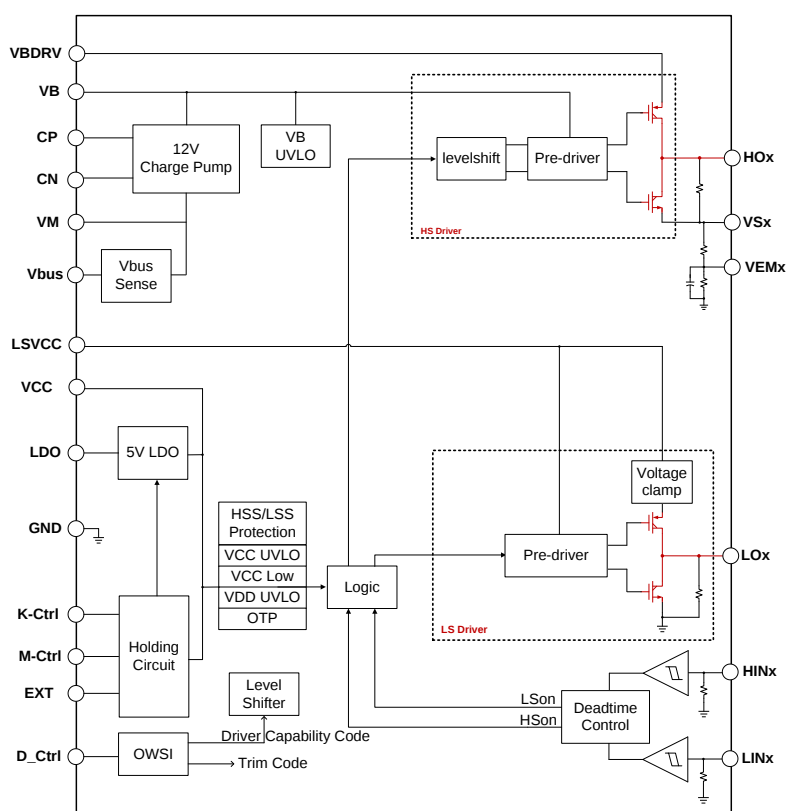
Figure 21-6 Typical Application Diagram of Gate Driver Module
