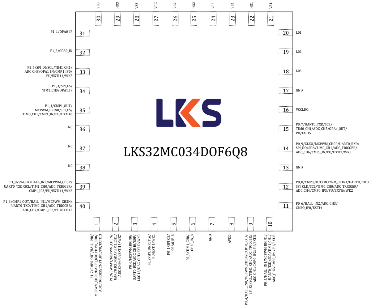
Figure 3-9 LKS32MC034DOF6Q8B(C)/LKS32MC034SF6Q8B(C) Pin Assignment Diagram
