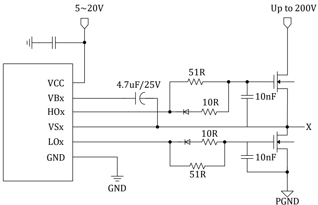
Figure 21-7 Typical Application Diagram of 6N Type Gate Drive Module LKS034S
