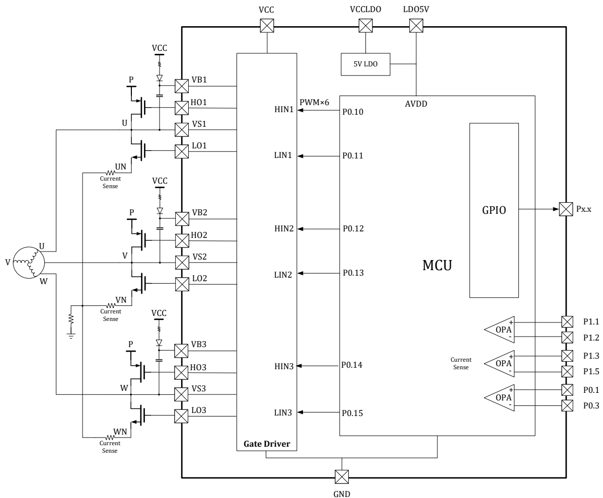
Figure 3-22 Schematic diagram of the LKS32MC038KU6Q8B(C) gate driver connection
