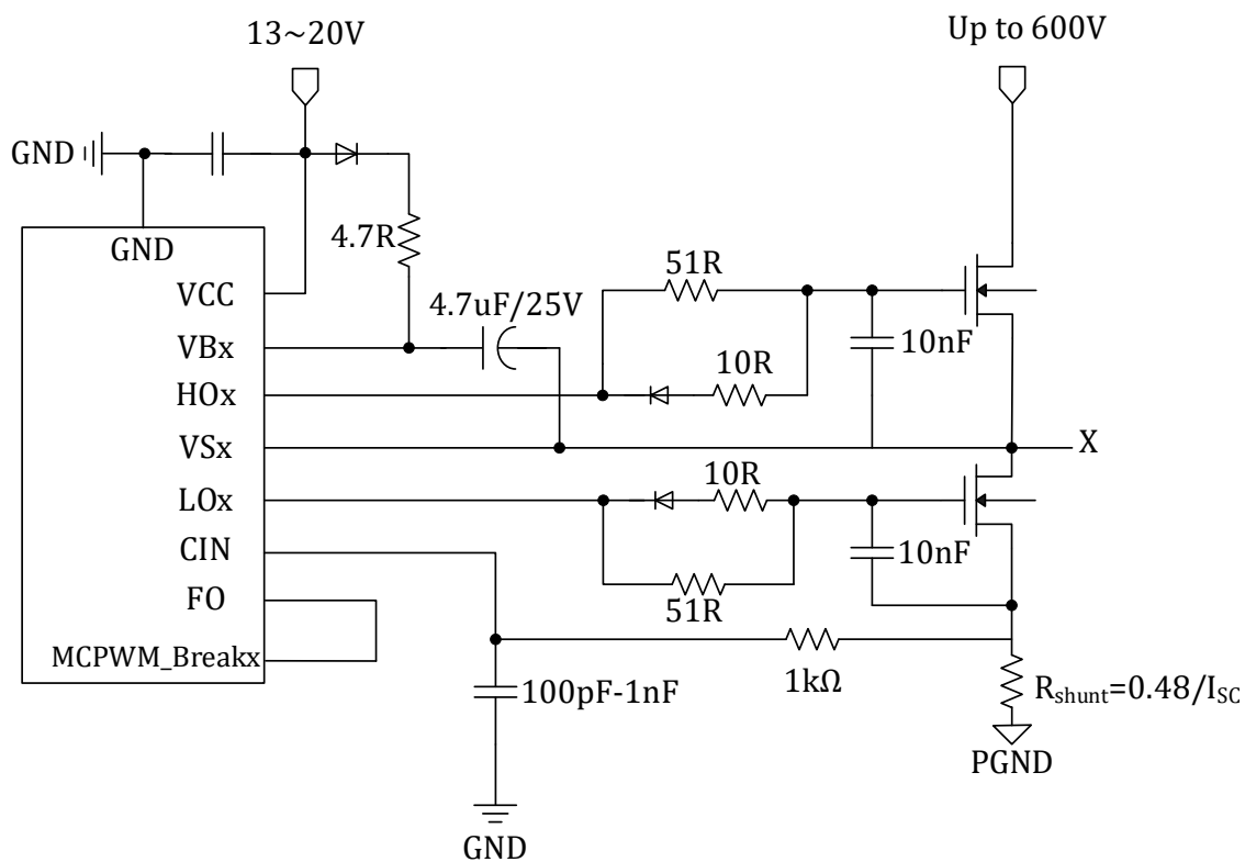
Figure 21-2 Typical Application Diagram of 6N Type Gate Drive Module LKS32MC031KLC6T8B
