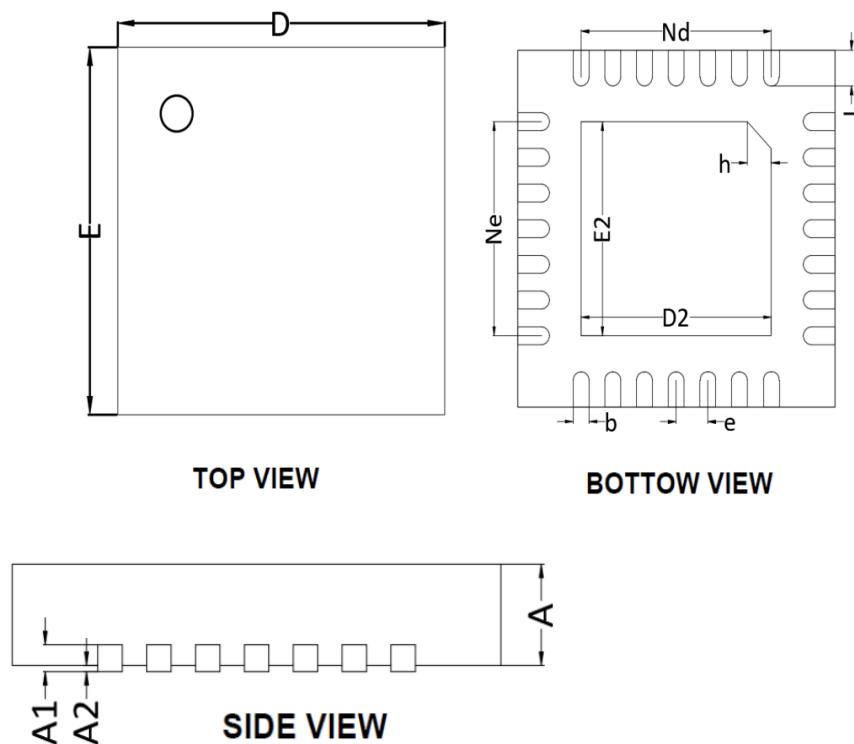
Figure 4-5 LKS32MC038LY6Q8(B/C) Packaging
