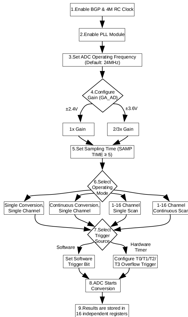
Figure 11-1ADC Configuration Flowchart
