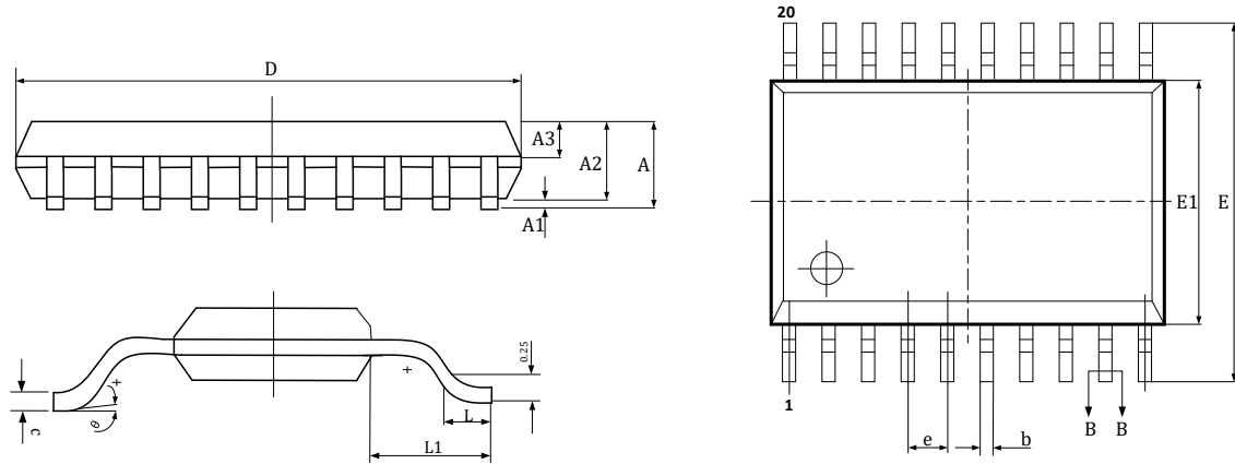
Figure 4-1 LKS32MC033H6P8(B/C) Packaging
