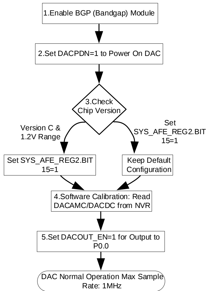
Figure 15-1DAC Configuration Flowchart
