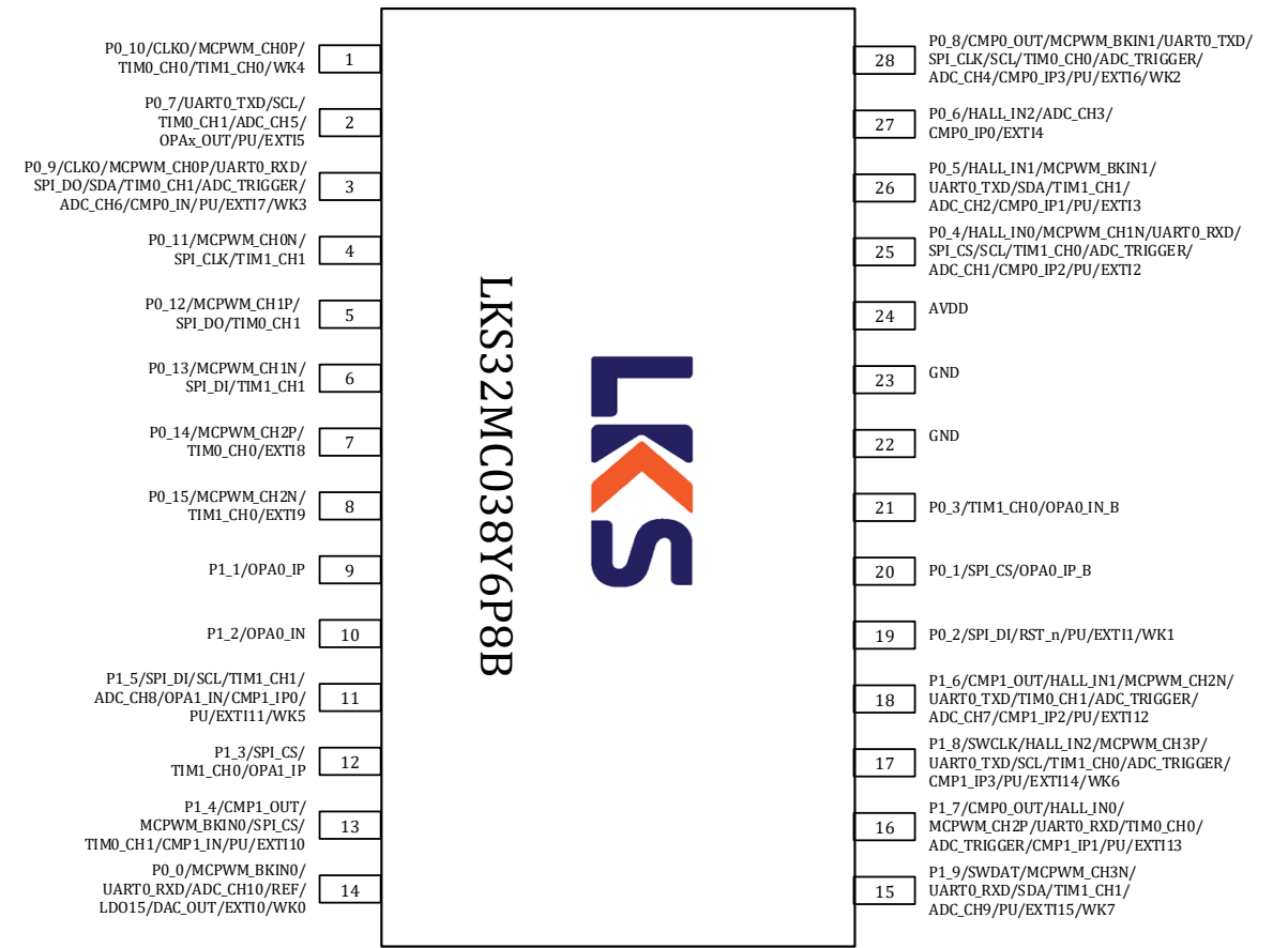
图 3-10 LKS32MC038Y6P8B/LKS32MC038Y6P8C 管脚分布图
