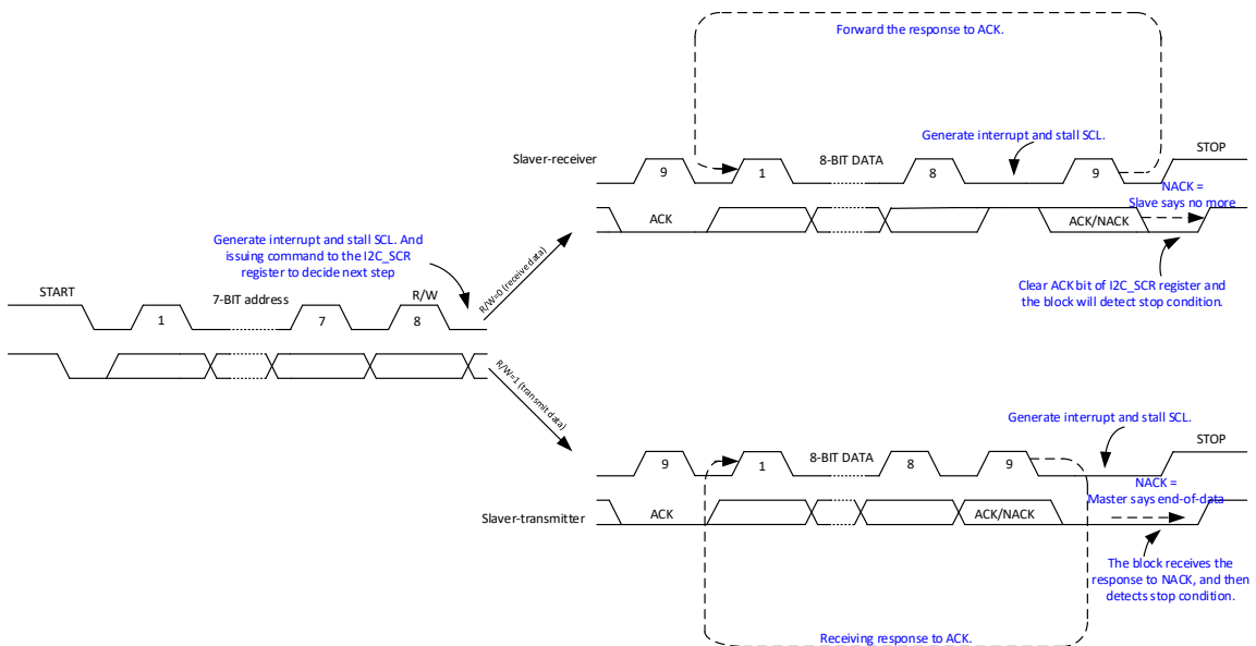
Fig. 9-5 Schematic Diagram of Transmission in Slave Mode
