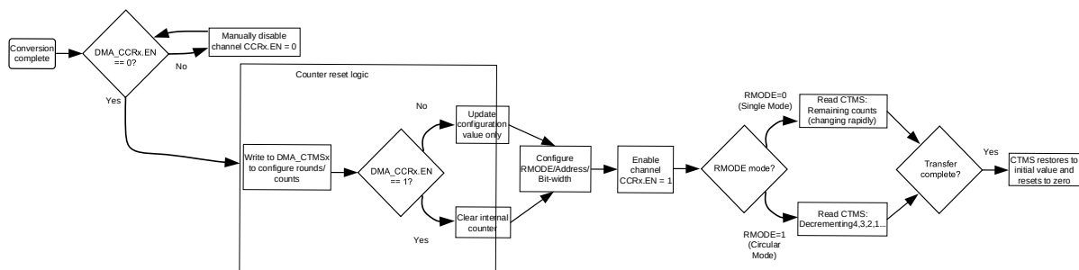
Fig. 17-7 DMA Operation Logic Flowchart
