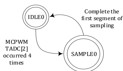
Fig. 12-6 State Transition Diagram of ADC Single-round Sampling
