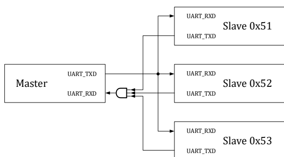
Fig. 16-5 Example of UART Multi-computer Communication
