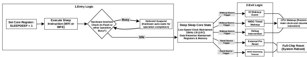
Figure 20-1 WWDG Counting & Refresh Mechanism and Deep Sleep Entry/Exit Flow
