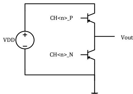
Fig. 14-12 MCPWM IO Control Diagram
