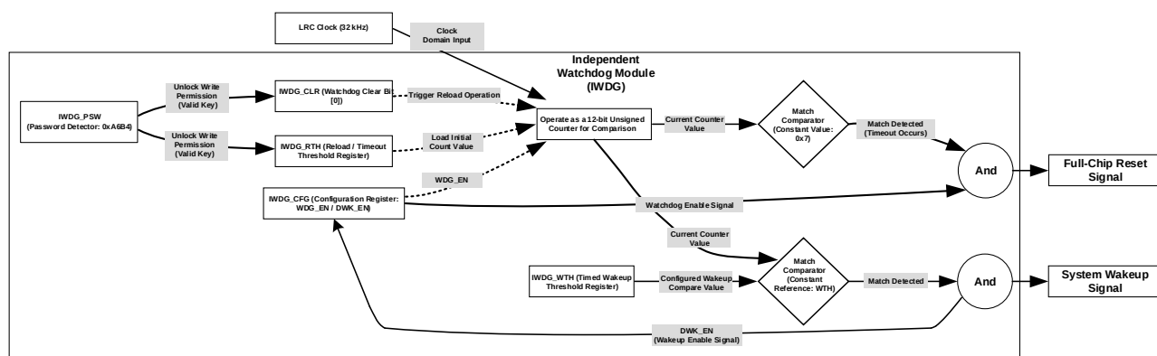
Figure 19-1 IWDG Operating Principle & Signal Flow
