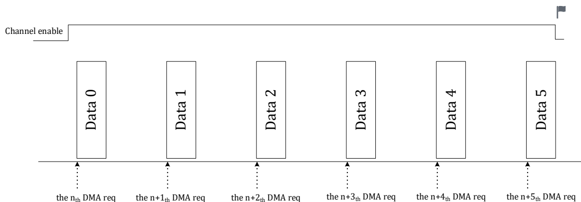
Fig. 17-3 RMODE=1 DMA transmission
