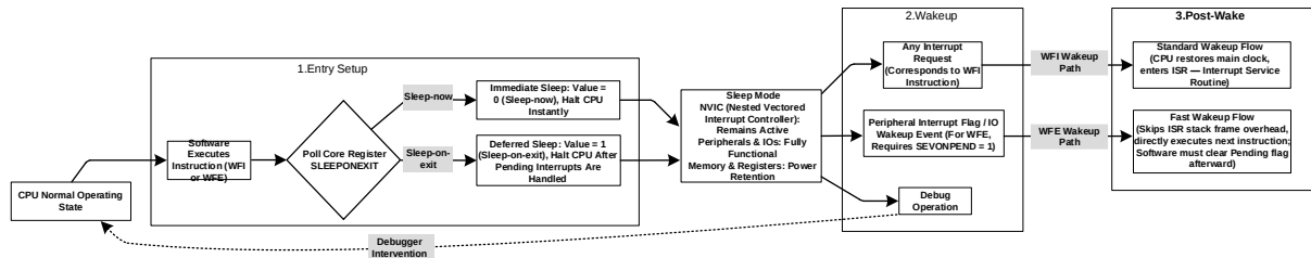
Figure 20-2 Flowchart of Conventional Sleep Mode Entry and Wakeup
