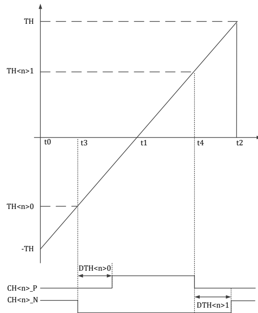
Fig. 14-8 MCPWM Timing TH &lt;n&gt; 0 and TH &lt;n&gt; 1 - Complementary Mode
