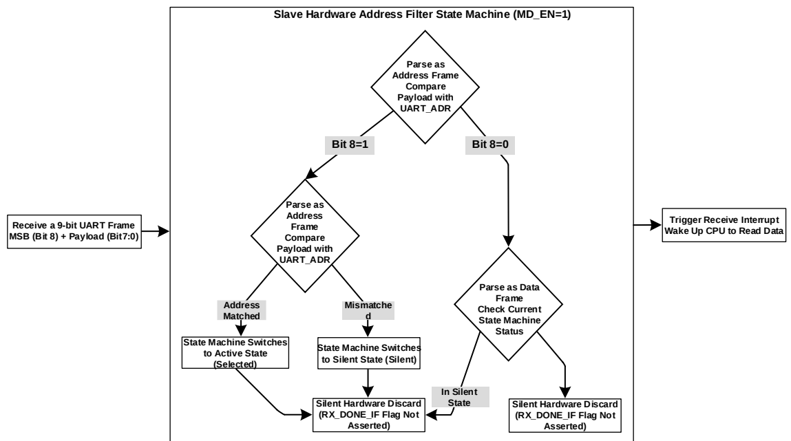
Fig. 16-4 Processing Flow of Slave 9-bit UART Address Frame Filter State Machine
