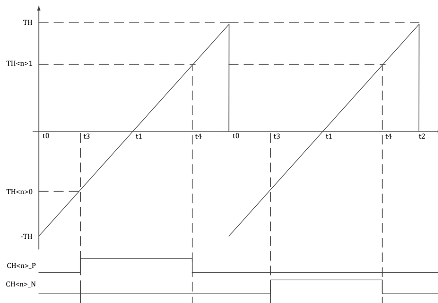
Fig. 14-9 MCPWM Timing TH&lt;n&gt;0 and TH&lt;n&gt;1 - Center-aligned Push-pull Mode
