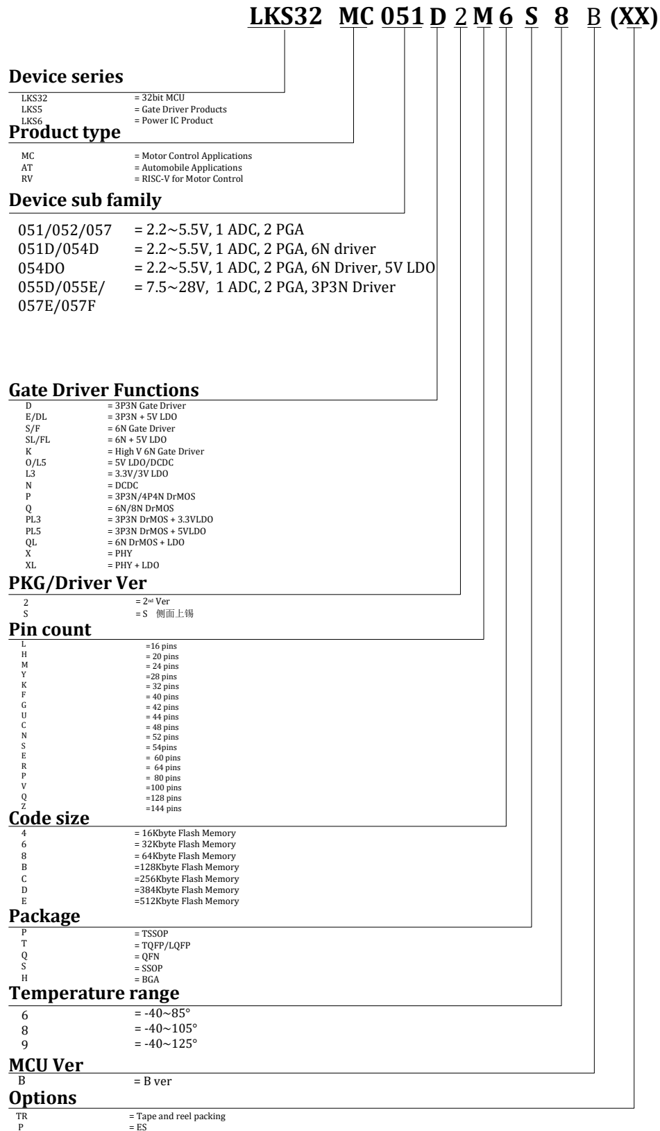
Fig. 1-1 Naming Conventions of LKS32MC057EM6S8 Components
