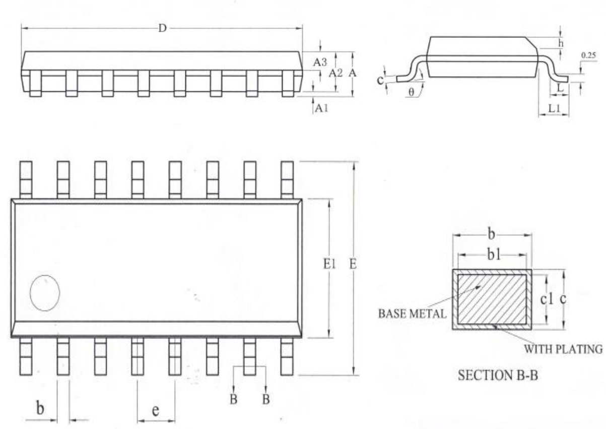
Fig. 4-2 LKS32MC055DL6S8 Package Diagram
