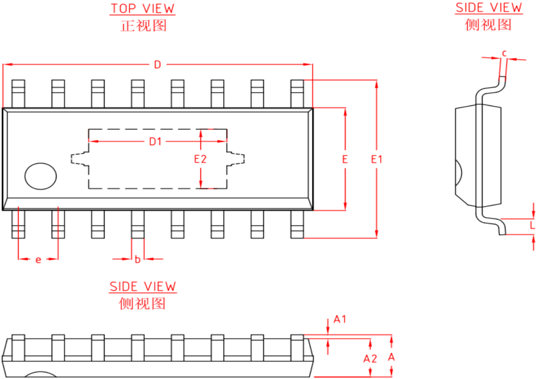
Fig. 4-3 LKS32MC055EL6S8 Package Diagram
