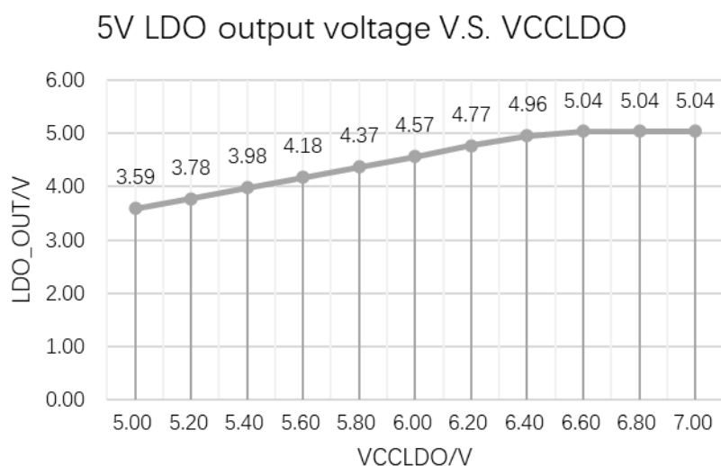
Figure 7-1 5V LDO output V.S. VCCLDO
