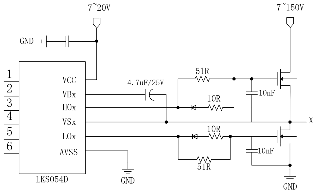
Fig. 21-2 Gate Driver Module G3 typical schematic
