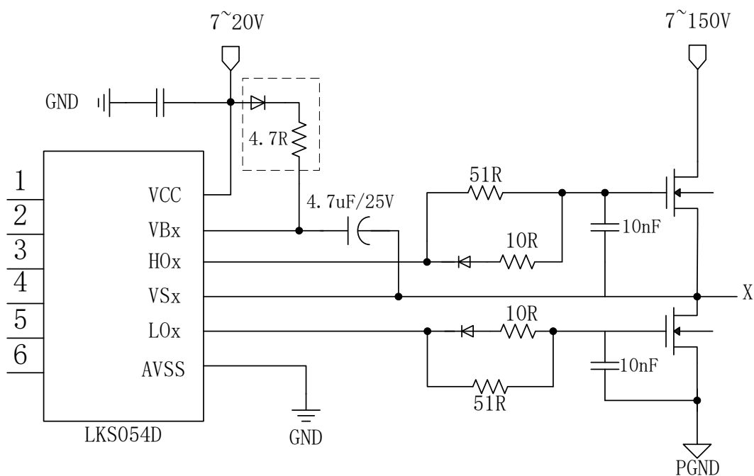
Fig. 21-1 Gate Driver Module G1/G2 Typical Application Diagram
