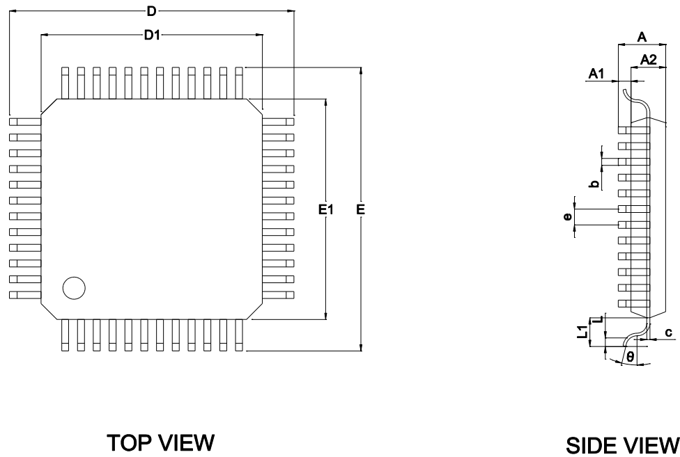
Fig. 4-1 LKS32MC051DC6T8 Package Diagram
