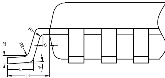
图 4-3 LKS32MC071CBT8/LKS32MC071C8T8 Package Diagram(LQFP48)
