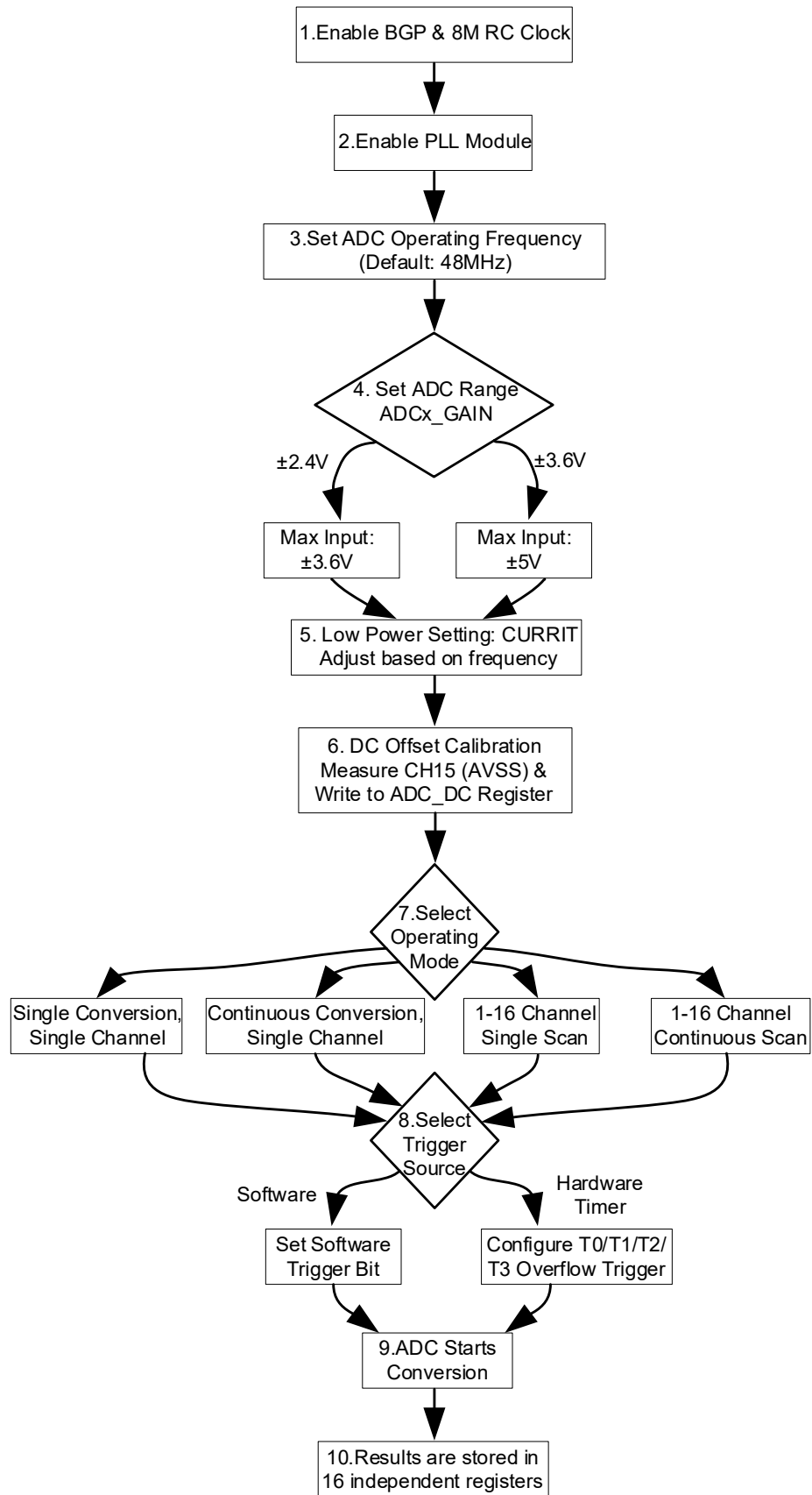
Figure 10-1ADC Configuration Flowchart
