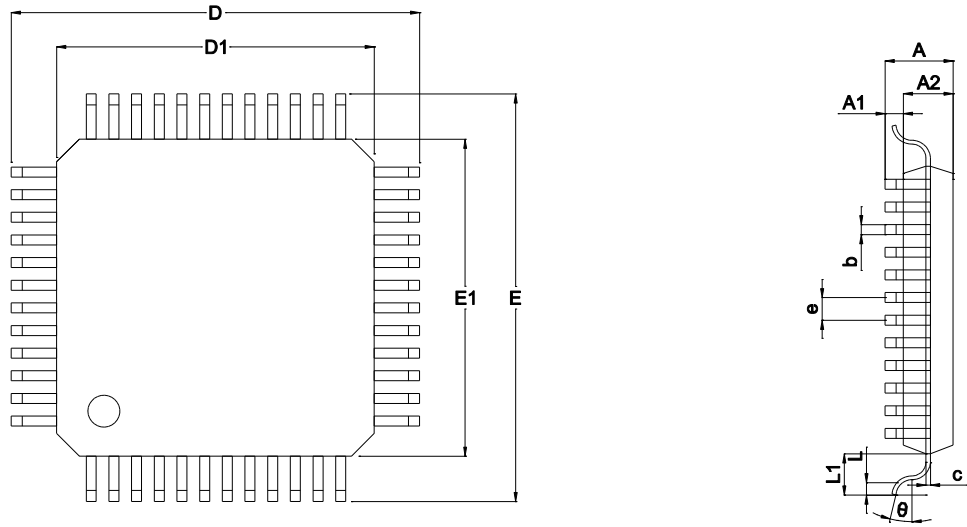
TOP VIEW SIDE VIEW Fig.4-2 LKS32MC071CBT8/LKS32MC071C8T8 Package Diagram(TQFP48)
