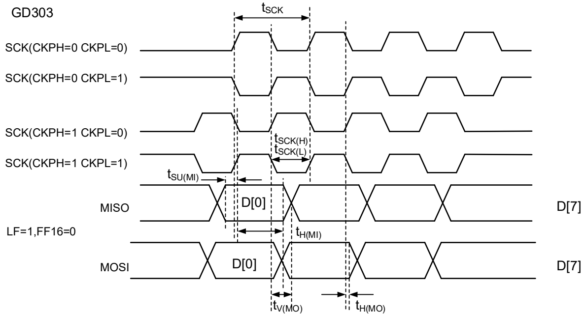
图 11-3 SPI Master Mode Timing Diagram
