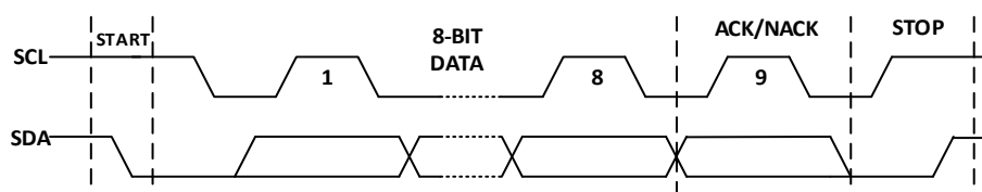
Fig. 9-2 Basic I2C Transfer Timing Diagram
