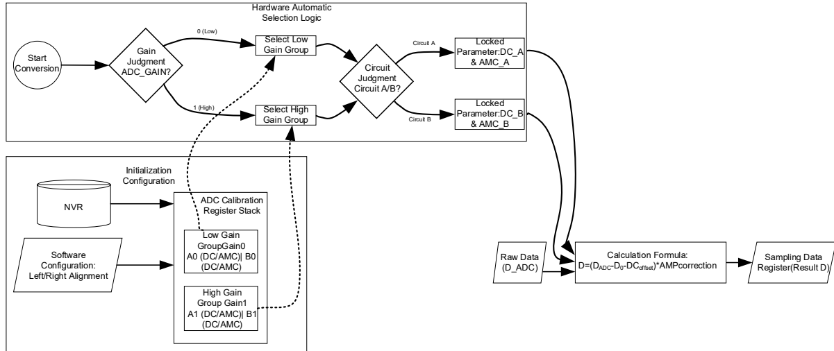
Figure 12-4 ADC Calibration Processing Flowchart
