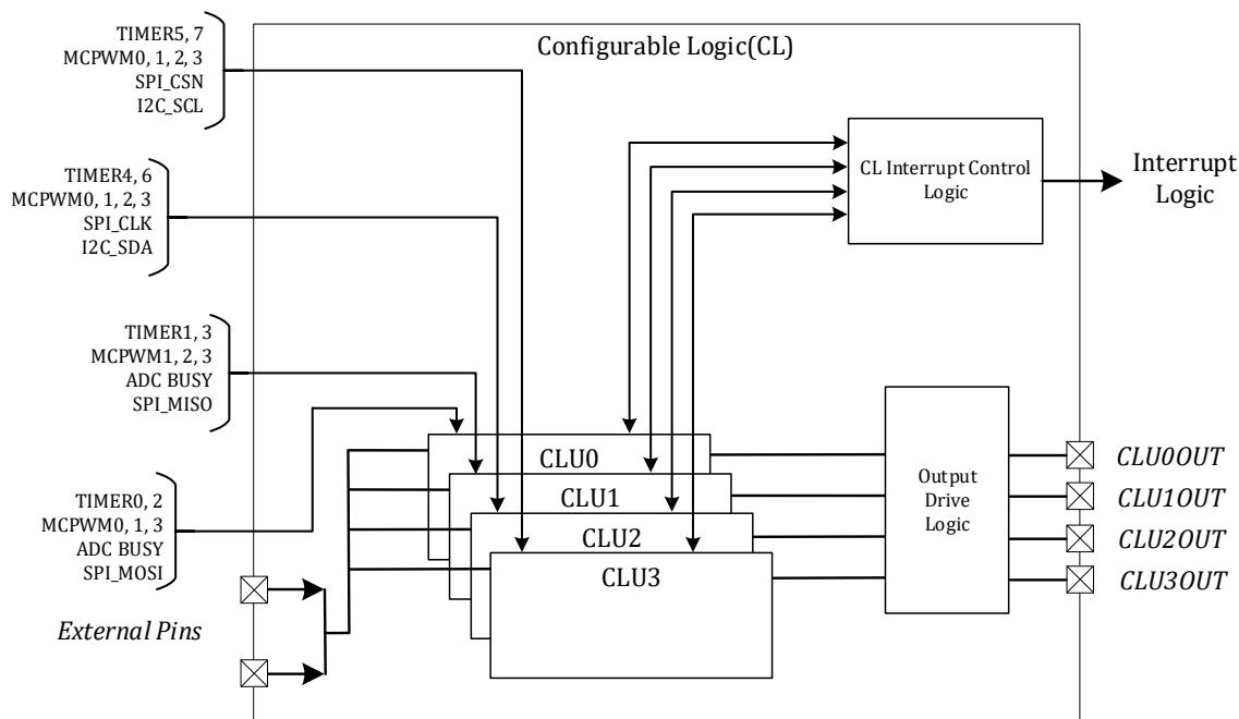
Figure 23-1 CL Module Top Level Functional Block Diagram
