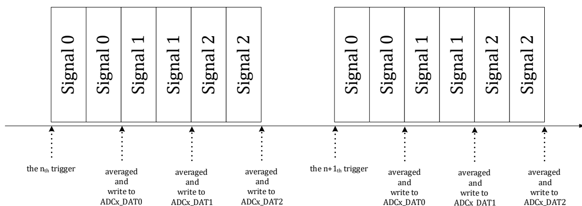
Figure 12-6 Oversampling Conversion Timing Example 1
