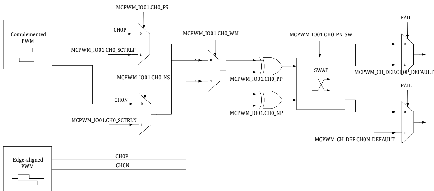
Figure 14-6 IO Driver Module Data Flow Diagram
