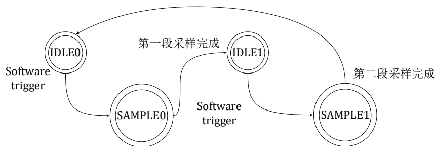
Figure 12-7 ADC Two-Segment Sampling State Transition Diagram
