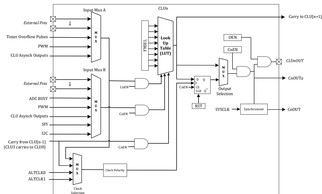
Figure 23-2 Functional block diagram of independent CLU module
