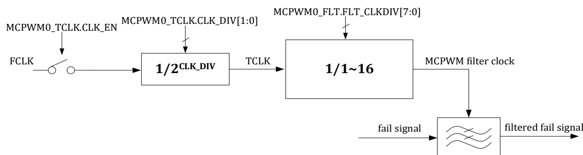
Figure 14-5 MCPWM Fail Signal Filter Clock Generation Logic
