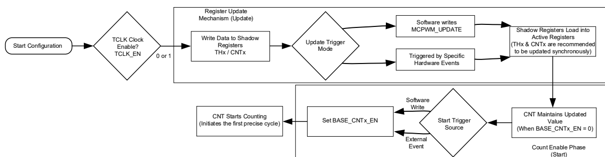
Fig. 14-1 Flow Chart of Time Base Register Update and Count Enable
