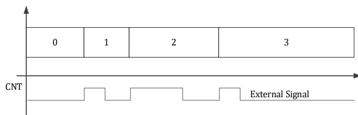
Figure 13-10 TIMER counts with an external clock
