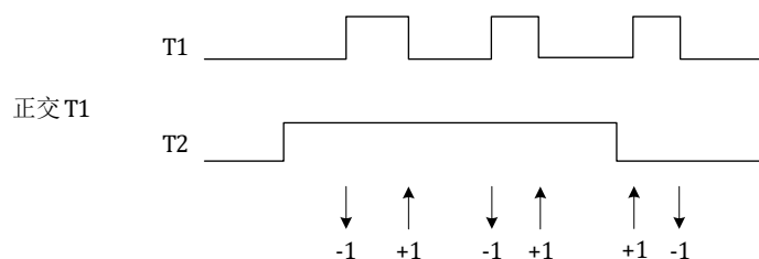
Figure 13-14 Quadrature Encoded Signal Count Case Counted by Encoder at Time T1 or T2
