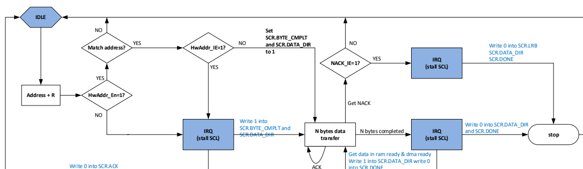
Fig. 9-7 Schematic diagram of multi-byte sending in slave mode
