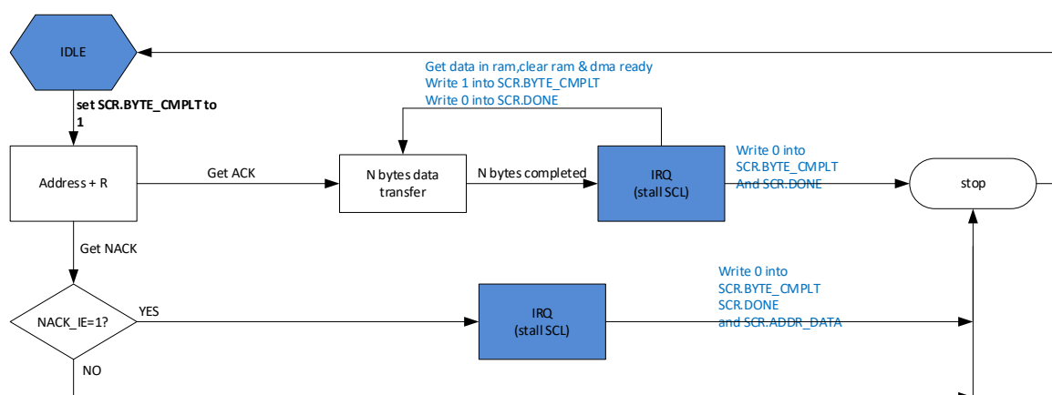
Fig. 9-12 Schematic diagram of multi-byte reception in master mode
