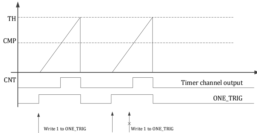
Figure 13-6 TIMER single trigger
