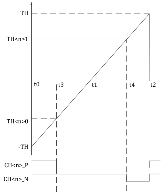
Figure14-9MCPWM Timing Edge Alignment Mode
