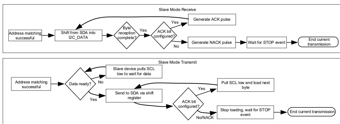
Fig. 9-6 I2C Slave Mode (Transmit/Receive/DMA) Logic Flowchart
