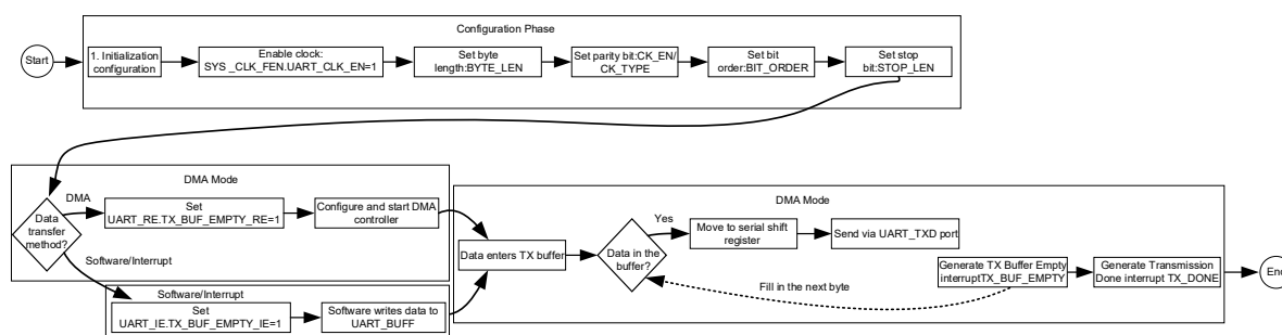
Figure17-1 UART Transmission Flow and Hardware Mechanisms
