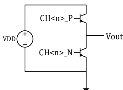
Figure14-11MCPWM IO Control Schematic
