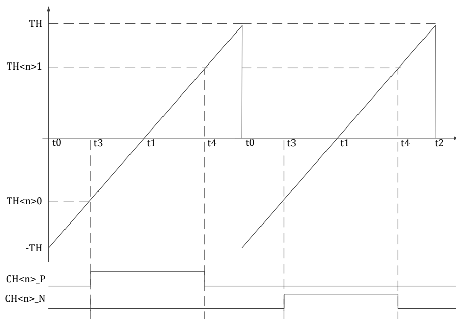
Figure14-8 MCPWM Timings TH &lt; n &gt; 0 and TH &lt; n &gt; 1-Center Aligned Push-Pull Mode
