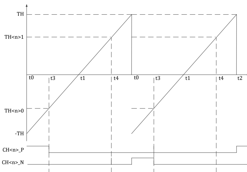
Figure14-10MCPWM Timing TH &lt; n &gt; 0 and TH &lt; n &gt; 1 Edge-Aligned Push-Pull Mode
