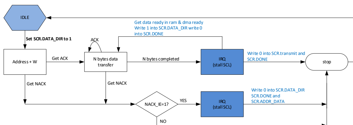
Fig. 9-11 Schematic diagram of multi-byte transmission in master mode
