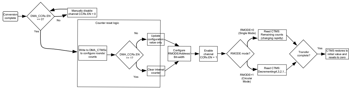
Figure18-8 DMA Operation Logic Flowchart
