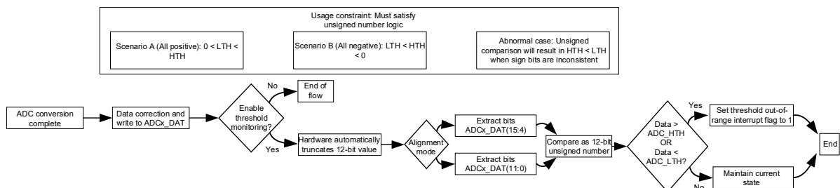
Figure 12-5 ADC Calibration and Processing Flowchart
