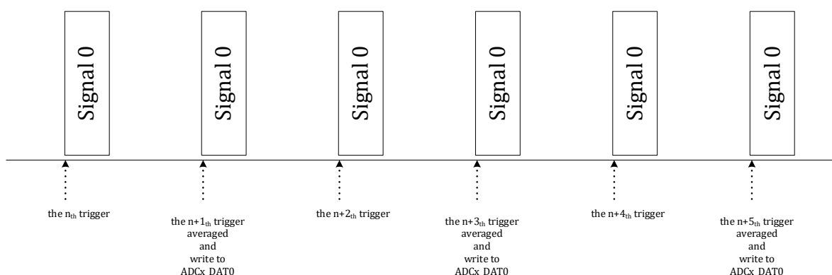
Figure 12-6 Oversampling Conversion Timing Example 1
