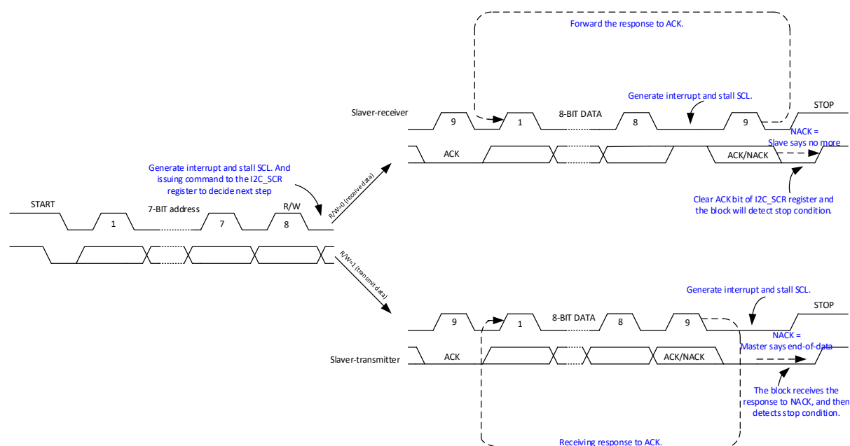
Fig. 9-5 Schematic diagram of slave mode transmission
