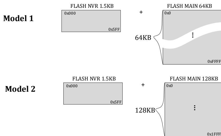
Figure7-1 Non-volatile memory space division block diagram and model
