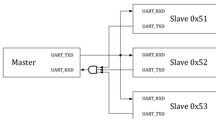
Figure17-3 UART multi-machine communication interconnection topology
