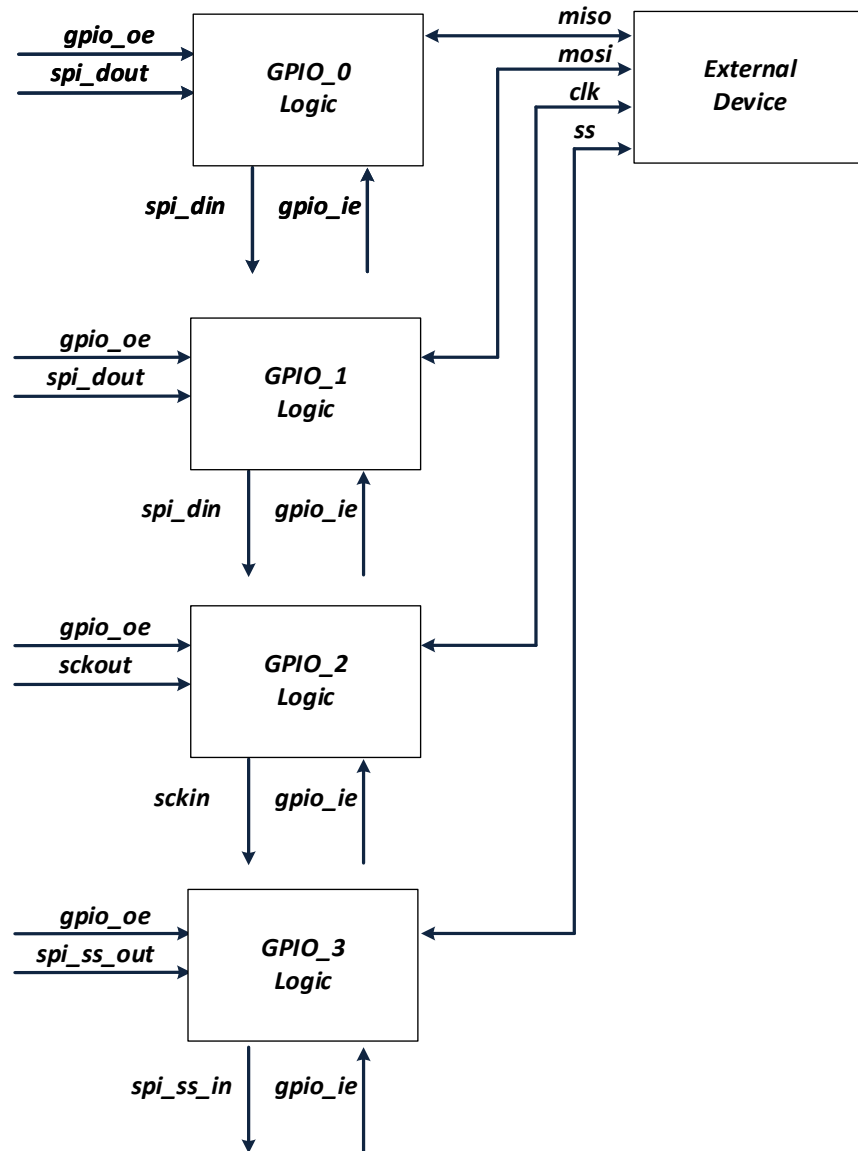
Figure 8-2 SPI Interface Full Duplex Interconnect Block Diagram
