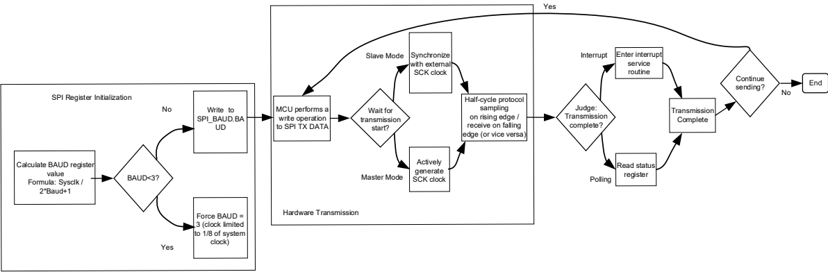
Fig. 8-1 Working Principle of SPI
