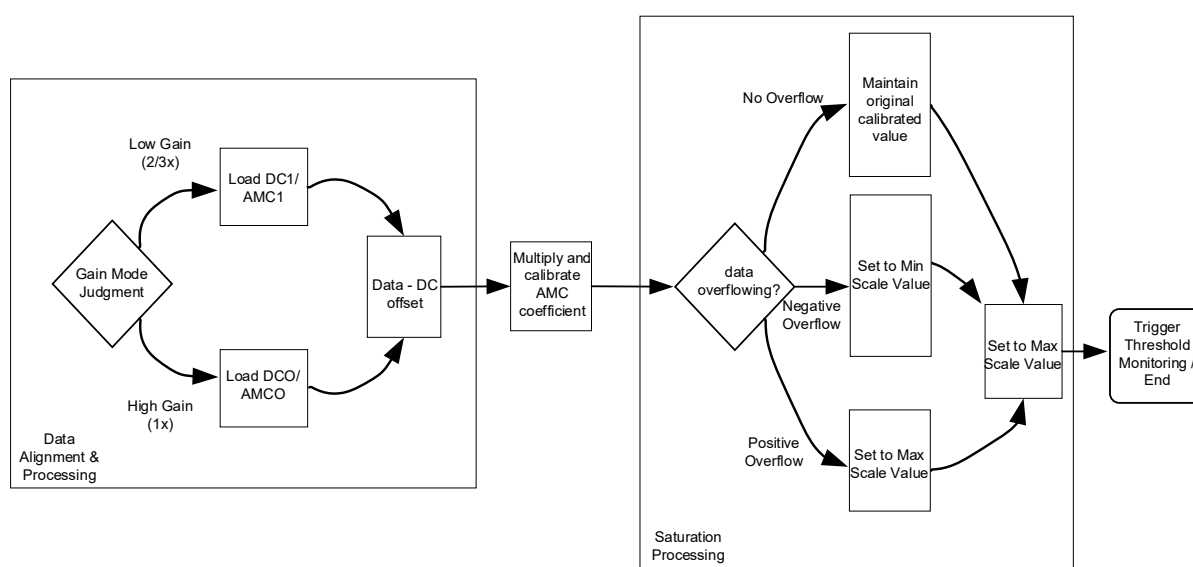
Figure 12-9 ADC Auto-Calibration Logic Flowchart
