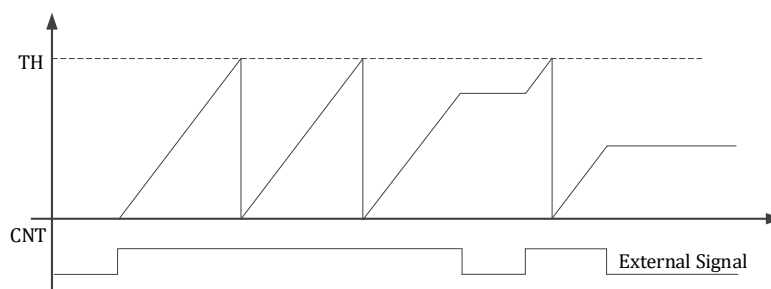
Figure13-12 TIMER external signal gating function
