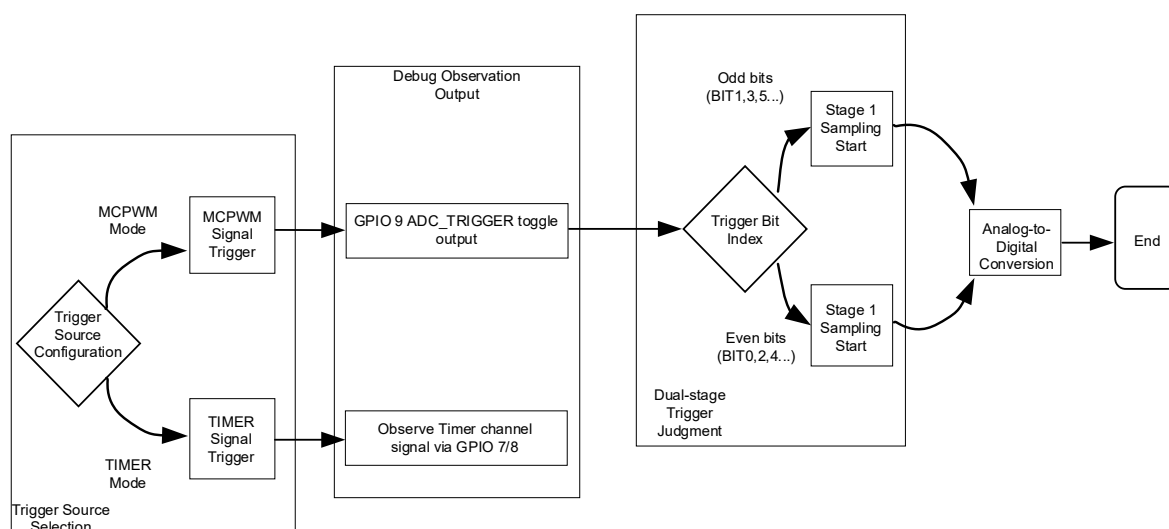
Figure 12-8 ADC Trigger and Debug Observation Flowchart
