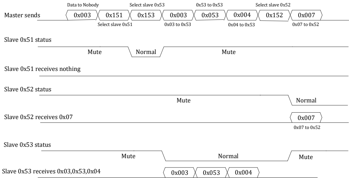
Figure17-4 UART Multi-machine Communication Example
