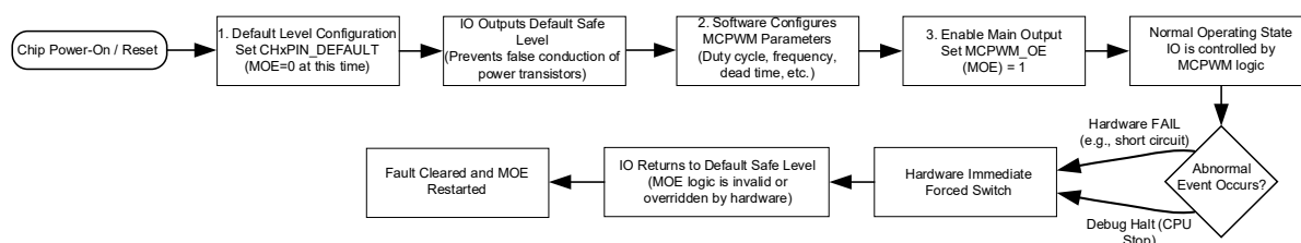
Figure14-12 Flow Chart of Fail-Safe Protection and Output Control
