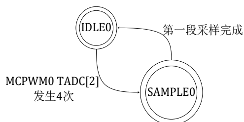
Figure 12-10 ADC Single Segment Sampling State Transition Diagram
