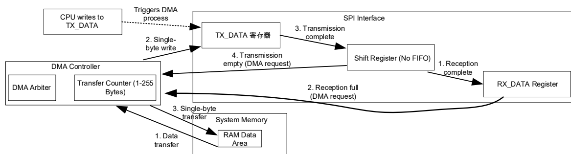
Figure 8-6 SPI DMA Data Flow and Handshake Logic Diagram
