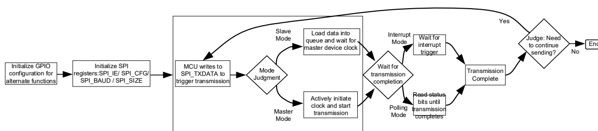
Figure 8-7 SPI Transmission Software Configuration and Operation Flow
