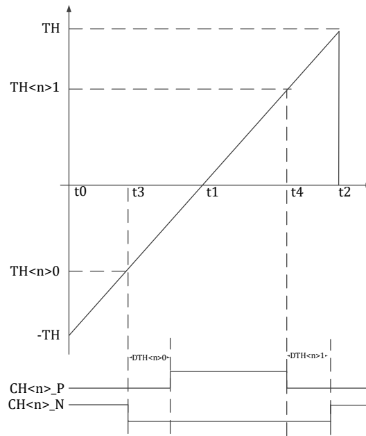
Figure14-7MCPWM Timings TH &lt; n &gt; 0 and TH &lt; n &gt; 1-Center Alignment Mode
