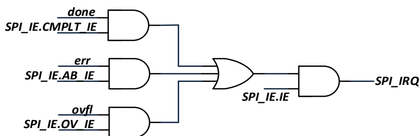
Figure 8-8 SPI module interrupt selection signal generation diagram
