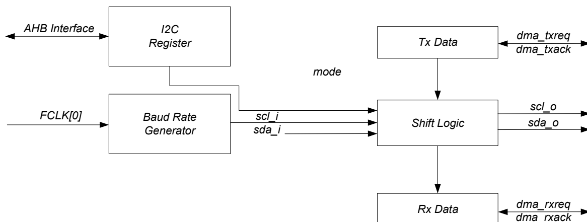
Fig. 9-1 I2C Module Top Level Functional Block Diagram
