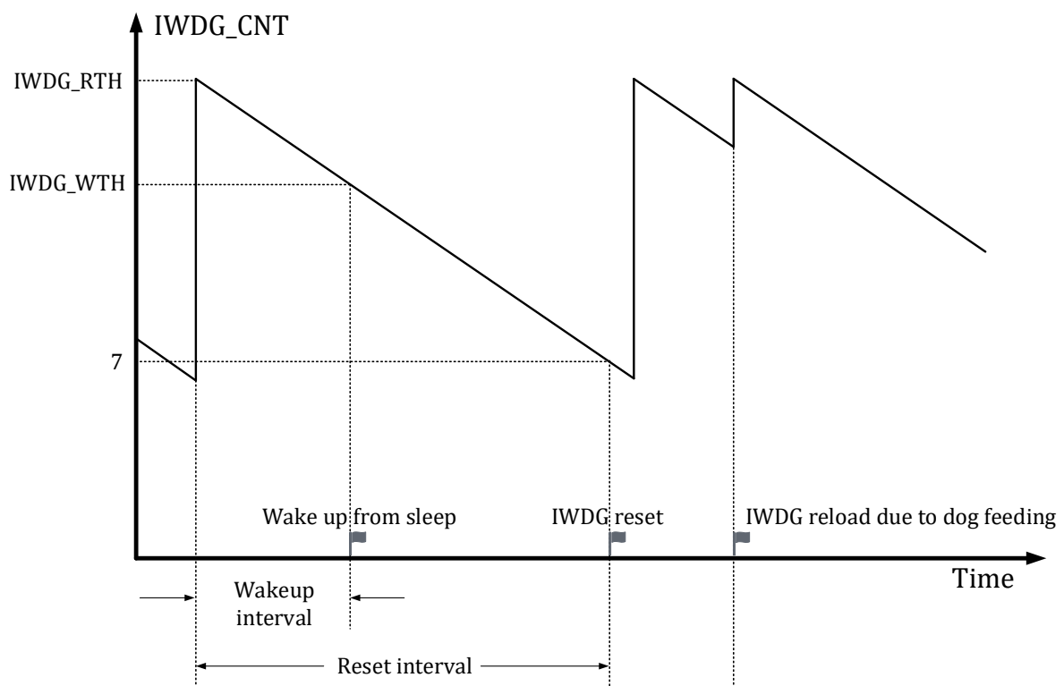
Figure 20-1 Example of an IWDG countdown event occurring
