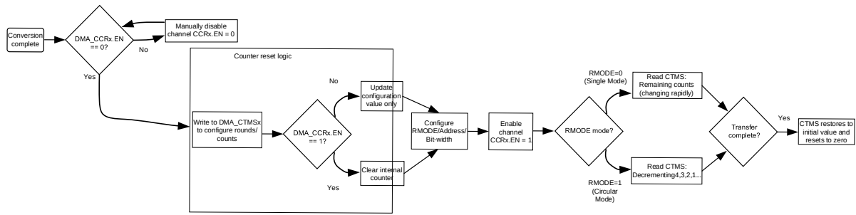
Figure18-8 DMA Operation Logic Flowchart
