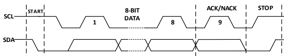
Fig. 9-2 Basic I2C Transfer Timing Diagram
