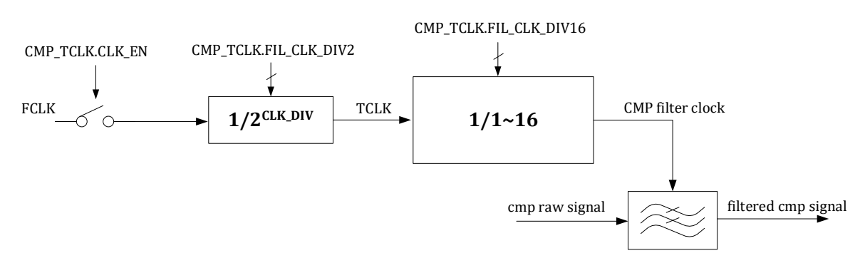
Figure 10-1 Comparator filter clock generation
