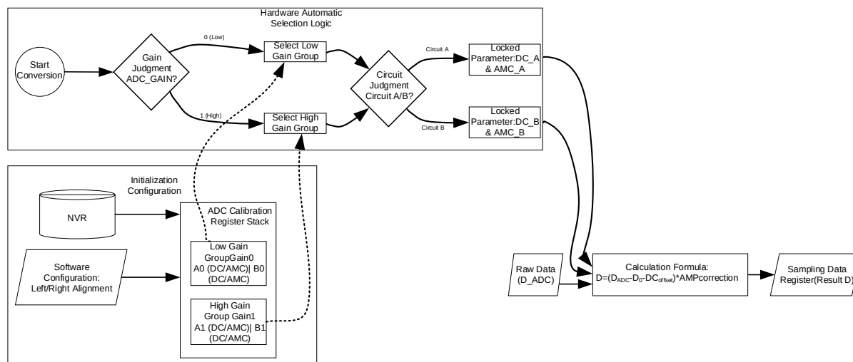
Figure 12-4 ADC Calibration Processing Flowchart
