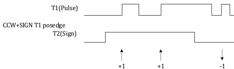
Figure 13-16 The Counts of Pulse Signal with Symbolic Data Type when the Encoder Counts only on T1 Rising Edges
