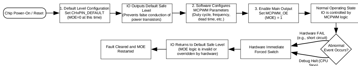
Figure14-12 Flow Chart of Fail-Safe Protection and Output Control
