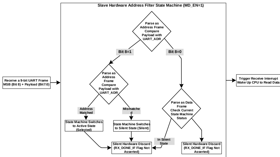
Figure17-4 Processing Flow of Slave 9-bit UART Address Frame Filter State Machine
