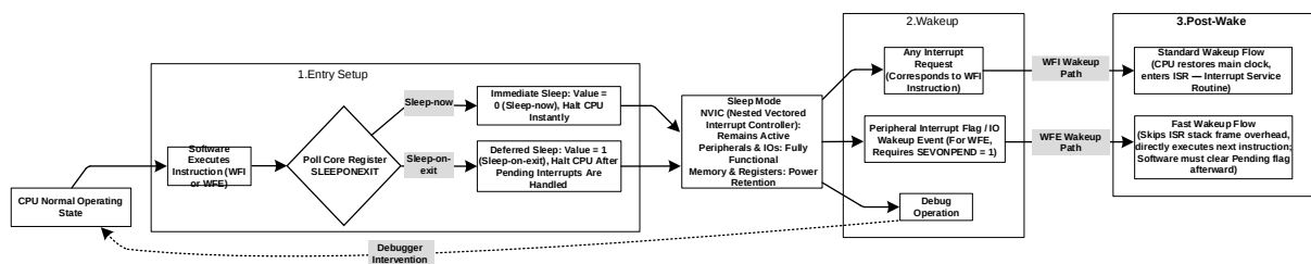
Figure 21-2 Flowchart of Conventional Sleep Mode Entry and Wakeup
