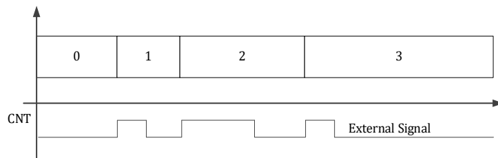
Figure 13-10 TIMER counts with an external clock
