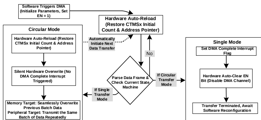
Figure18-7 Flowchart of DMA Transmission in Single Mode and Circular Mode
