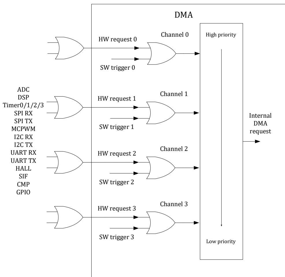
Figure18-8 DMA channel priority
