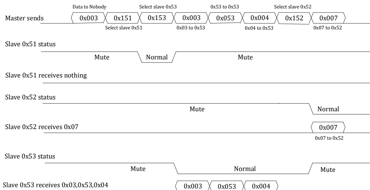
Figure17-5 UART Multi-machine Communication Example
