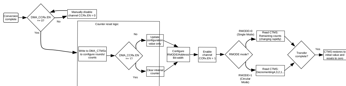
Figure 18-9 DMA Operation Logic Flowchart
