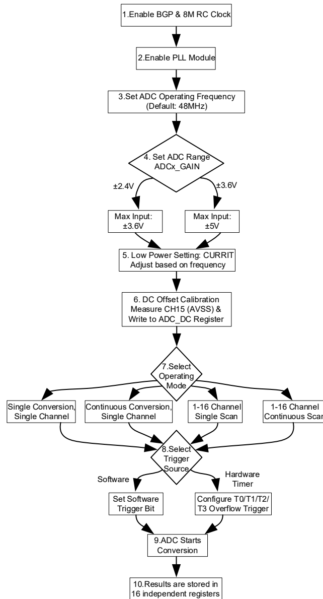
Figure 10-1ADC Configuration Flowchart
