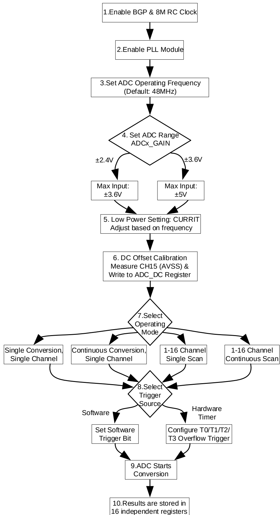
Figure 10-1ADC Configuration Flowchart
