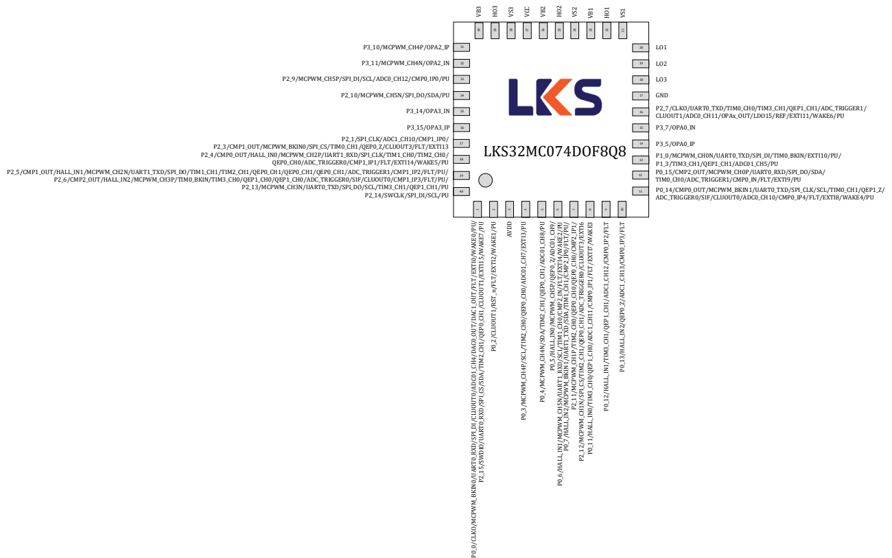
Fig.3-9 LKS32MC074DOF8Q8 Pin Assignment
