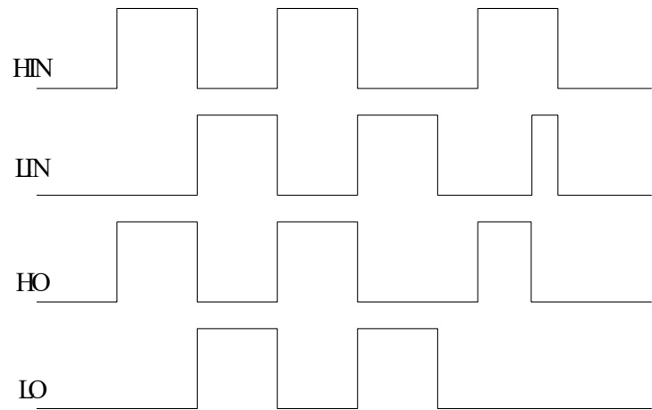
Figure 22-5 Gate Driver Module G1/G2/G3/G6 polarity illustration
