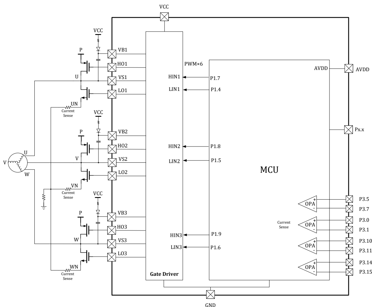
Fig.3-13 LKS32MC076FNBQ8 Schematic diagram of inner driver connection
