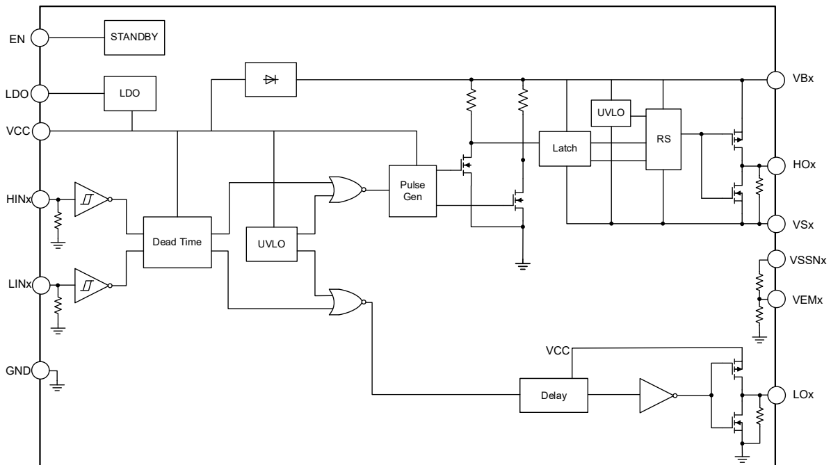
Figure22-3 Gate Driver Module G6 internal block diagram
