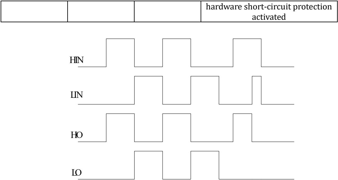
Figure 22-7 Polarity Timing Diagram of G7 Gate Driver Module
