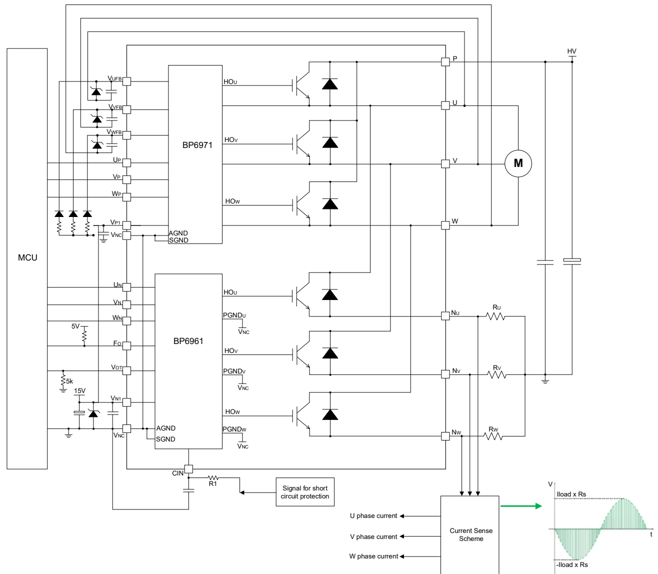
Figure 22-6 Typical Application Diagram of G7 Gate Driver Module
