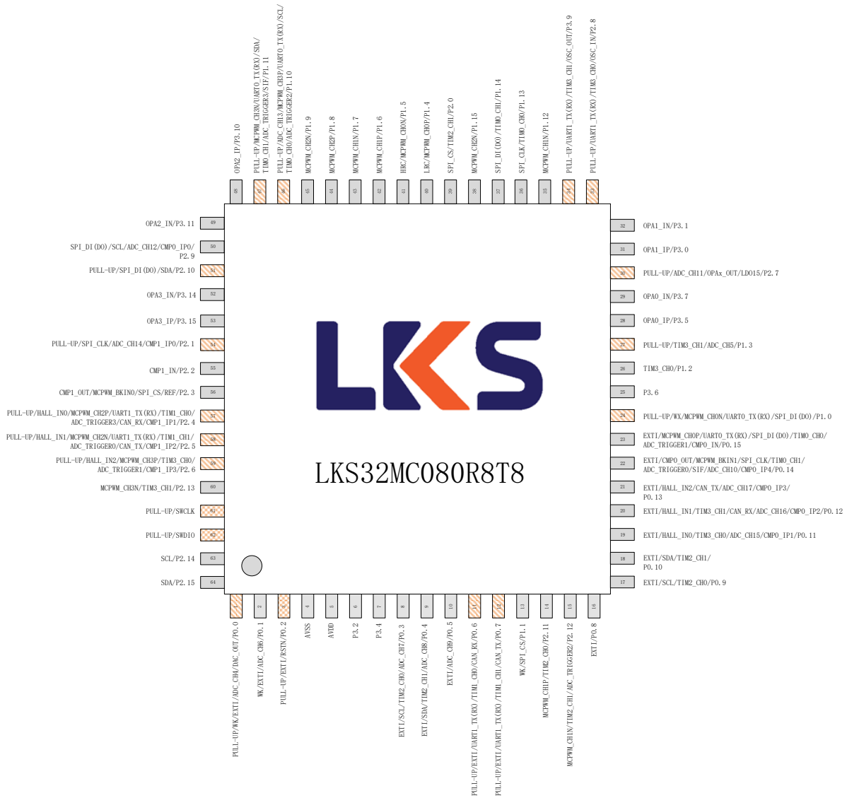
Fig. 3-1 LKS32MC080R8T8(B) Pin Assignment
