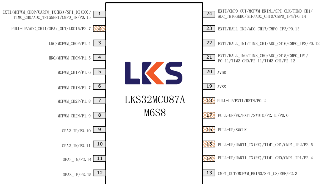
Fig. 3-6 LKS32MC087AM6S8(B) Pin Assignment
