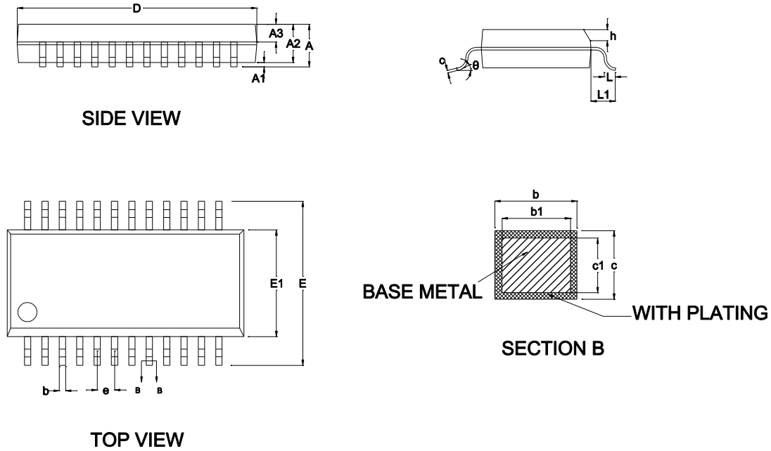
Fig. 4-4 LKS32MC087M6S8(B) Package Diagram
