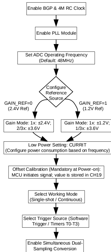
Fig. 10-1 Configuration Flowchart
