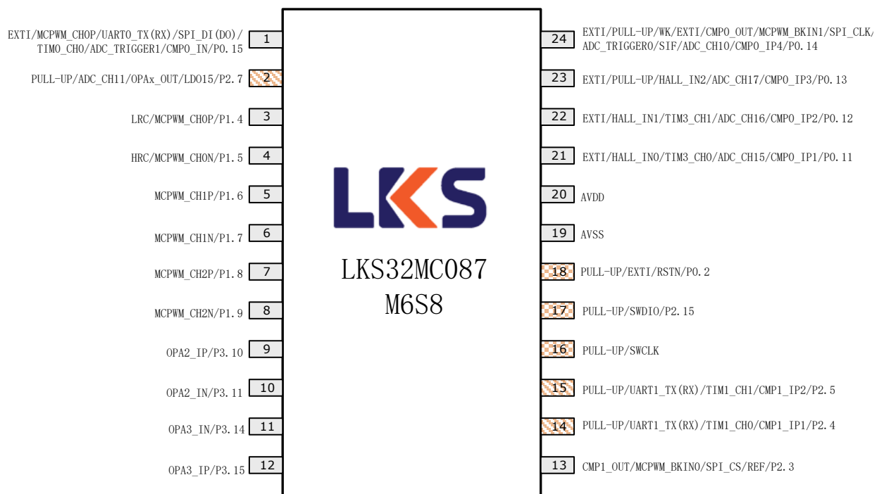
Fig. 3-5 LKS32MC087M6S8(B) Pin Assignment
