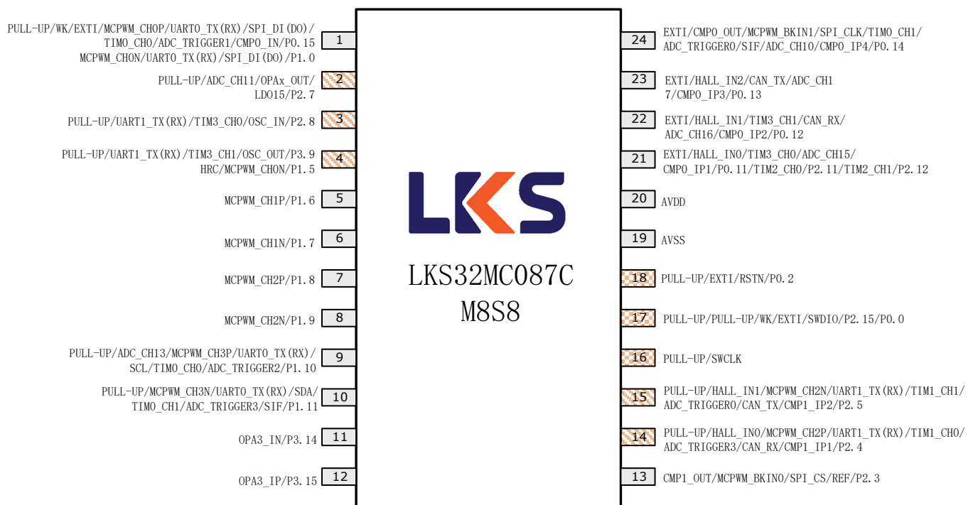
Fig. 3-7 LKS32MC087CM8S8(B) Pin Assignment
