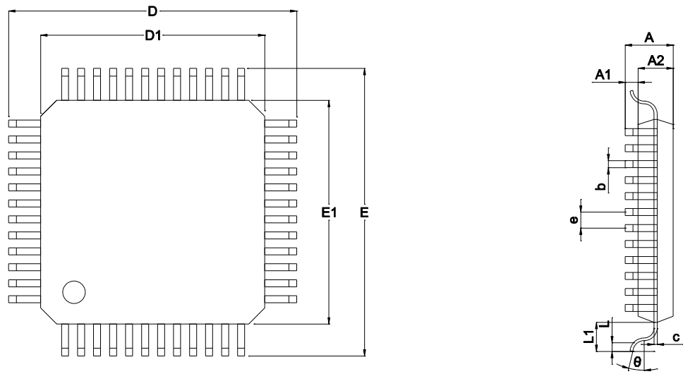
图 4-2 LKS32MC081C8T8(B)/LKS32MC083C8T8(B)/LKS32MC088C6T8(B)封装图示
