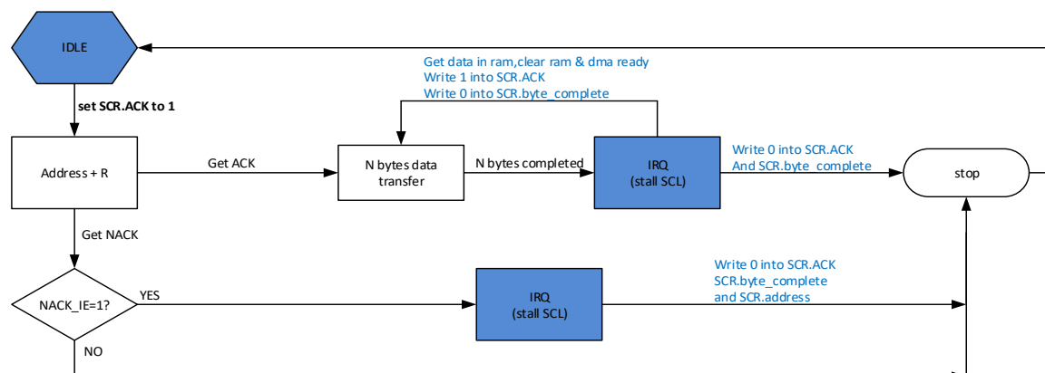
Fig. 16-12 Schematic Diagram of Multi-byte Reception in Master Mode
