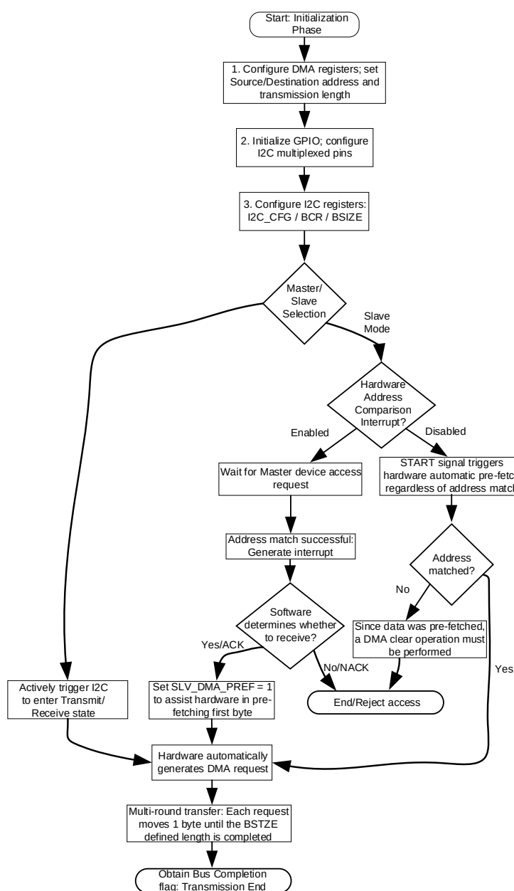
Fig. 16-13 Logic Flow Chart for DMA Configuration and Execution of I2C Interface in High-Volume Data Transmission
