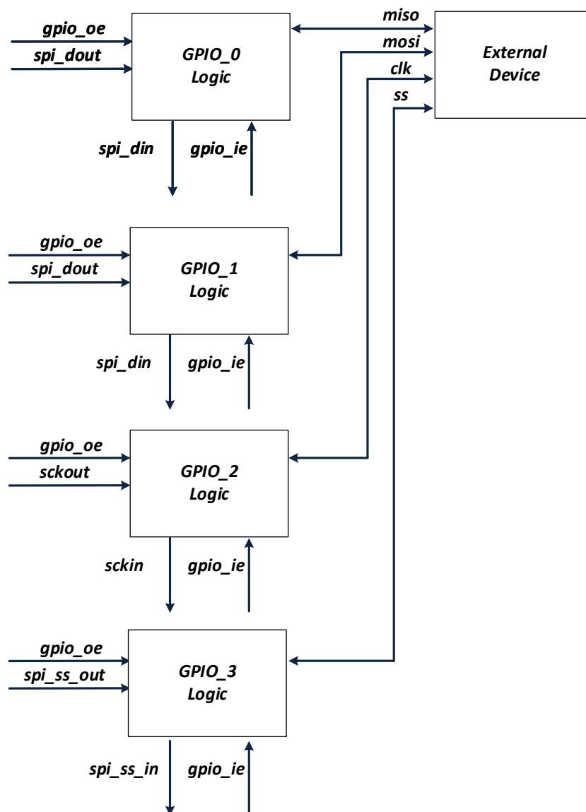
Fig. 17-2 SPI Interface Full Duplex Mode Interconnection Block Diagram
