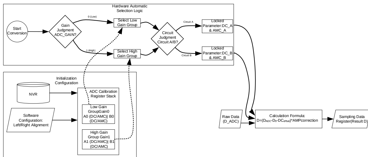
Fig. 10-4 ADC Calibration Processing Flowchart
