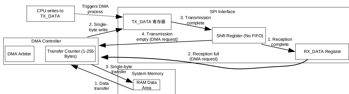
Fig. 17-10 SPI DMA Data Flow and Handshake Logic Diagram
