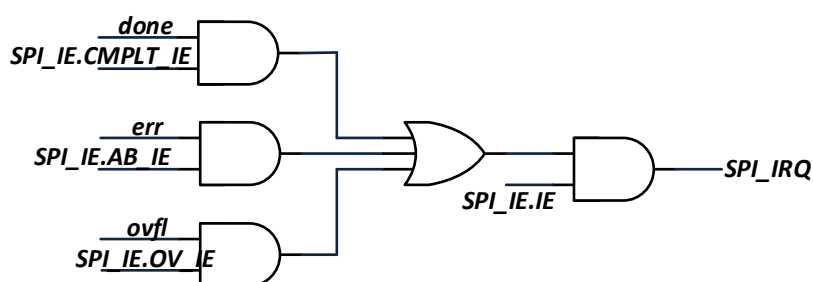
Fig. 17-13 Generation Diagram for SPI Module Interrupt Selection Signal
