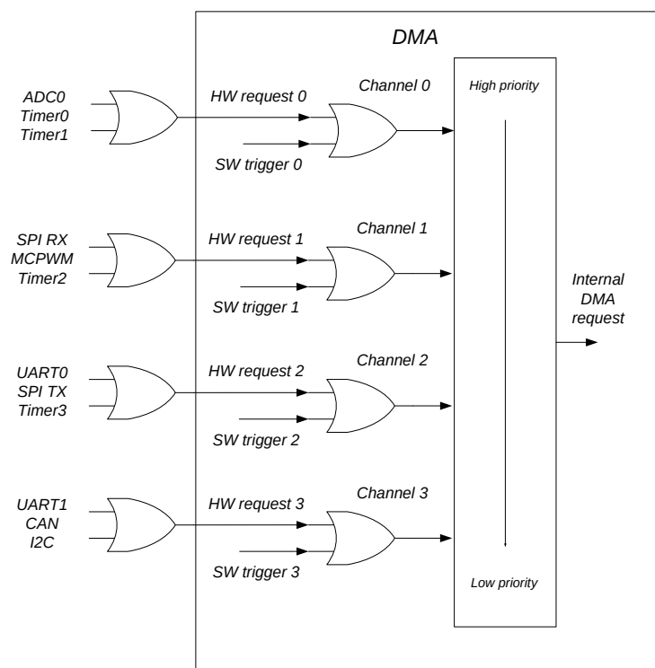
Fig. 7-4 DMA Channel Priority
