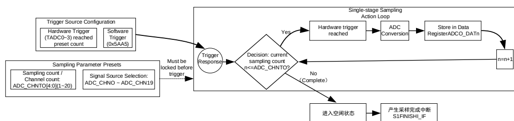
Fig. 10-7 Single-stage Sampling Operation Loop
