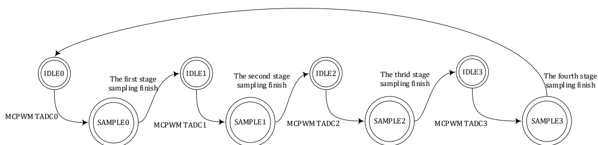
Fig. 10-10 State Transition Diagram of ADC Four-round Sampling
