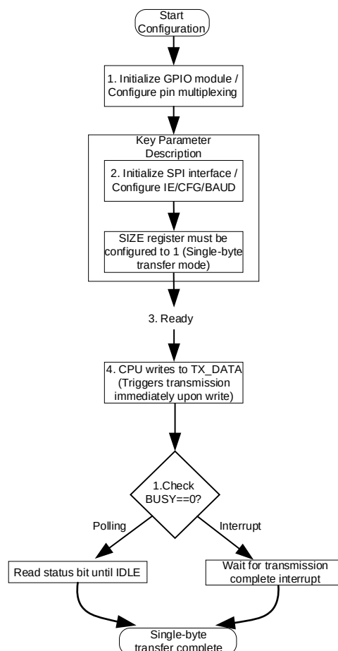
Fig. 17-12 Software Configuration Flowchart
