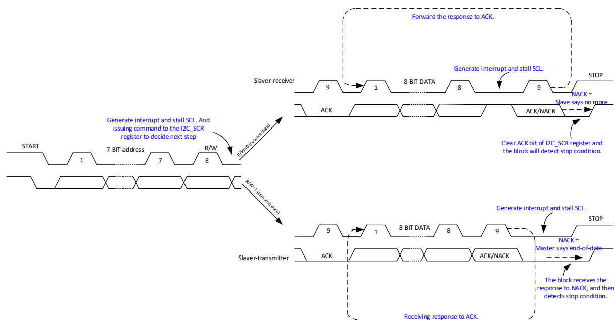
Fig. 16-5 Schematic Diagram of Single-byte Transmission in Slave Mode
