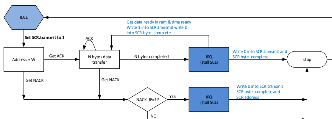
Fig. 16-11 Schematic Diagram of Multi-byte Transmission in Master Mode
