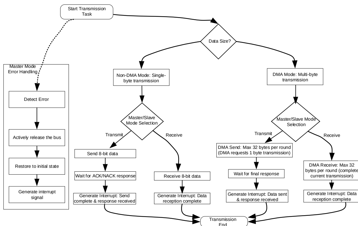
Fig. 16-3 I2C Transmission Mode Decision and Execution Flowchart
