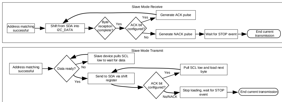
Fig. 16-6 I2C Slave Mode (Transmit/Receive/DMA) Logic Flowchart
