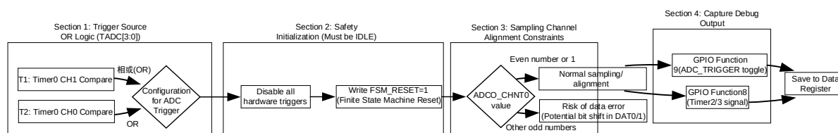
Fig. 10-5 ADC Trigger and Channel Alignment Logic
