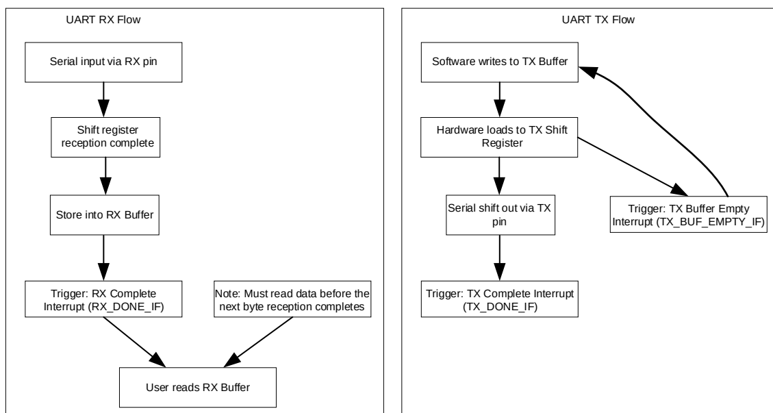
Fig. 14-1 UART Transmit and Receive Interrupts
