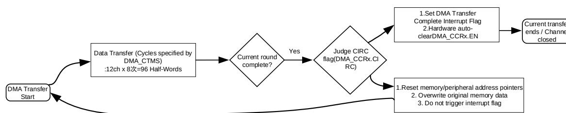
Fig. 7-3 DMA Transfer Mode Logic Flowchart
