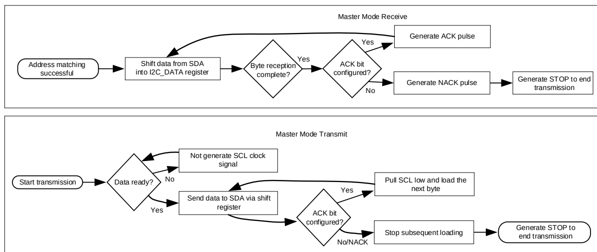
Fig. 16-10 Logic Flow Chart for I2C Master Mode Transmission and Reception
