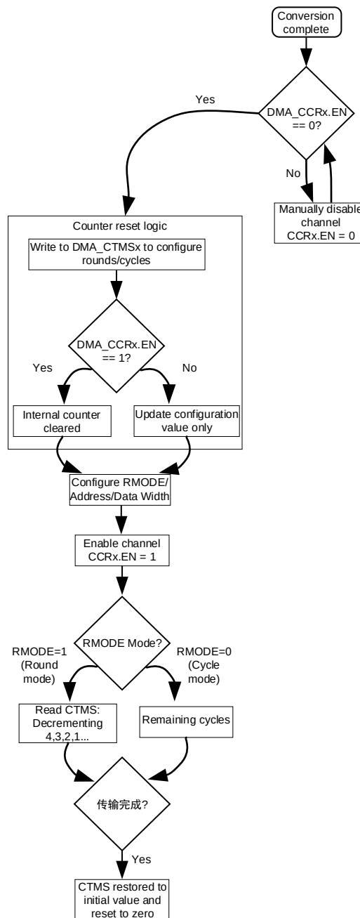
Fig. 7-5 DMA Operational Logic Flowchart
