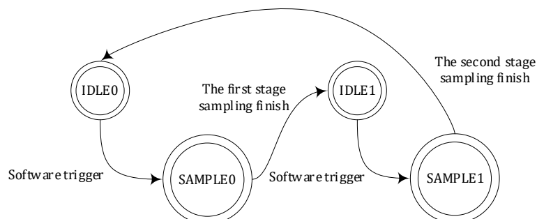
Fig. 10-9 State Transition Diagram of ADC Two-round Sampling
