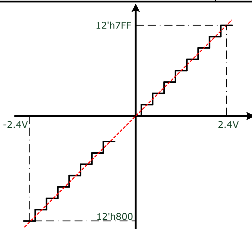
Fig. 10-3 ADC Digital Range at Double Gain Setting
