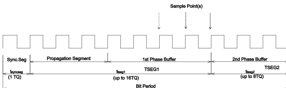
Fig. 19-2 CAN Module Bit Cycle Introduction Diagram
