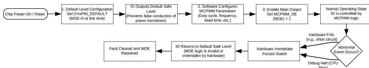
Fig. 13-12 Flow Chart of Fail-Safe Protection and Output Control
