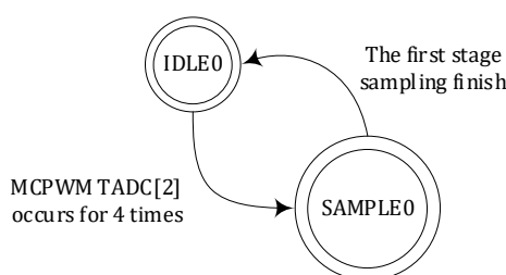
Fig. 10-8 State Transition Diagram of ADC Single-round Sampling
