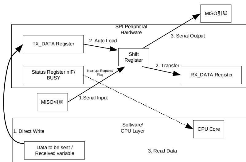
Fig. 17-11 SPI CPU Data Transfer Stream Block Diagram
