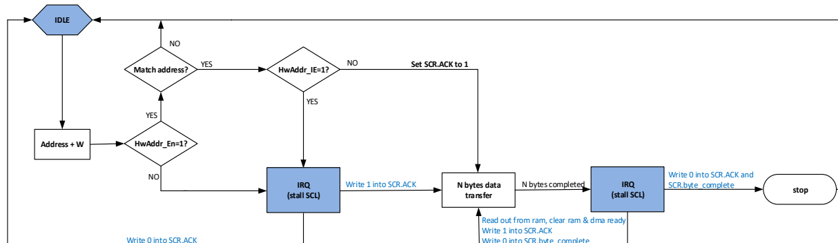
Fig. 16-8 Schematic Diagram of Multi-byte Reception in Slave Mode
