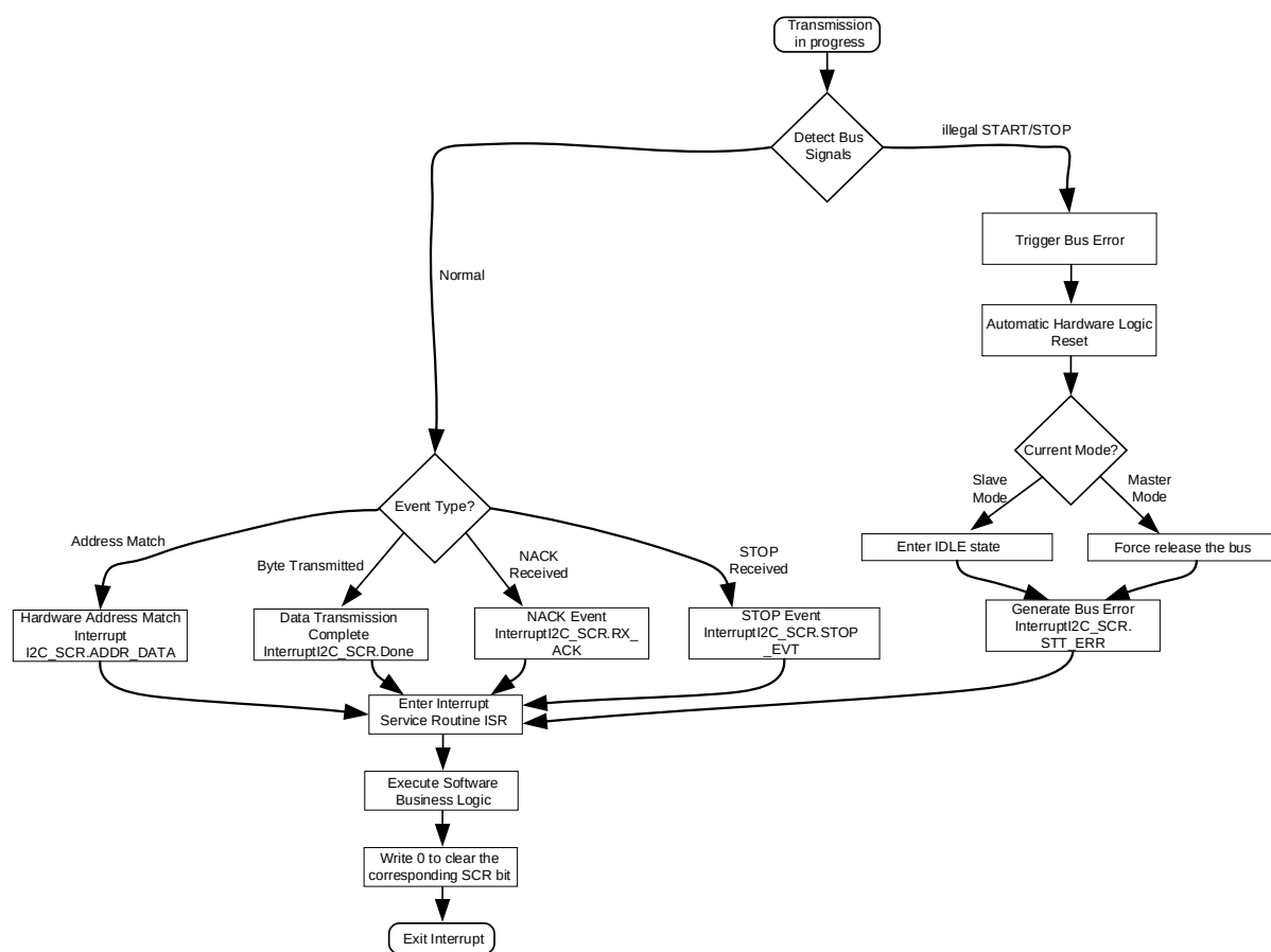
Fig. 16-14 Logic Flow Chart for I2C Bus Error Handling and Interrupt Management
