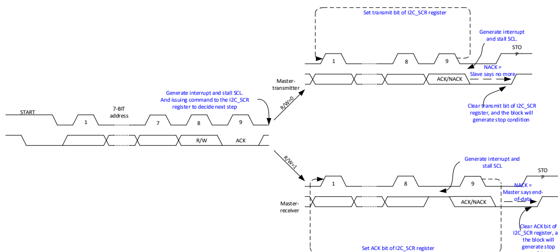
Fig. 16-9 Schematic Diagram of Single-byte Transmission in Master Mode
