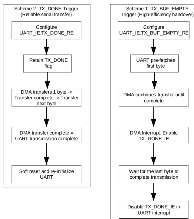
Fig. 14-2 UART DMA Transmission Comparison
