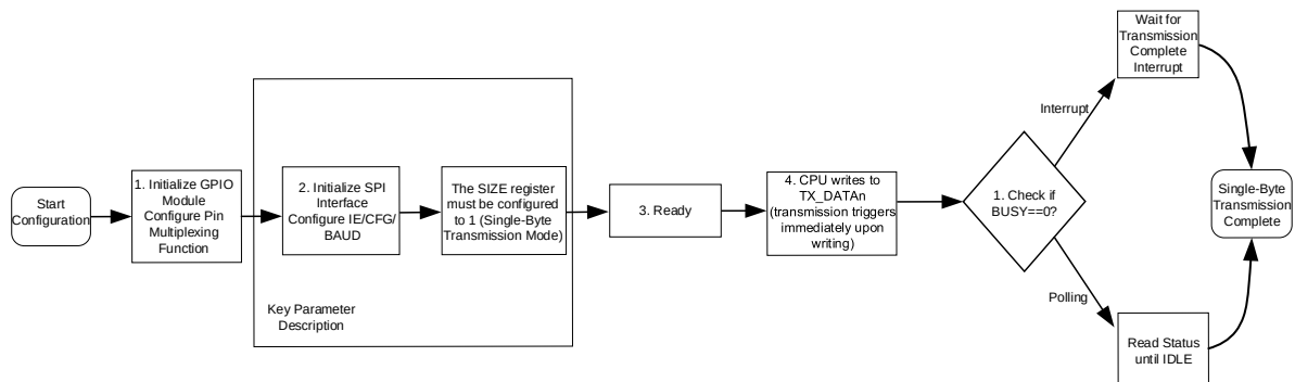
Fig. 17-14 Working Principle of SPI
