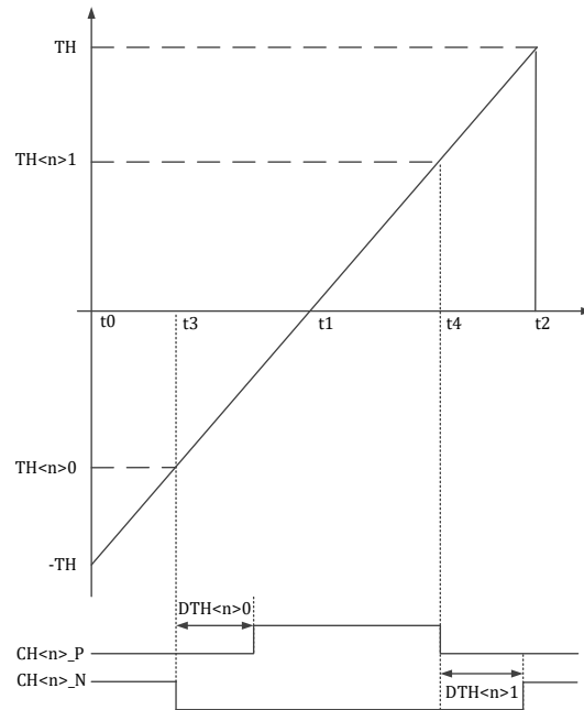
Fig. 13-7 MCPWM Timing TH_{<n>0} and TH_{<n>1} ——Complementary Mode
