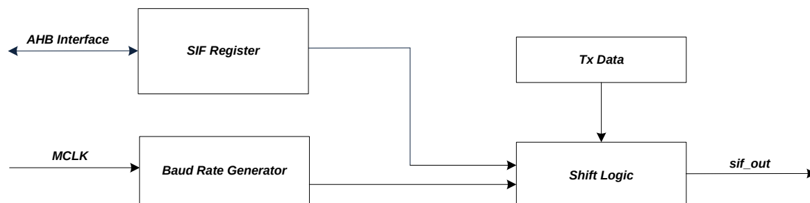
Fig. 20-1 SIF Module Top Functional Block Diagram
