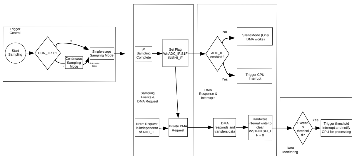
Fig. 10-6 Trigger Control and DMA Flow
