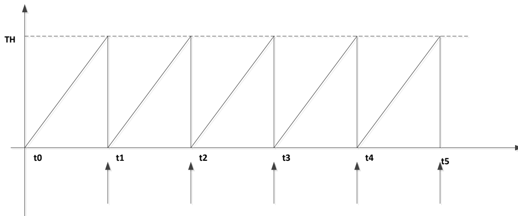
Fig. 11-3 General Counter
