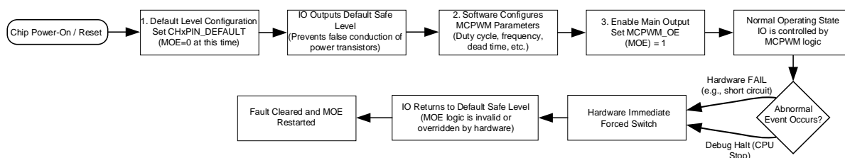
Fig. 13-12 Flow Chart of Fail-Safe Protection and Output Control
