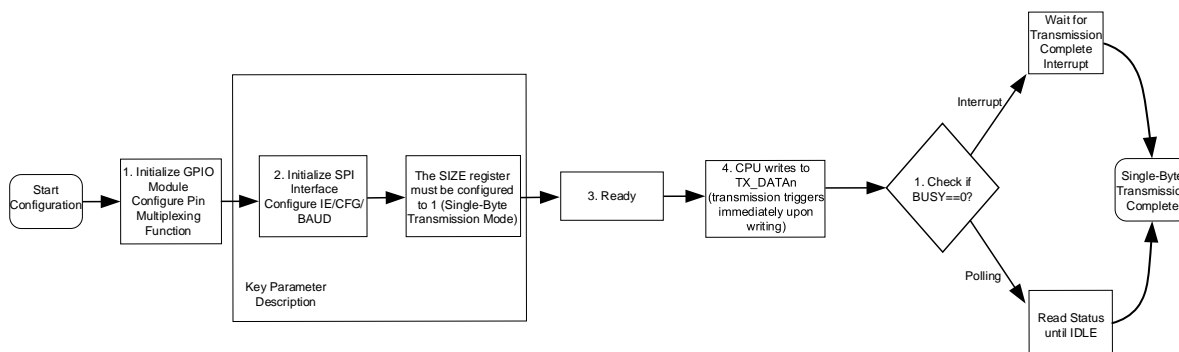
Fig. 17-14 Working Principle of SPI
