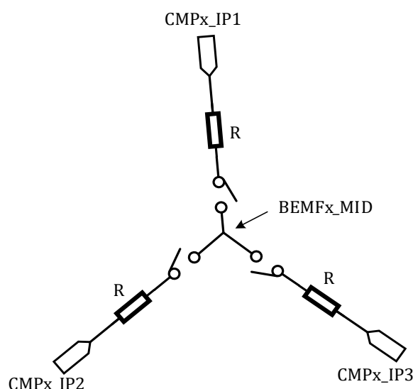
Fig. 18-2 BEMF x _MID Signal
