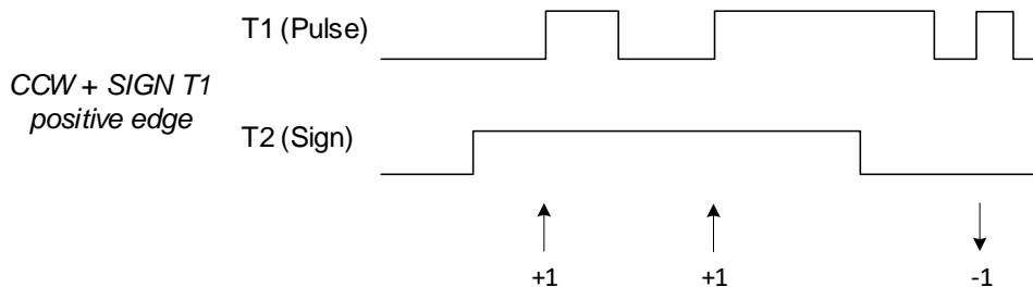
Fig. 11-9 The Counts of Pulse Signal with Symbolic Data Type when the Encoder Counts only on T1 Rising Edges
