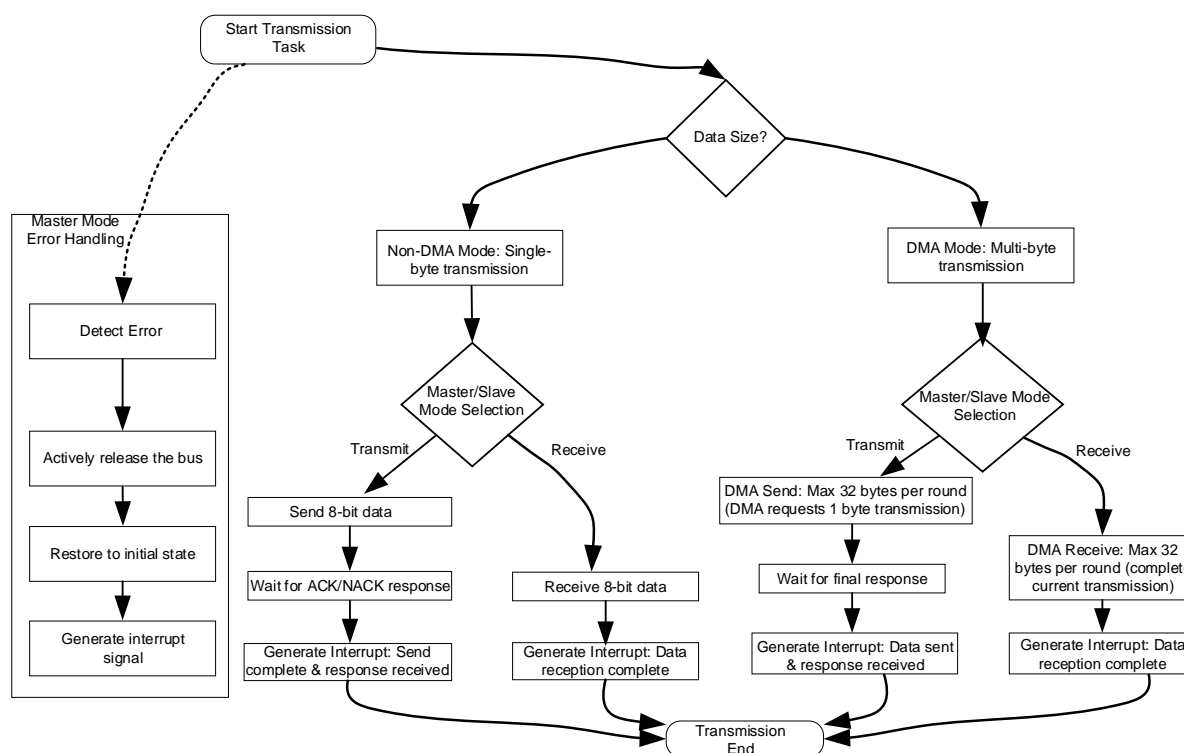
Fig. 16-3 I2C Transmission Mode Decision and Execution Flowchart
