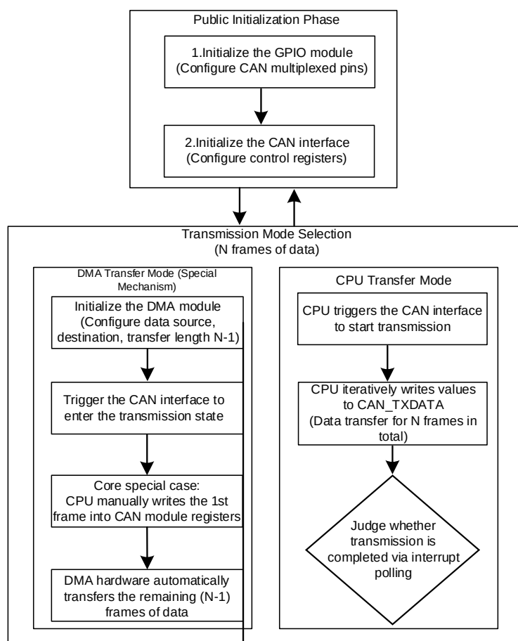
Fig. 19-2 CAN Multi-frame Data Transmission Workflow: DMA Mode vs CPU Mode
