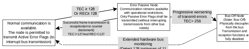
Fig. 19-8 Schematic Diagram for Three Error State Transitions of the CAN Controller
