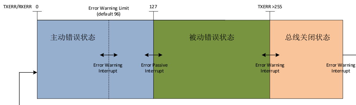
Fig. 19-7 CAN Module Error Management
