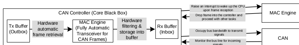
Fig. 19-6 Error Management of CAN Module
