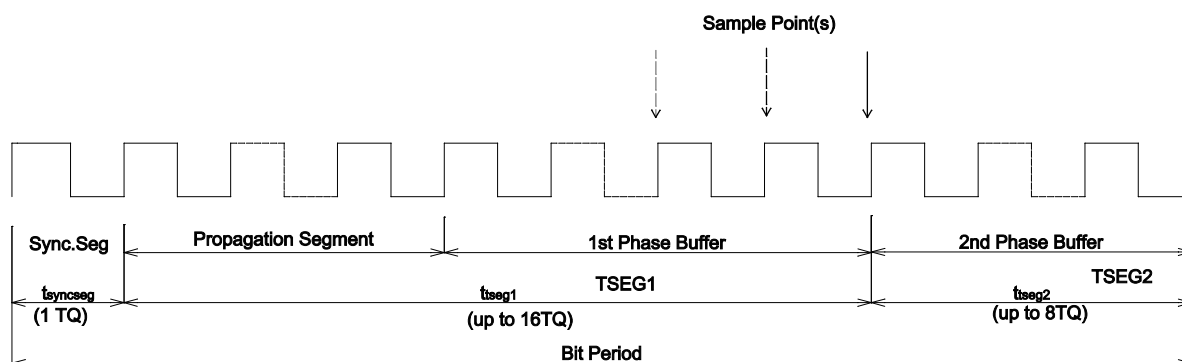
Fig. 19-4 CAN Module Bit Cycle Introduction Diagram
