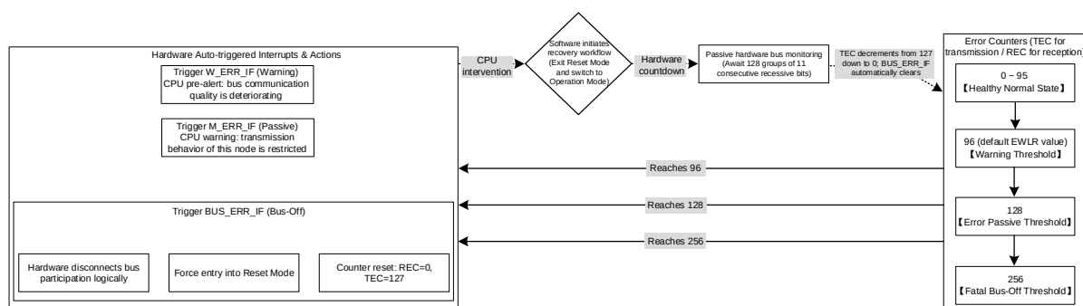
Fig. 19-9 CAN Fault-Graded Interrupt Reporting and Bus-Off Recovery Flow
