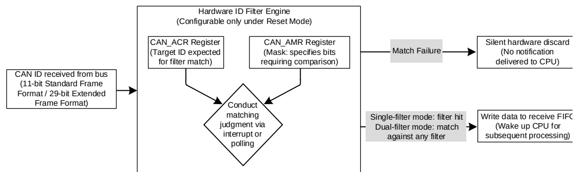
Fig. 19-5 CAN Hardware ID Filter Reception Judgment Flow
