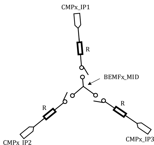
Fig. 18-2 BEMF_MID Signal
