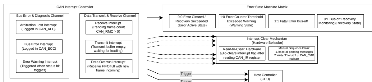
图 19-3 CAN Module Interrupt Handling and State Machine Architecture
