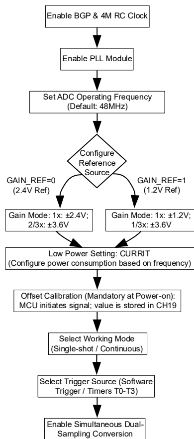
Fig. 10-1 Configuration Flowchart
