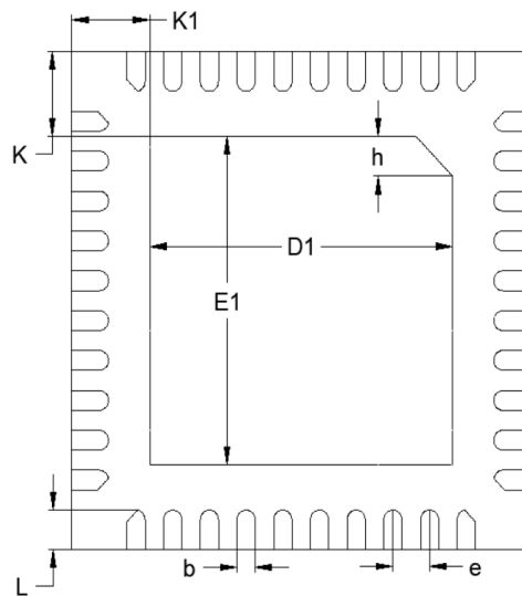
BOTTOM VIEW
