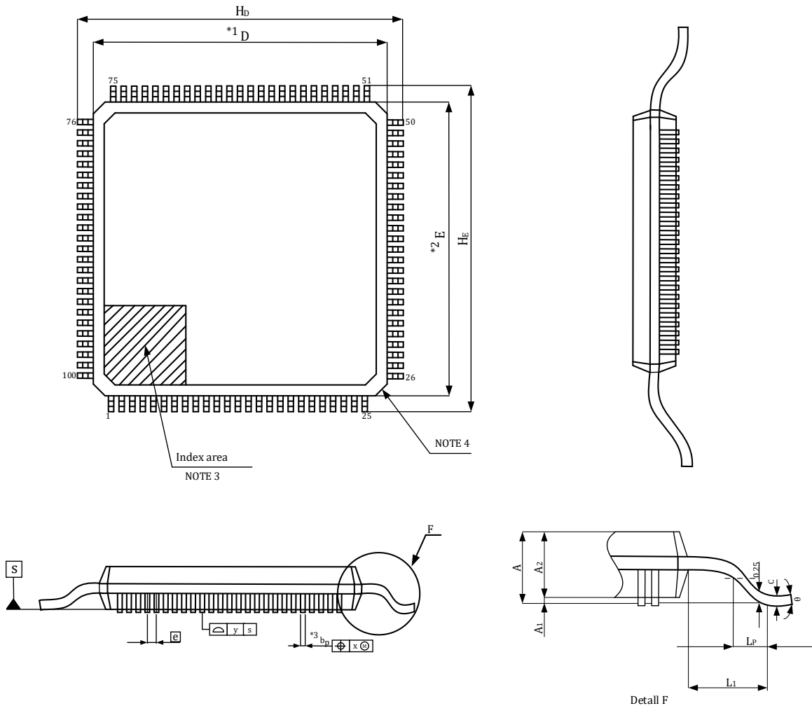
Figure 4-1 LKS32MC451VCT8 package diagram
