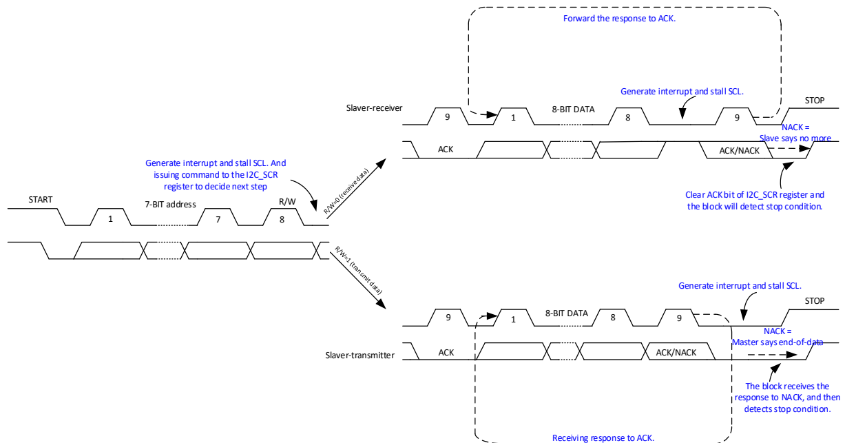
Figure 18-5 Schematic Diagram of Transmission in Slave Mode
