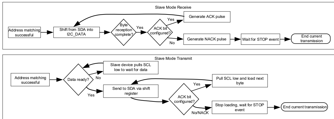
Figure 18-6 I2C Slave Mode (Transmit/Receive) Logic Flowchart
