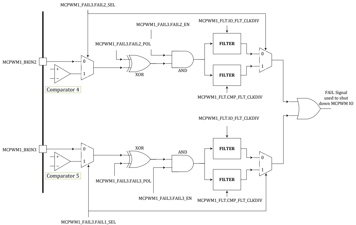
Figure 16-8 MCPWM1 FAIL2/3 Logic Diagram
