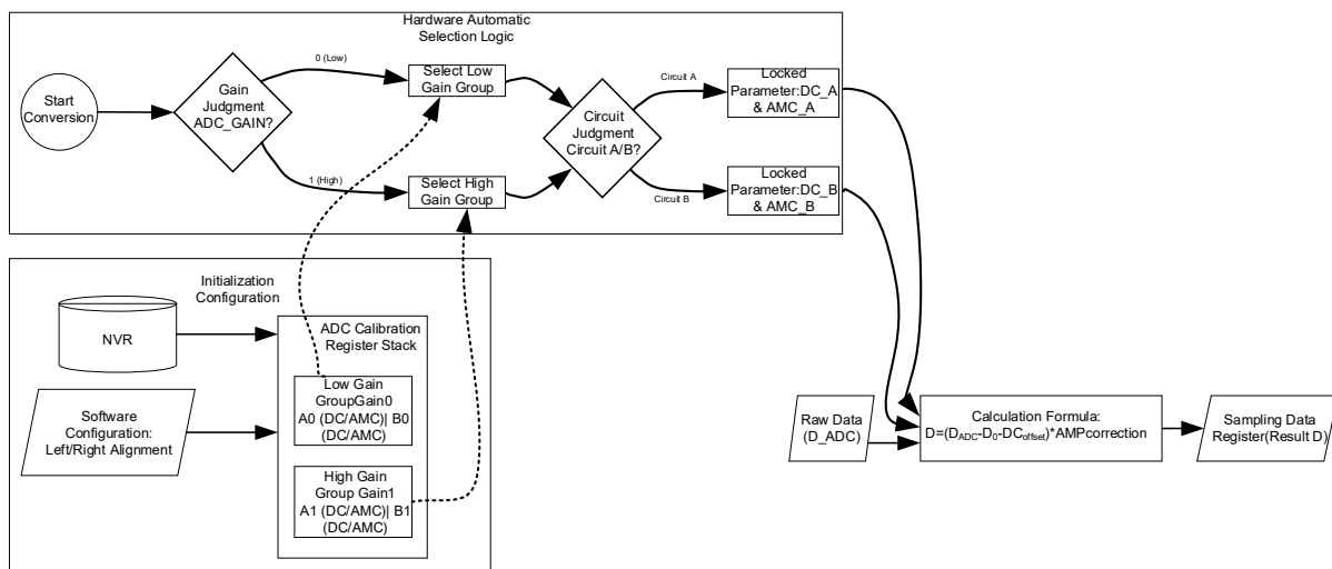
Figure 13-3 ADC Calibration Processing Flowchart
