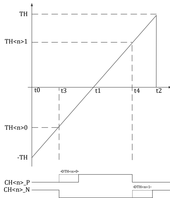
Figure 16-11 MCPWM Timing TH0 and TH1 - Complementary Mode
