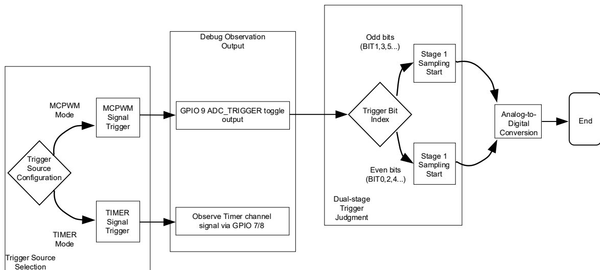
Figure 13-7 ADC Trigger and Debug Observation Flowchart
