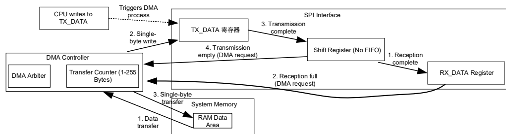
Figure 19-6 SPI DMA Data Flow and Handshake Logic Diagram
