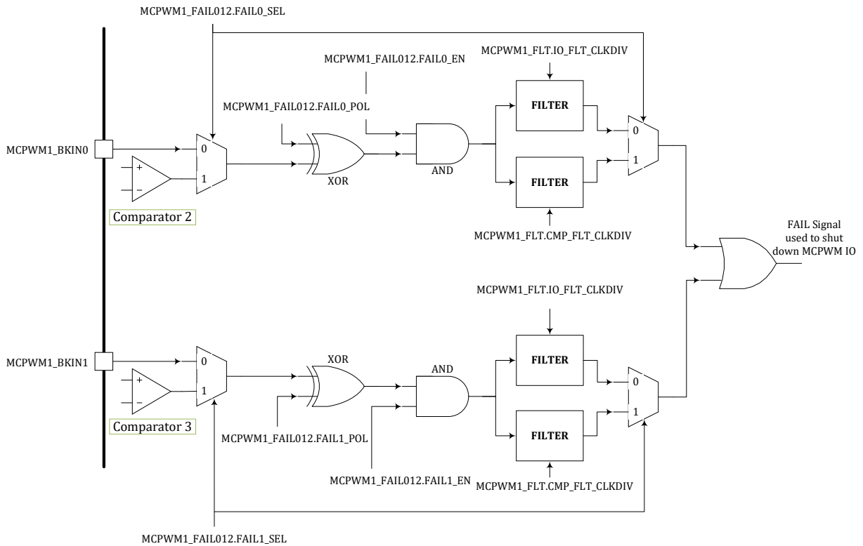
Figure 16-7 MCPWM1 FAIL0/1 Logic Diagram
