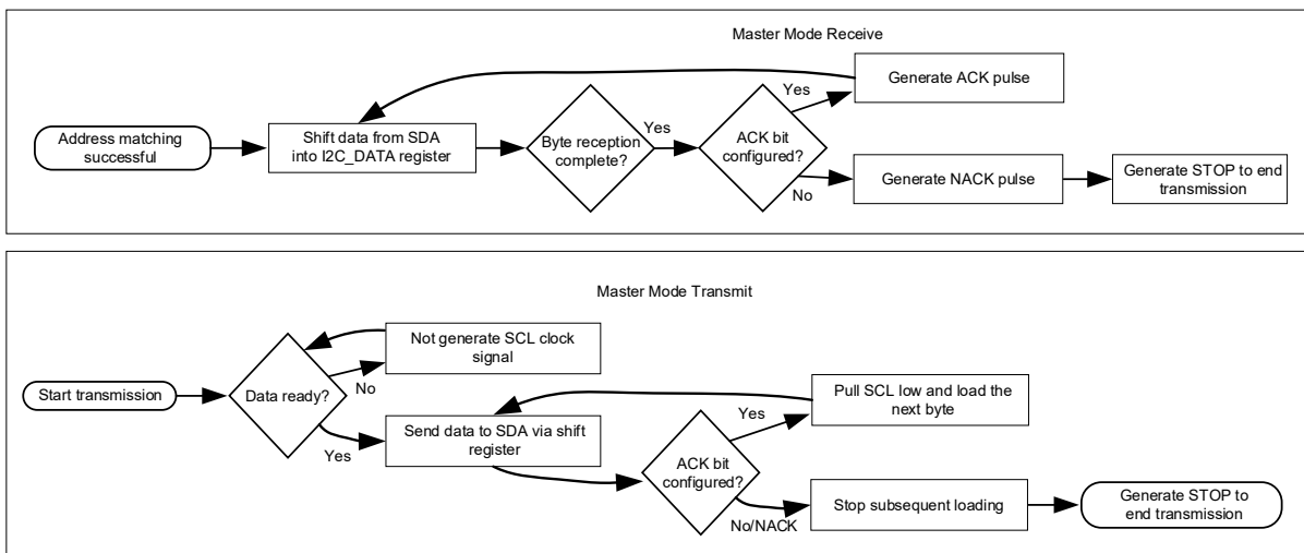
Figure 18-8 Logic Flow Chart for I2C Master Mode Transmission and Reception
