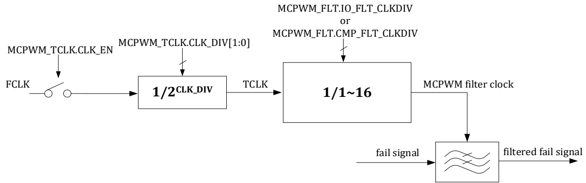
Figure 16-9 MCPWM Fail Signal Filtering Clock Generation Logic
