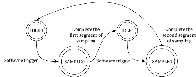
Figure 13-11 State Transition Diagram of ADC Two-round Sampling
