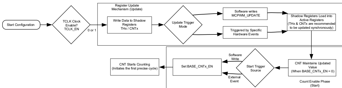
Figure 16-4 Flow Chart of Time Base Register Update and Count Enable
