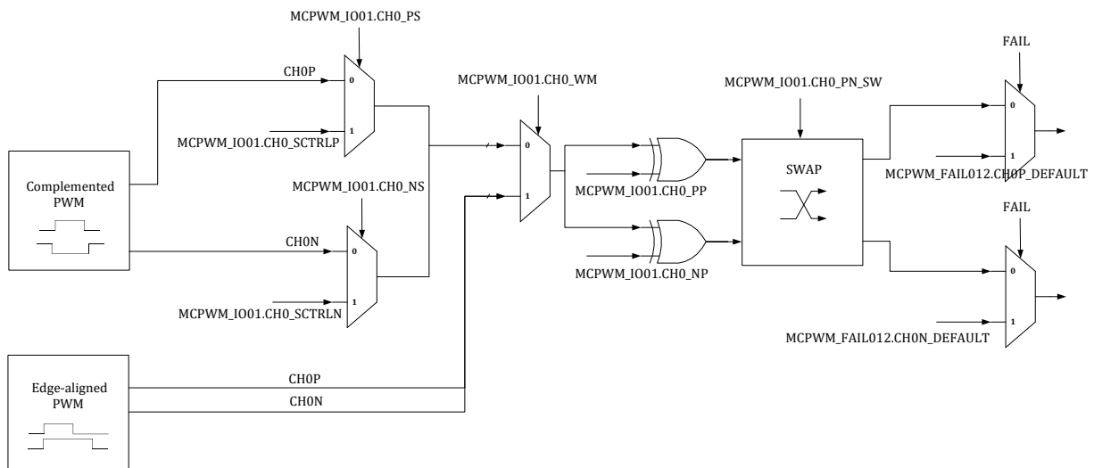
Figure 16-10 IO Driver Module Data Flow Chart
