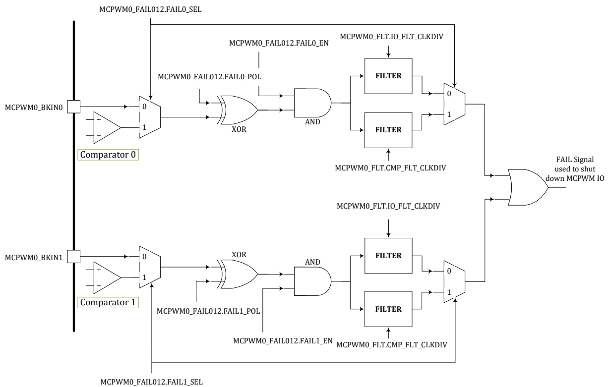
Figure 16-5 MCPWM0 FAIL0/1 Logic Diagram
