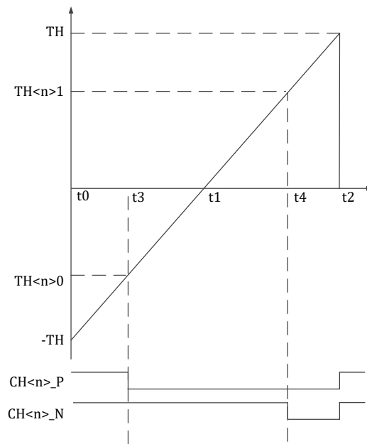
Figure 16-13 MCPWM Timing Edge-aligned Mode
