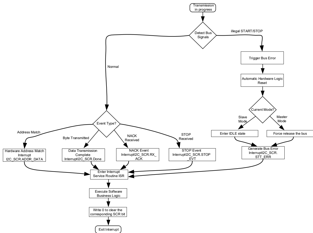
Figure 18-9 Logic Flow Chart for I2C Bus Error Handling and Interrupt Management
