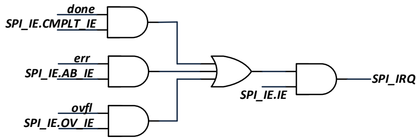
Figure 19-8 Generation Diagram for SPI Module Interrupt Selection Signal
