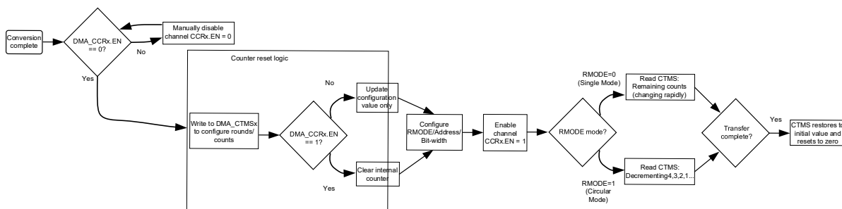
Figure8-1 DMA Operation Logic Flowchart
