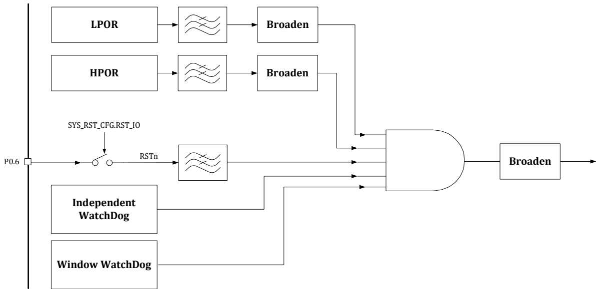
Figure 6-2 Reset Architecture
