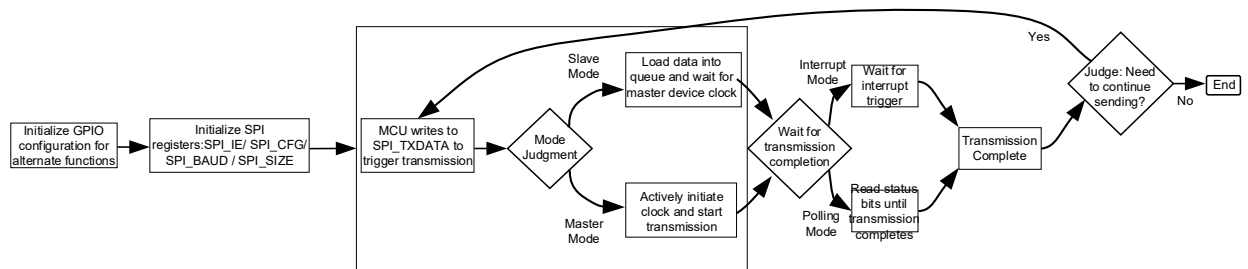
Figure 19-7 SPI Transmission Software Configuration and Operation Flow
