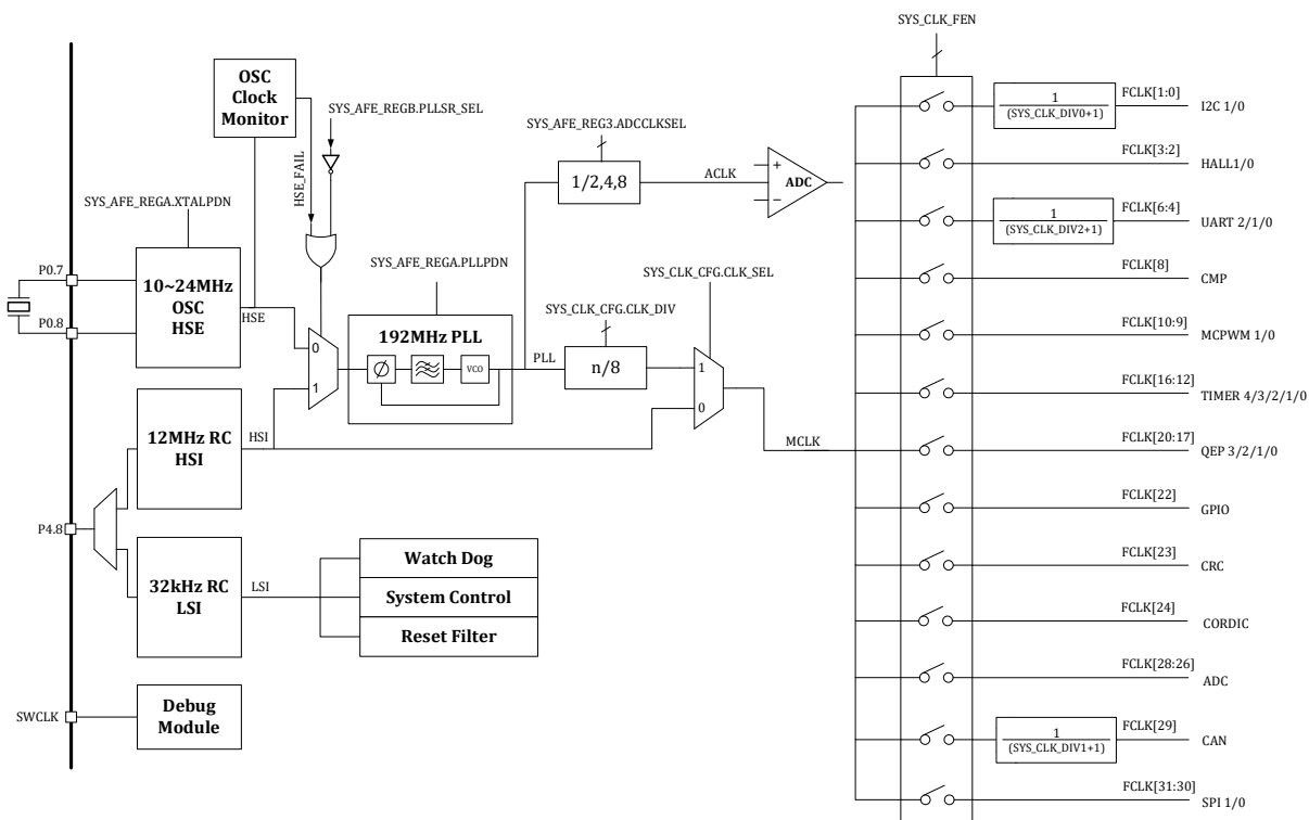
Figure 6-1 Clock Source
