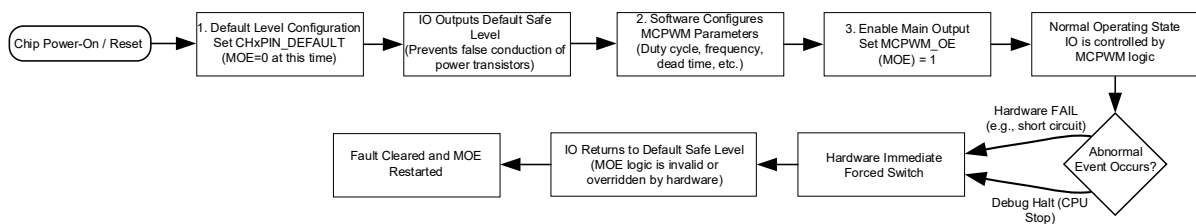
Figure 16-16 Flow Chart of Fail-Safe Protection and Output Control
