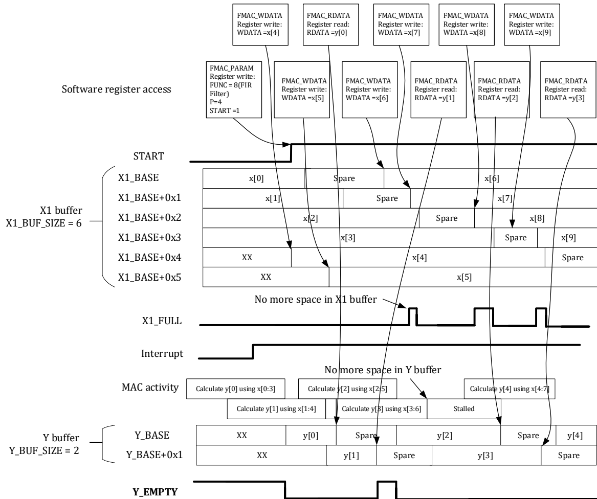
Figure 12-11 Filtering example 1
