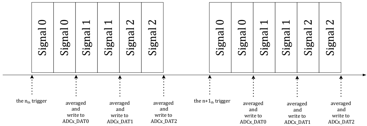
Figure 13-5 Oversampling Conversion Sequence Sample 1
