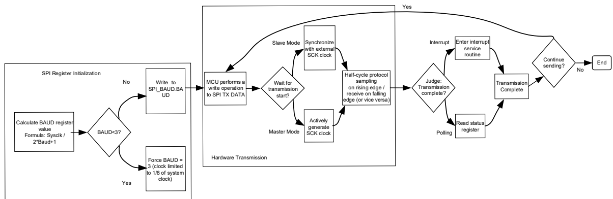
Figure 19-9 Working Principle of SPI
