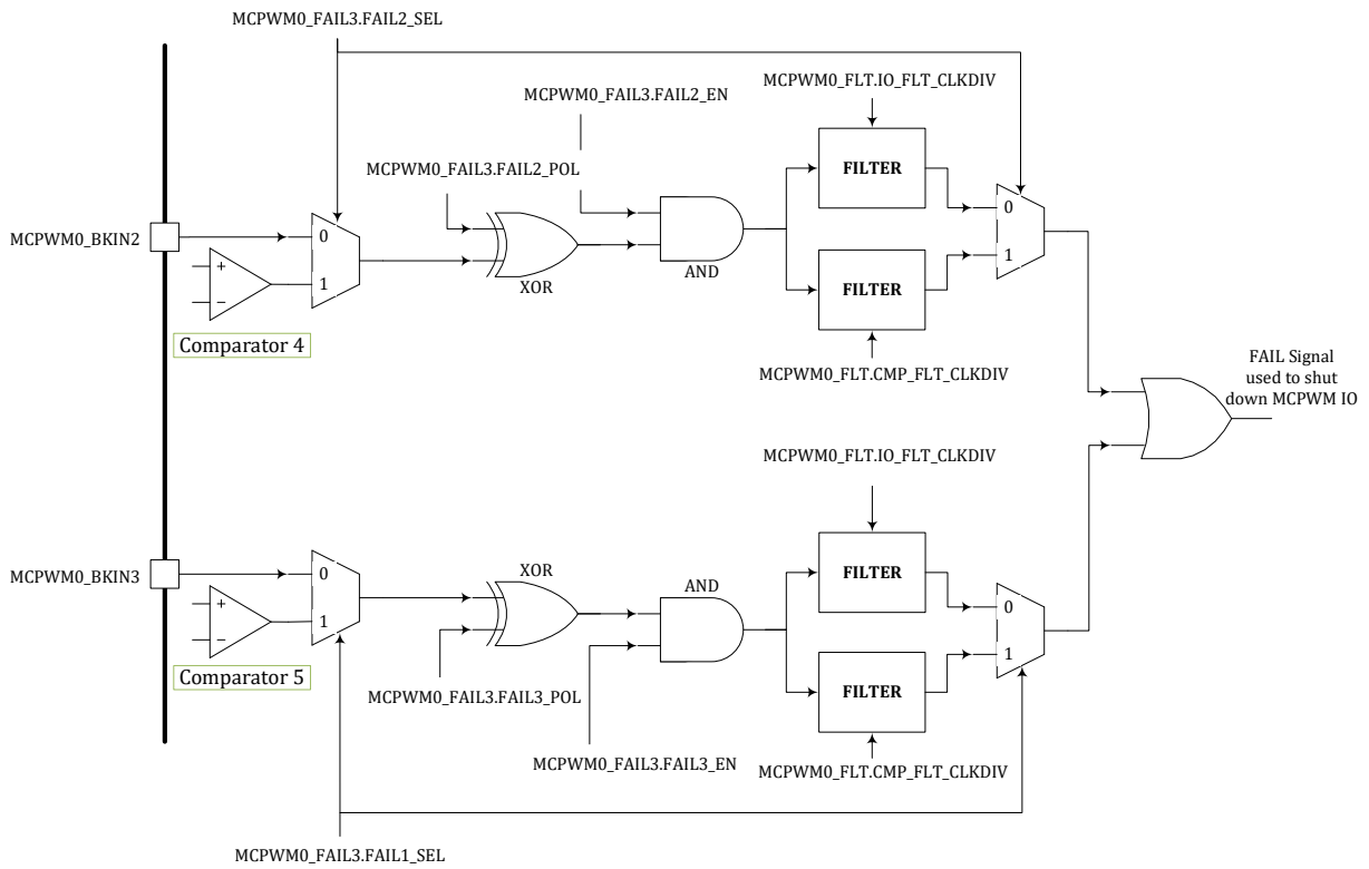
Figure 16-6 MCPWM0 FAIL2/3 Logic Diagram
