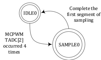
Figure 13-9 State Transition Diagram of ADC Single-round Sampling
