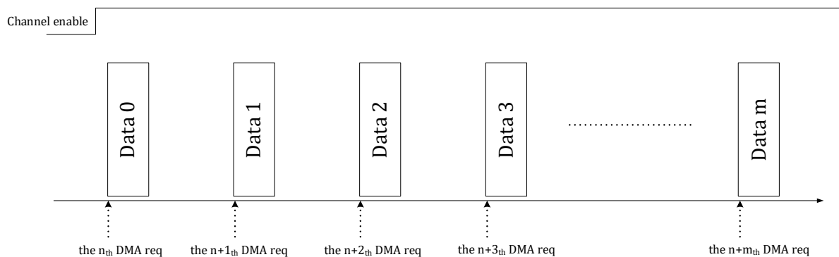
Figure 8-5 CIRC=1 and RMODE=1 DMA Transmission
