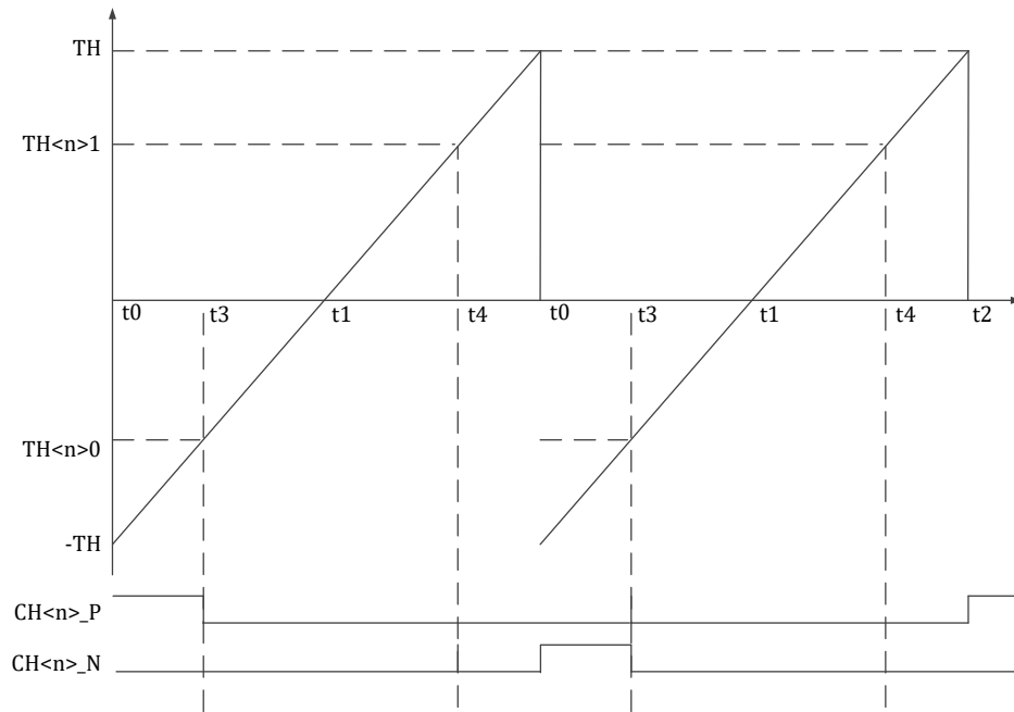
Figure 16-14 MCPWM Timing TH0 and TH1 Edge-aligned Push-pull Mode
