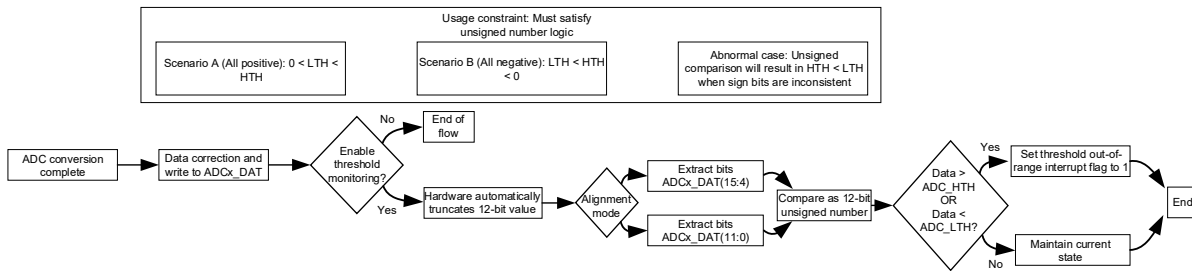
Figure 13-4 ADC Calibration and Processing Flowchart
