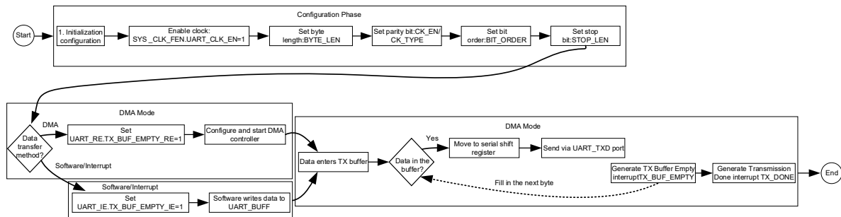
Figure17-1 UART Transmission Flow and Hardware Mechanisms
