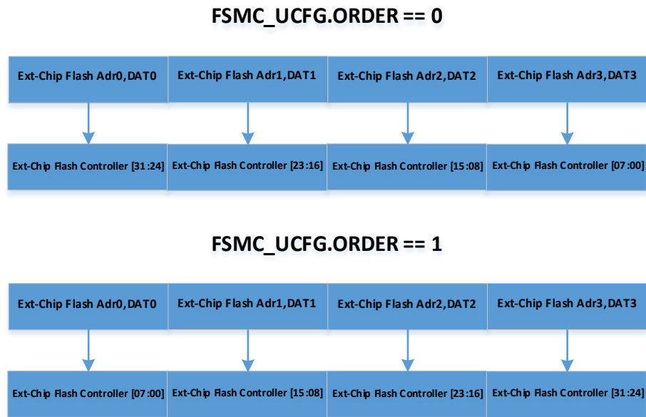
Figure 7-9 Data Read Sequence of Ext-Chip FLASH Indirect Access
