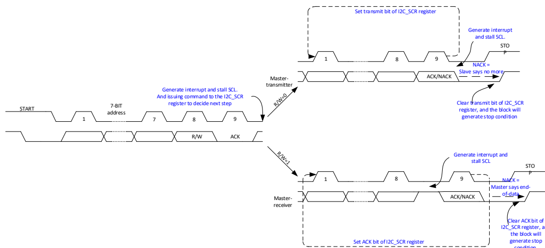
Figure 18-7 Schematic Diagram of Single-byte Transmission in Master Mode
