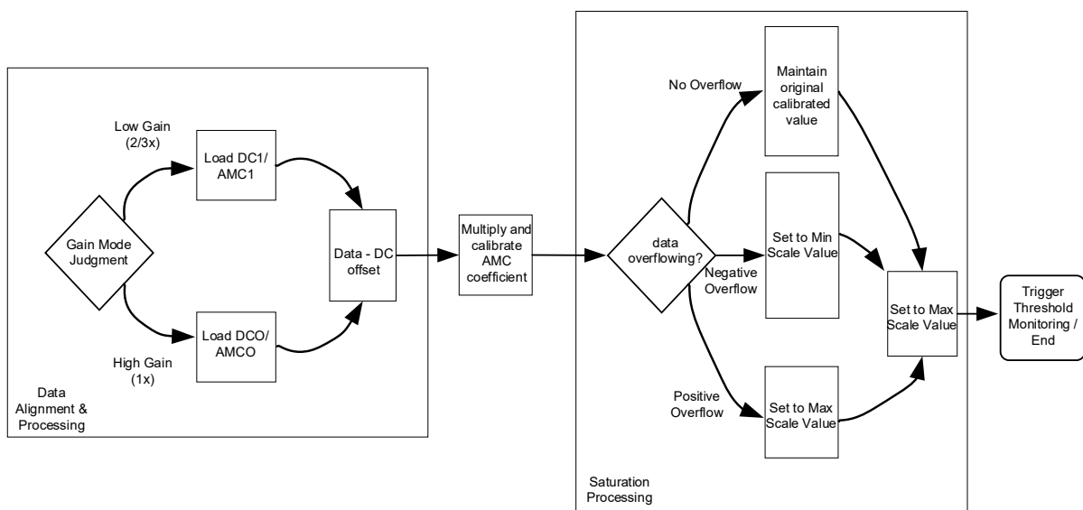
Figure 13-8 ADC Auto-Calibration Logic Flowchart
