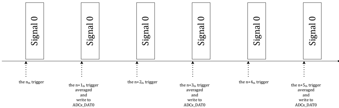
Figure 13-6 Oversampling Conversion Sequence Sample 2
