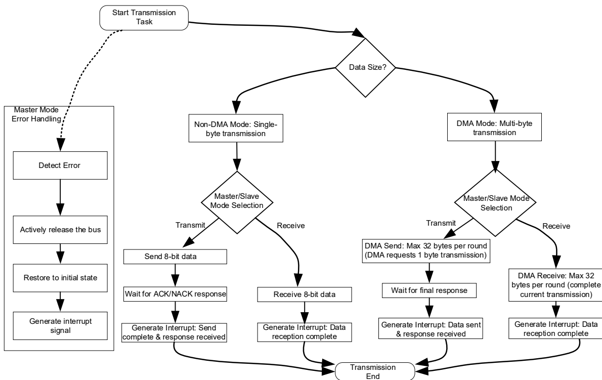
Figure 18-3 I2C Transmission Mode Decision and Execution Flowchart
