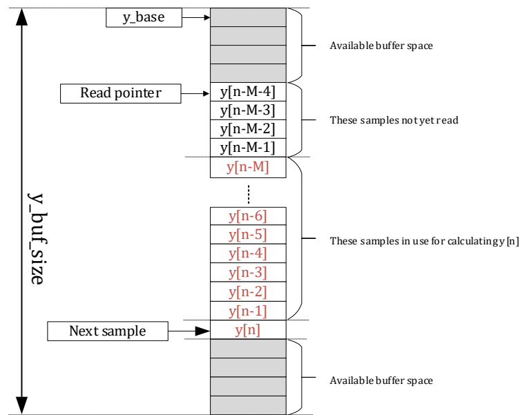
Figure 12-6 Circular output buffer
