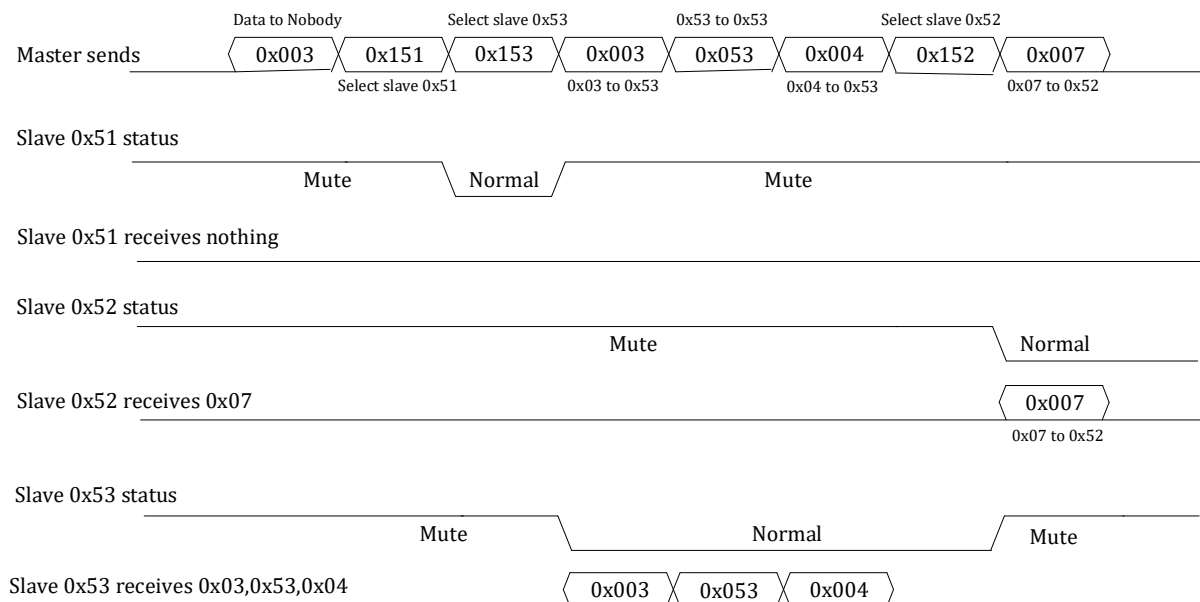
Figure 17-5 Example of UART Multi-computer Communication
