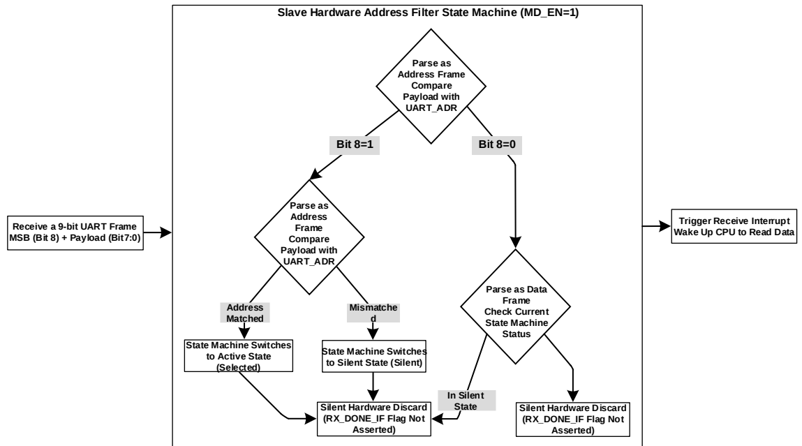
Figure 17-4 Processing Flow of Slave 9-bit UART Address Frame Filter State Machine
