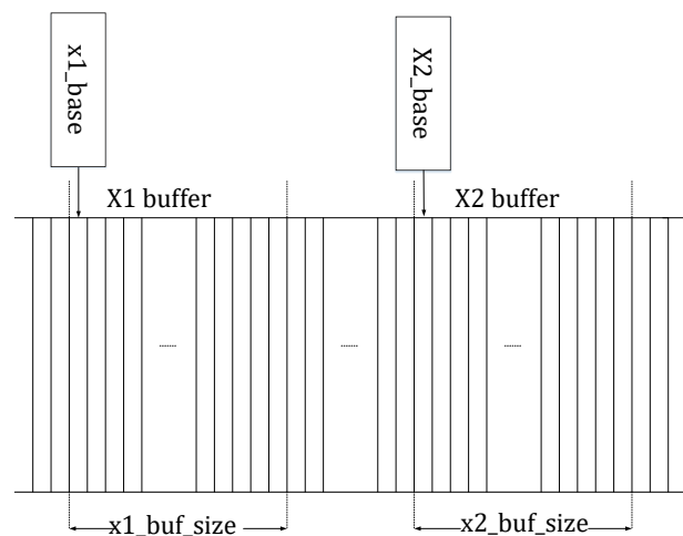
Figure 12-3 Input buffer areas
