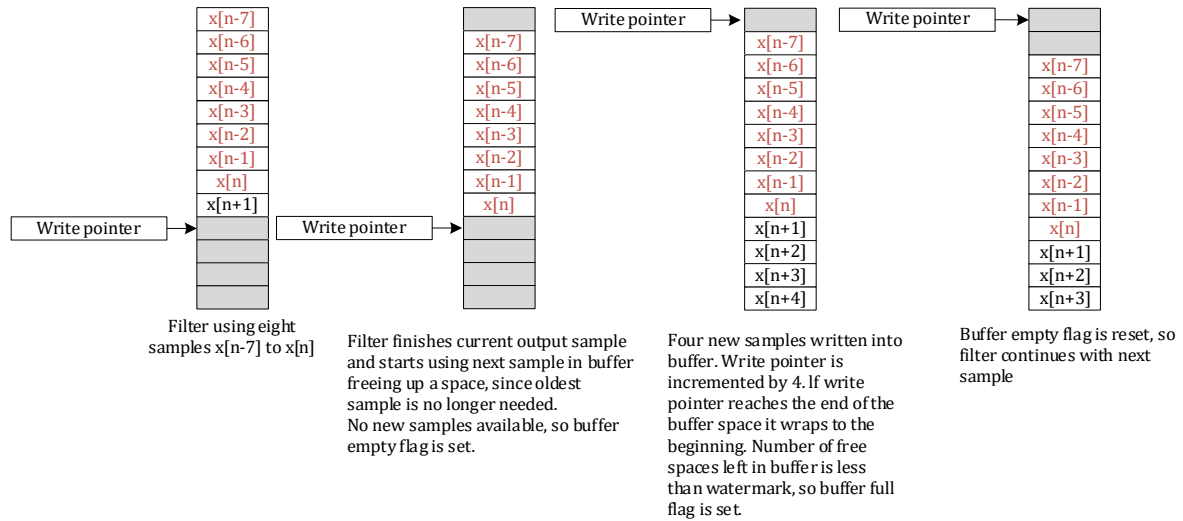
Figure 12-5 Circular input buffer operation
