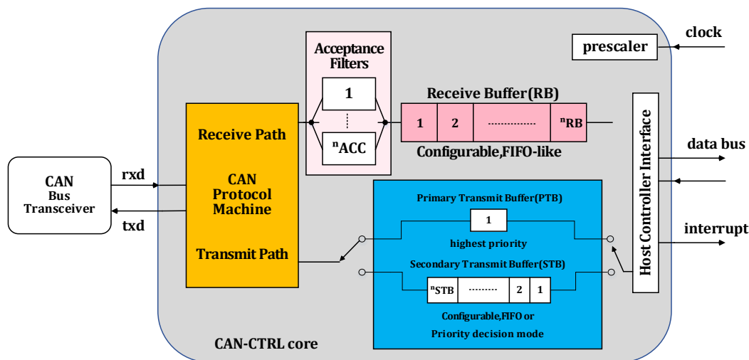
Figure 21-3 Message Buffers Concept
