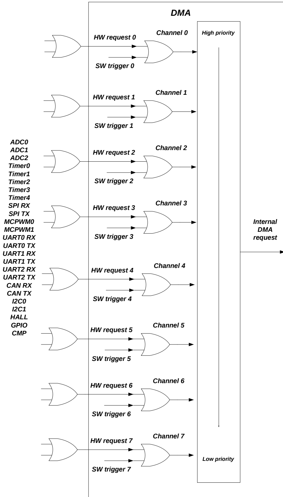
Figure 8-8 DMA Channel Priority
