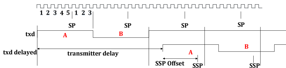
Figure 21-19 Transmitter Delay
