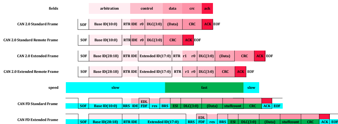
Figure 21-7 CAN 2.0 and CAN FD Frame Types
