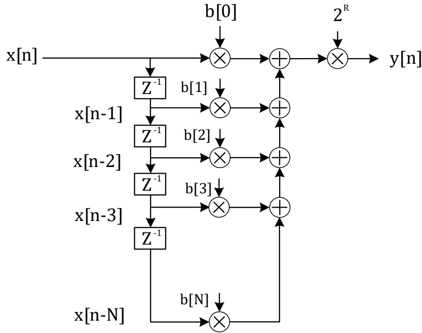
Figure 12-9 FIR filter structure
