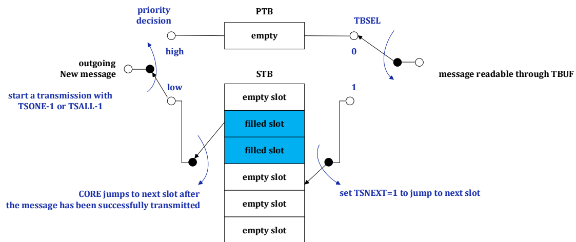
Figure 21-13 Schematic of PTB and STB in FIFO mode (empty PTB and 6 STB slots)
