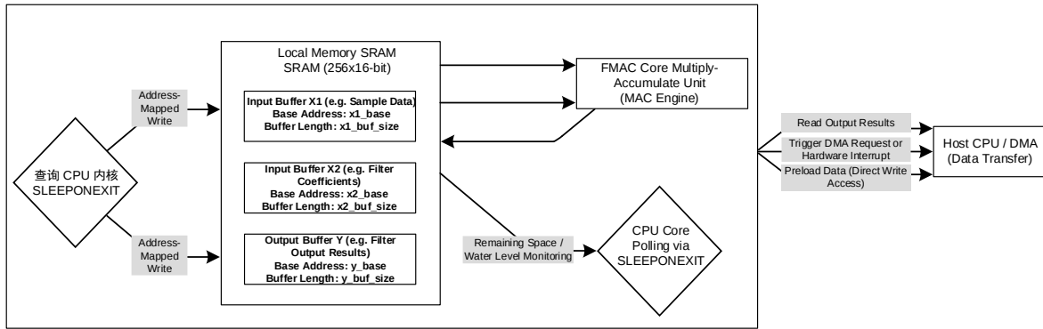
Figure 12-2 Overall Architecture of FMAC Hardware MAC Unit
