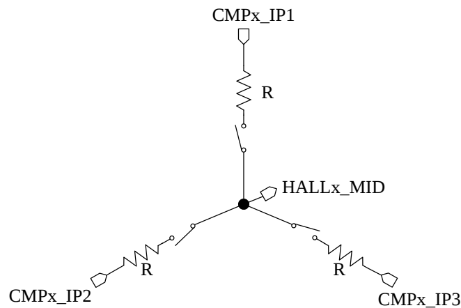
Figure 5-3 HALLx_MID signal
