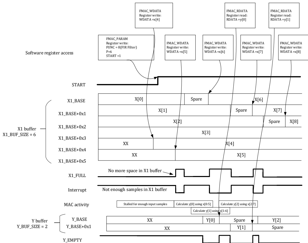
Figure 12-15 Filtering example 2
