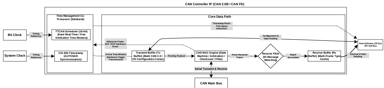
Figure 21-2 CAN Controller Data Path and Time Management Architecture
