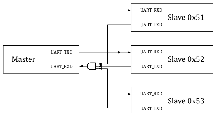
Figure 17-3 UART Multi-computer Communication Connection Topology
