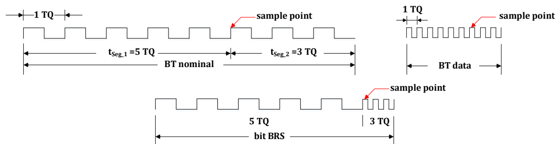
Figure 21-18 Bit Rate Switching at bit BRS S\_PRESC \neq F\_PRESC
