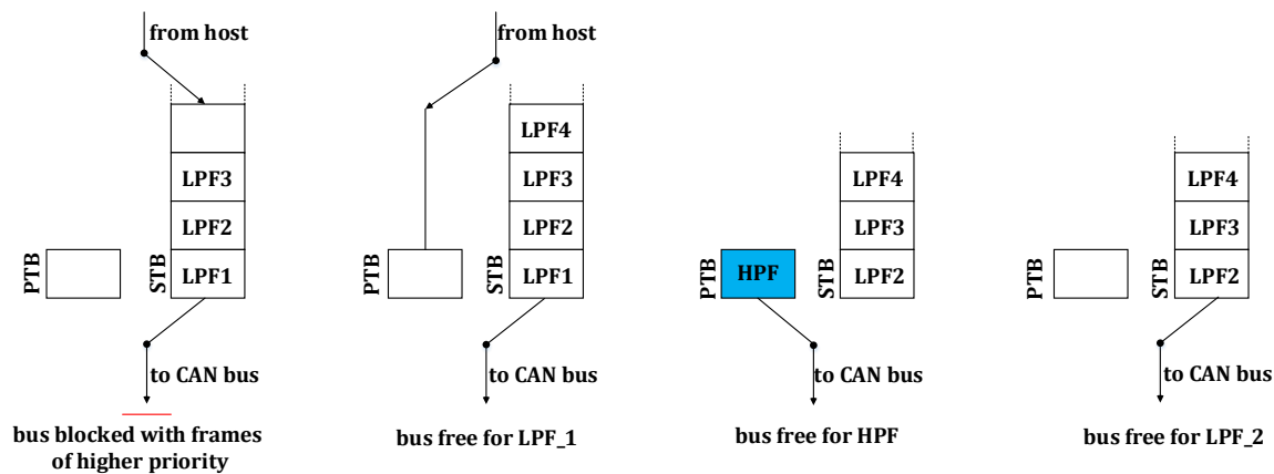
Figure 21-5 Transmit Buffer Application Example (TSALL=1)
