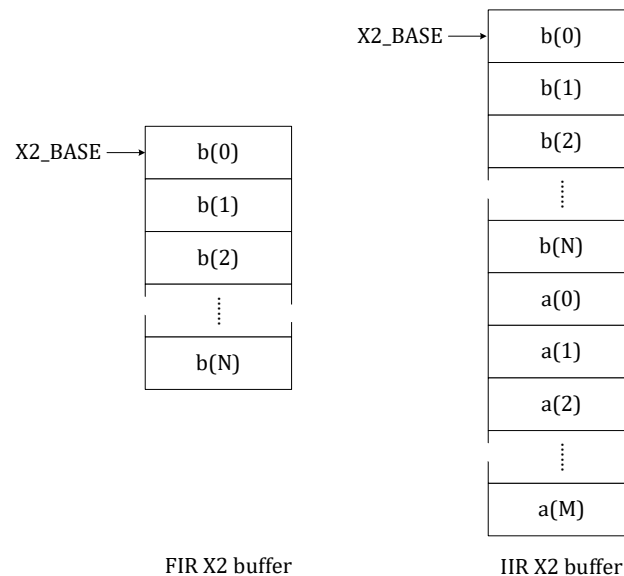
Figure 12-8 FIR and IIR filter x2 buffer coefficient
