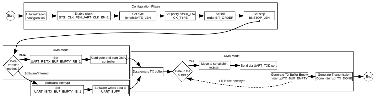
Figure17-1 UART Transmission Flow and Hardware Mechanisms
