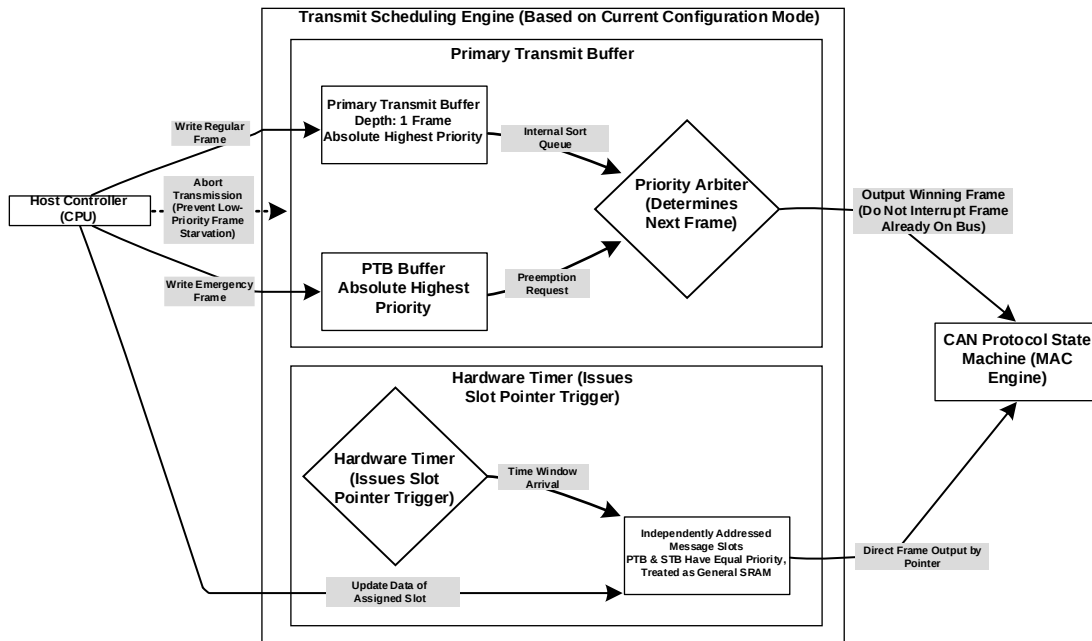
Figure 21-6 Conventional CAN Tx Events and TTCAN Time-Triggered Mechanism
