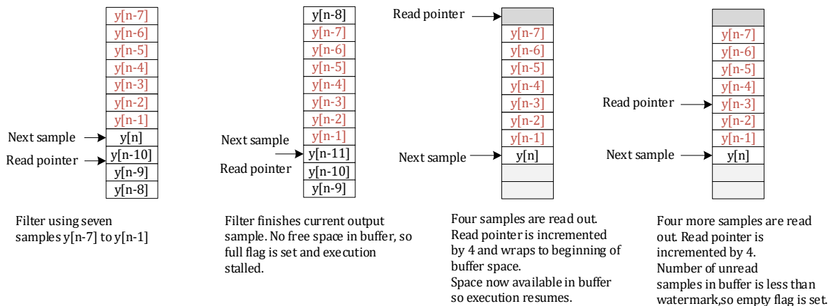
Figure 12-7 Circular output buffer operation
