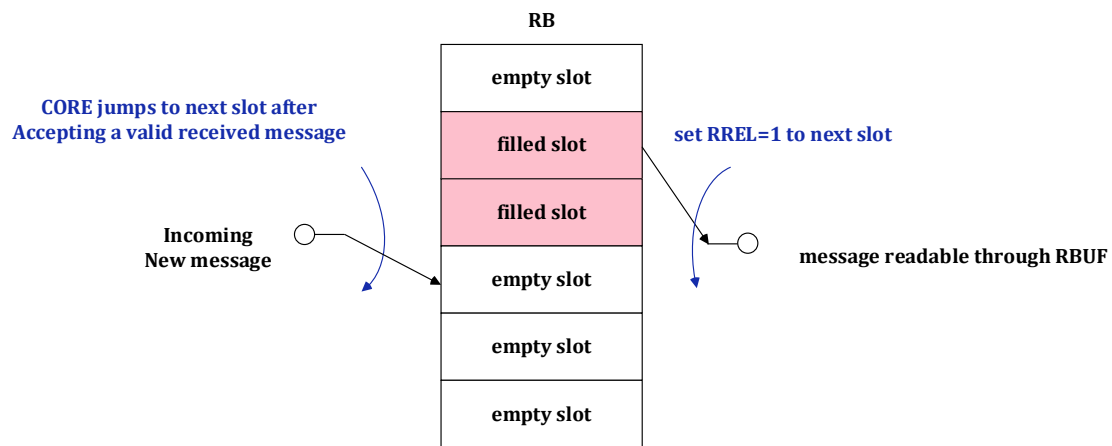
Figure 21-12 Schematic of the FIFO-like RB (example with 6 slots)
