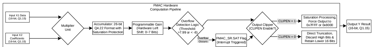
Figure 12-11 FMAC Hardware MAC Kernel Pipeline
