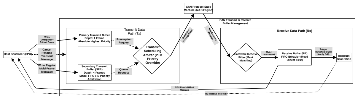
Figure 21-4 CAN Controller Data Path Architecture Diagram
