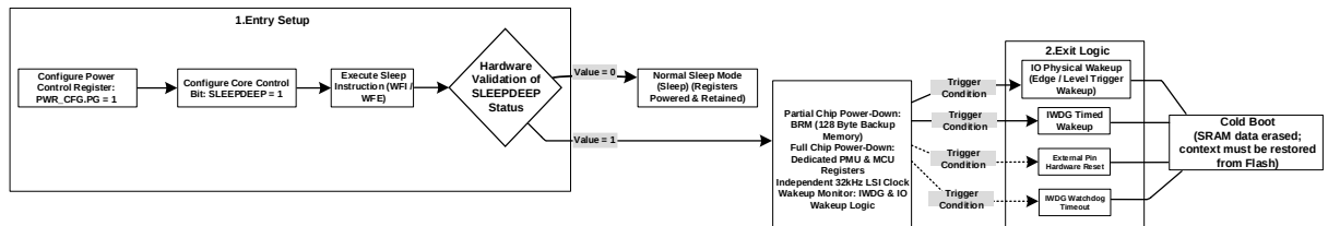
Figure 21-3 Stop/Standby Entry & Cold Boot Exit Flowchart
