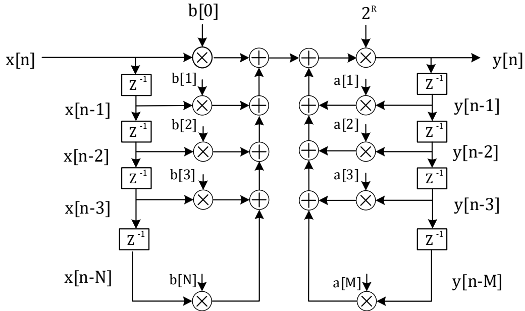
Figure 12-10 IIR filter structure (direct form 1)
