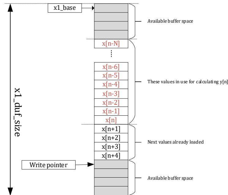
Figure 12-4 Circular input buffer
