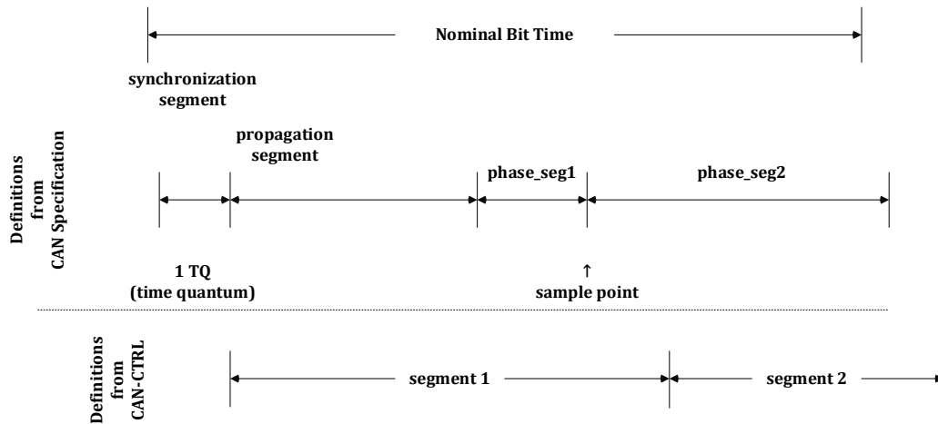
Figure 21-16 CAN Bit Timing Specifications
