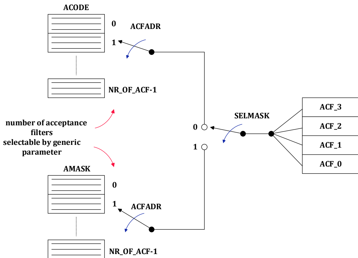
Figure 21-8 Access to the Acceptance Filters
