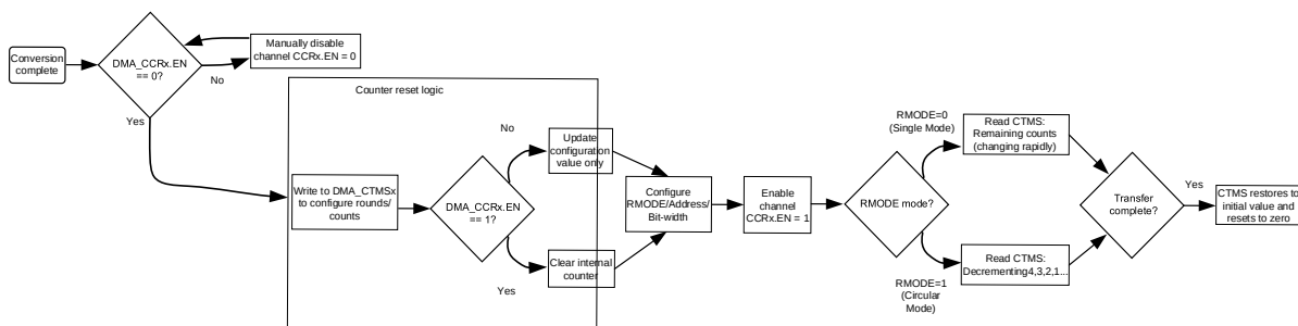
Figure 8-9 DMA Operation Logic Flowchart
