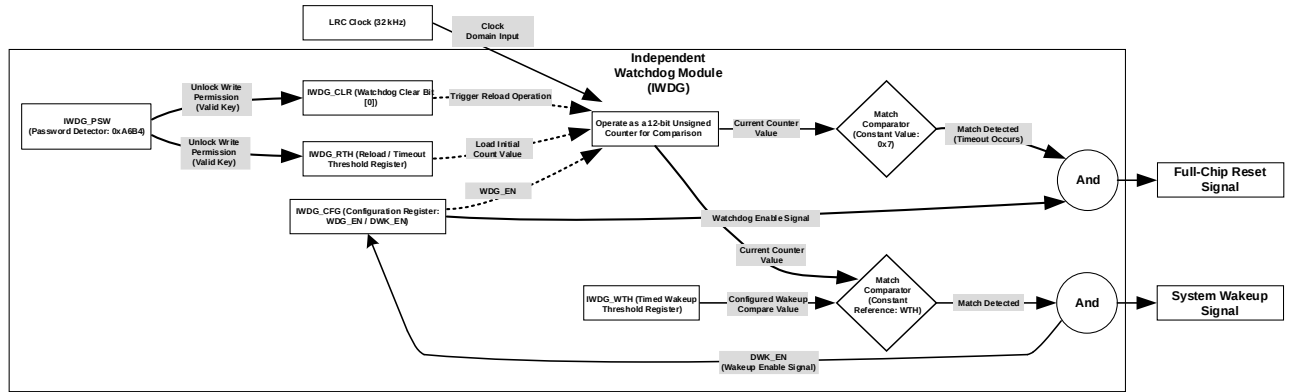
Figure 23-1 IWDG Operating Principle & Signal Flow
