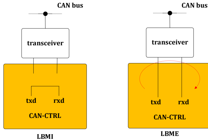
Figure 21-14 Loop Back Mode: Internal and External
