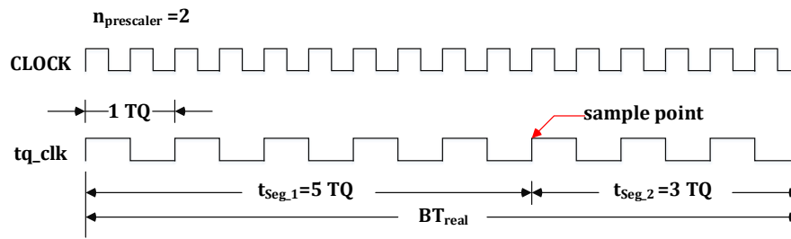
Figure 21-17 Clock Division for Bit Sampling
