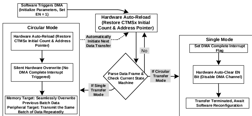
Figure 8-7 Flowchart of DMA Transmission in Single Mode and Circular Mode
