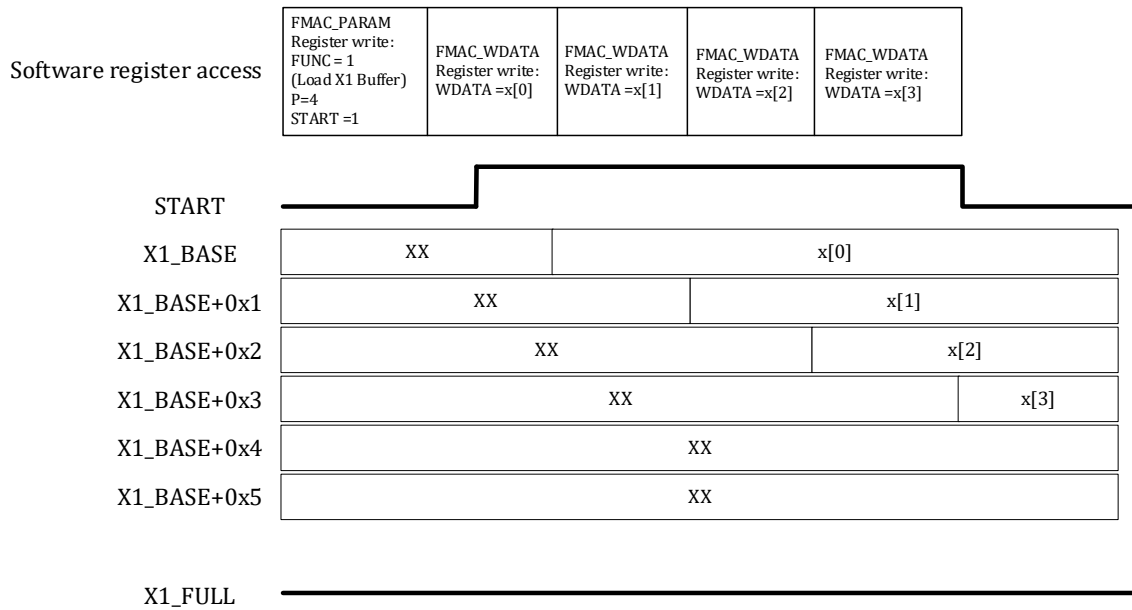
Figure 12-13 X1 buffer initialization
