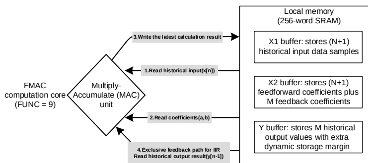
Figure 12-12 IIR Filter Data Interaction Architecture of FMAC (FUNC=9)
