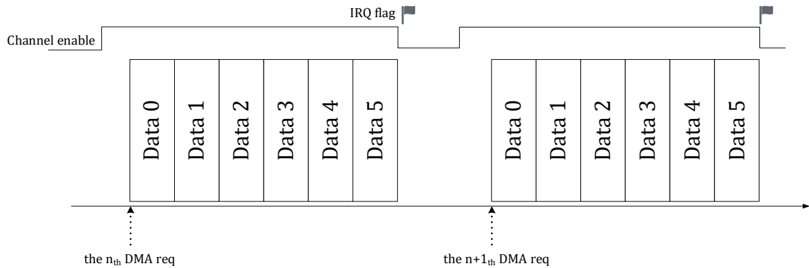
Figure 8-6 CIRC=1 and RMODE=0 DMA Transmission
