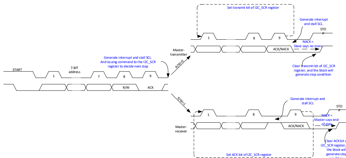
Figure 18-10 Schematic Diagram of Single-byte Transmission in Master Mode
