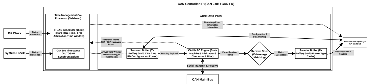
Figure 21-2 CAN Controller Data Path and Time Management Architecture
