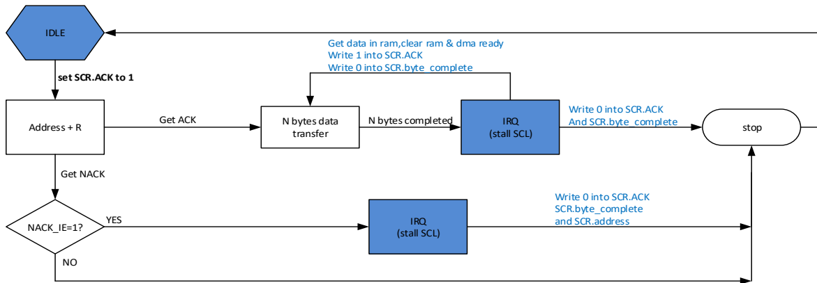
Figure 18-13 Schematic Diagram of Multi-byte Reception in Master Mode
