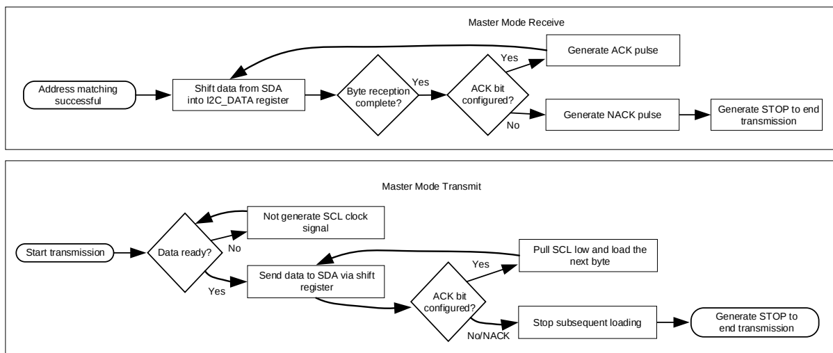
Figure 18-11 Logic Flow Chart for I2C Master Mode Transmission and Reception
