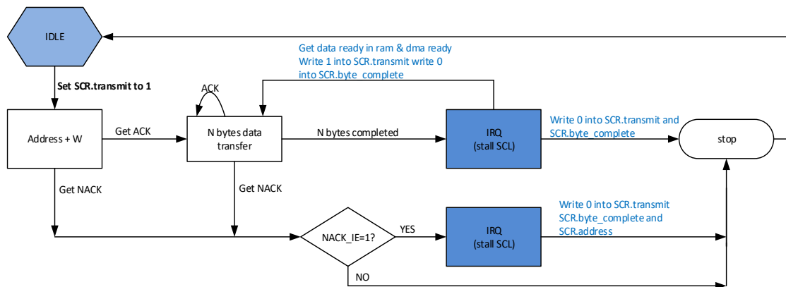
Figure 18-12 Schematic Diagram of Multi-byte Transmission in Master Mode
