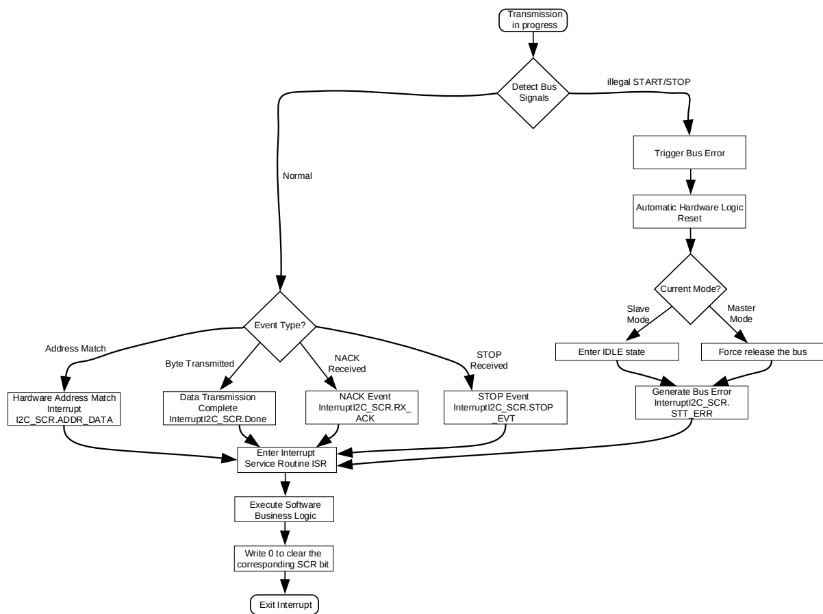
Figure 18-15 Logic Flow Chart for I2C Bus Error Handling and Interrupt Management
