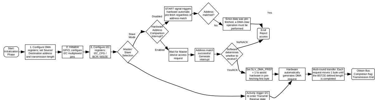
Figure 18-14 Logic Flow Chart for DMA Configuration and Execution of I2C Interface in High-Volume Data Transmission
