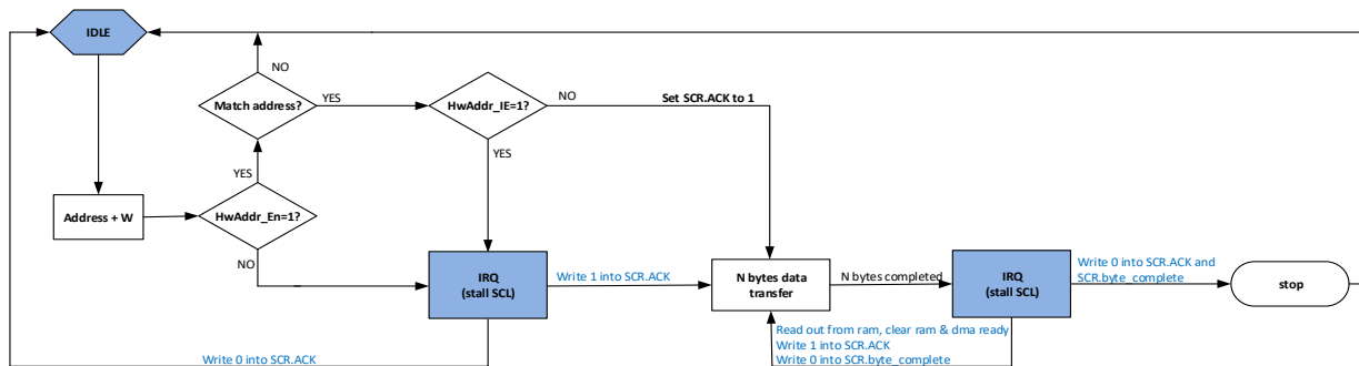
Figure 18-9 Schematic Diagram of Multi-byte Reception in Slave Mode
