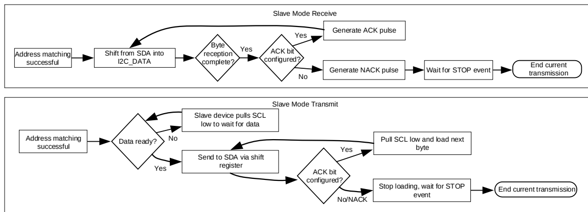
Figure 18-7 I2C Slave Mode (Transmit/Receive/DMA) Logic Flowchart
