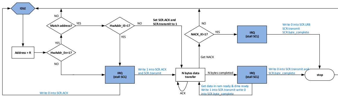
Figure 18-8 Schematic Diagram of Multi-byte Transmission in Slave Mode
