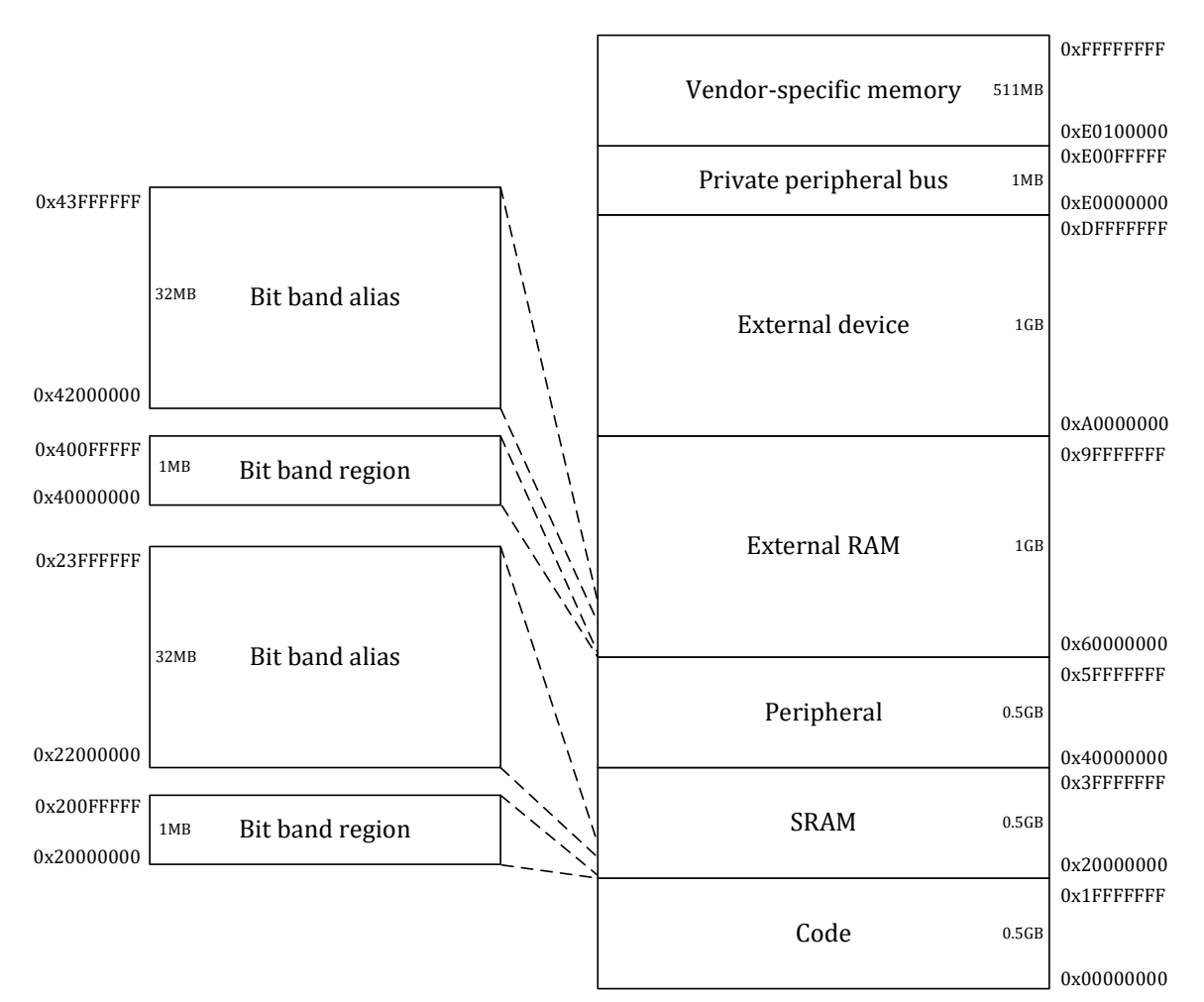
图 3-1 RISC CPU Memory Model
